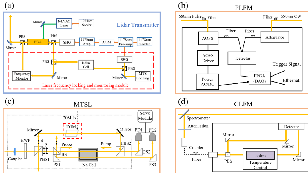
Figure 3. Schematic diagram of (a) the lidar transmitter, (b) pulsed laser frequency monitoring (PLFM) unit, (c) modulation transfer spectroscopy locking (MTSL) unit, (d) continuous laser frequency monitoring (CLFM) unit of the lidar system.
