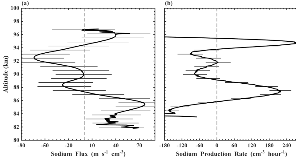
Figure 13. The dynamical flux of sodium. (a) Na flux due to dissipating gravity waves calculated from the measured Na density and vertical wind measurements at Hainan. (b) Na production rate calculated from measured Na flux at Hainan. Error bars are shown as thin lines.
