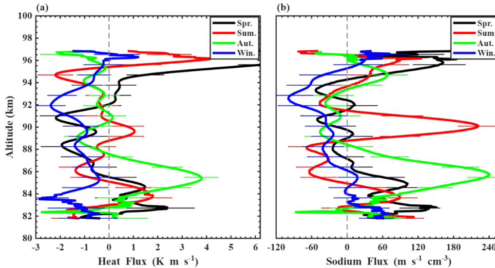
Figure 14. The seasonal profiles of the heat (a) and Na (b) fluxes. Spring (black), summer (red), autumn (green), winter (blue). Error bars are shown as thin lines.
