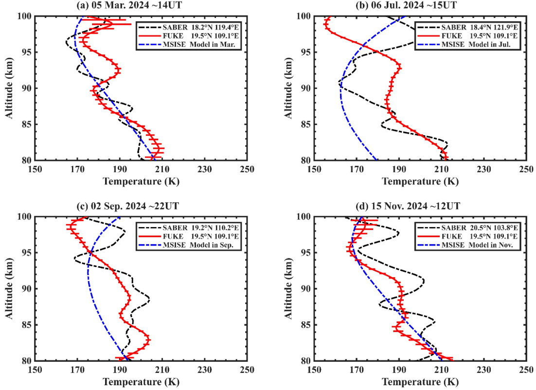
Figure 7. Typical profiles of temperature measured by lidar (red solid line), SABER (black dashed line) and 185 MSISE (blue dashed line) in different seasons. (a) spring, (b) summer, (c) autumn, (d) winter. Error bars are shown as thin lines.
