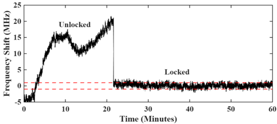
Figure 4. Continuous laser frequency monitoring results.
