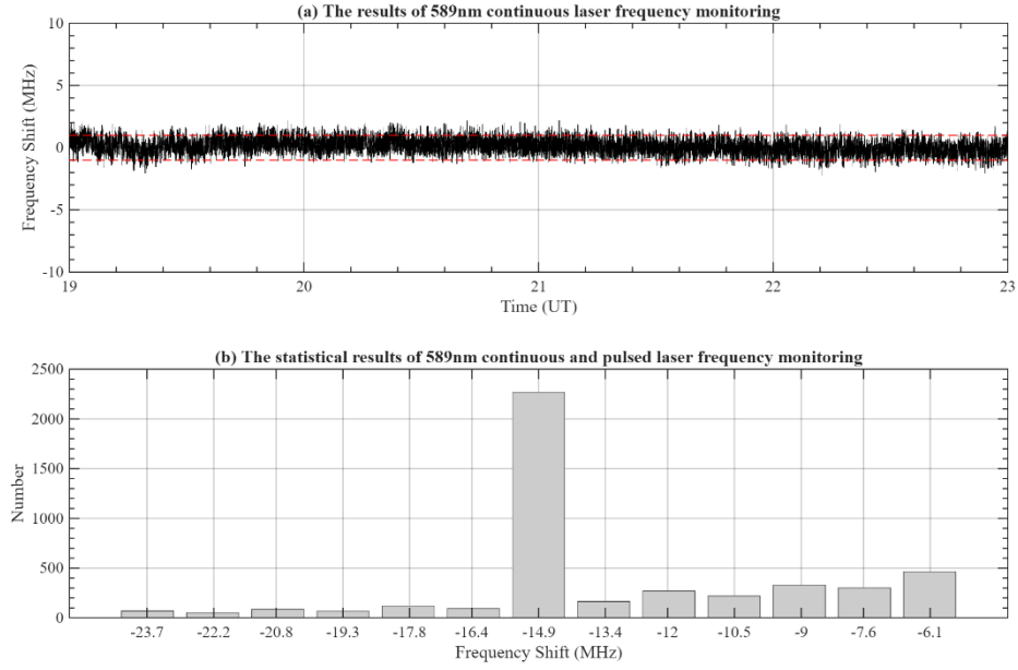
Figure 5. Results of the laser frequency locking and monitoring module on 7 July 2024. (a) the results from continuous laser frequency monitoring unit; (b) the statistical results from continuous and pulsed laser frequency monitoring unit.
