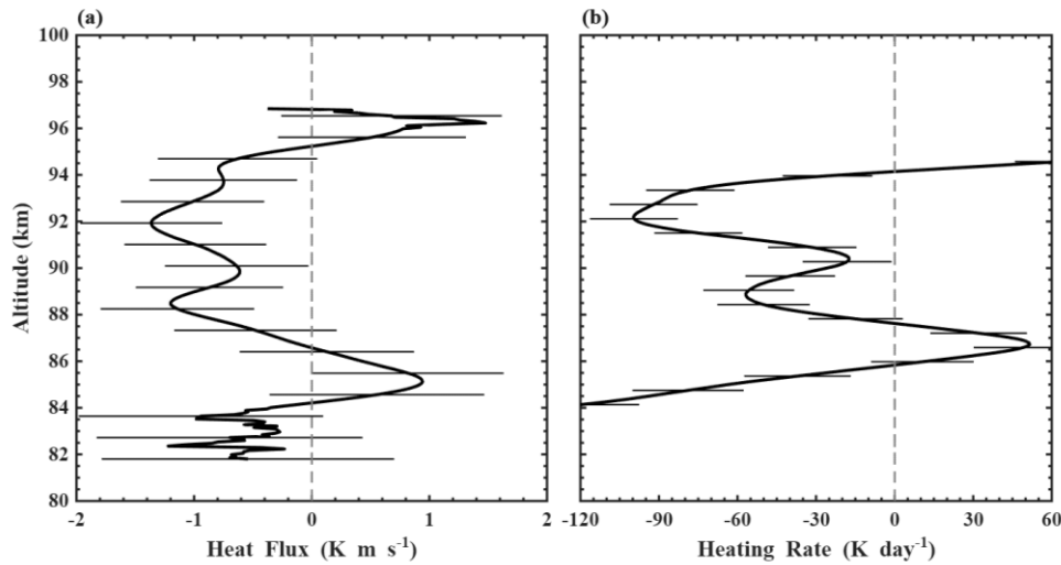
Figure 12. The vertical flux of sensible heat. (a) Annual mean sensible heat flux derived from vertical wind and temperature measurements at Hainan, China, and (b) the corresponding heating rates. Error bars are shown as thin lines.
