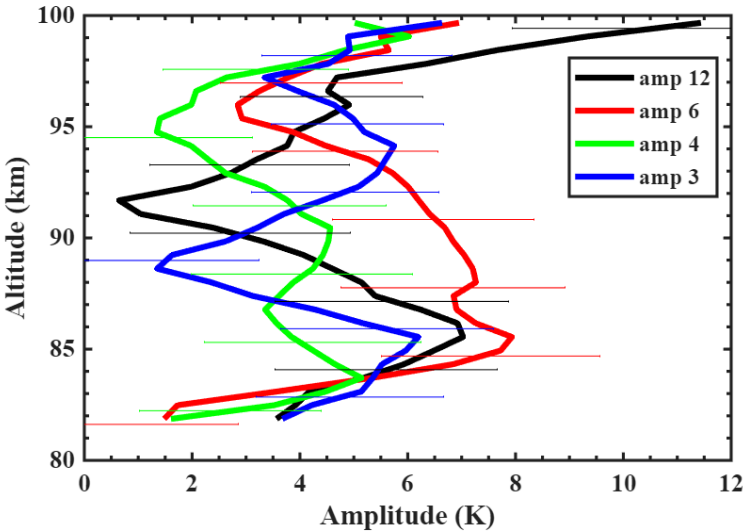
Figure 11. Seasonal harmonic amplitude profiles with the period of 12 (black), 6 (red), 4 (green), and 3 (blue) months. Error bars are shown as thin lines.
