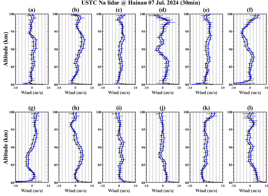
Figure 6. Sodium layer vertical wind (black dashed line) and the vertical wind after correcting frequency offset (blue solid line) at 30 minutes on 7 July 2024. Error bars are shown as thin lines.
