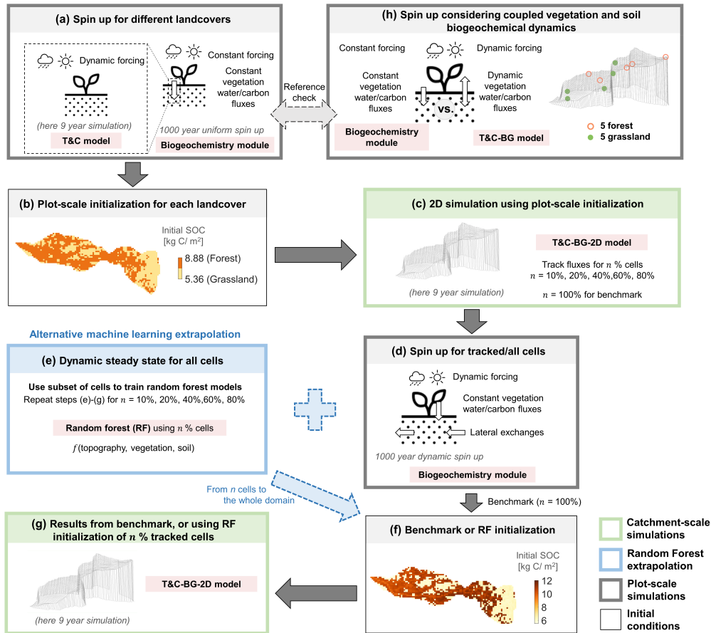
Figure 2. Workflow of the model initialization procedure. (a) For each soil–vegetation combination, the Deleted: perform T&C model is used to obtain Deleted: to get averaged water and plant fluxes, which are used in a 1D spin-up via the T&C-BG biogeochemistry module using long-term average meteorological inputs. The resulting steady-state pools are then assigned to all cells with the same soil–vegetation combination (b). (c) A 2D simulation (T&C-BG-2D) is run with these initial conditions, tracking fluxes all cells (benchmark) or for a given percentage n of all grid cells. (d) For these cells, the T&C-BG biogeochemistry module 1D spin-up with dynamic meteorology and imposed lateral fluxes is run to achieve a dynamic steady state in all tracked cells. (e) A random forest (RF) model is trained on results from different percentages ( n ) of the subset of these cells Deleted: ( n ) using topographic, soil, and vegetation attributes as predictors to reconstruct the initial conditions for the entire catchment domain (f), which are then used to initialize the final simulations (g). For each simulation scenario, steps (e) to (g) are repeated for different percentages of tracked cells n to investigate the optimal number of cells for the RF algorithm. (h) Additional plot-scale simulations are performed for 10 representative cells (5 forest, 5 grassland) to obtain a reference steady state using the fully coupled T&C-BG model (i.e., also considering dynamic vegetation fluxes), which is compared to the initial states generated in step (a). The solid arrows represent steps needed for the benchmark simulation, the dashed arrows represent the alternative machine learning extrapolation (blue) and the reference check (gray). See Table 1 for details on models used in the spin-up procedure and their acronyms.
