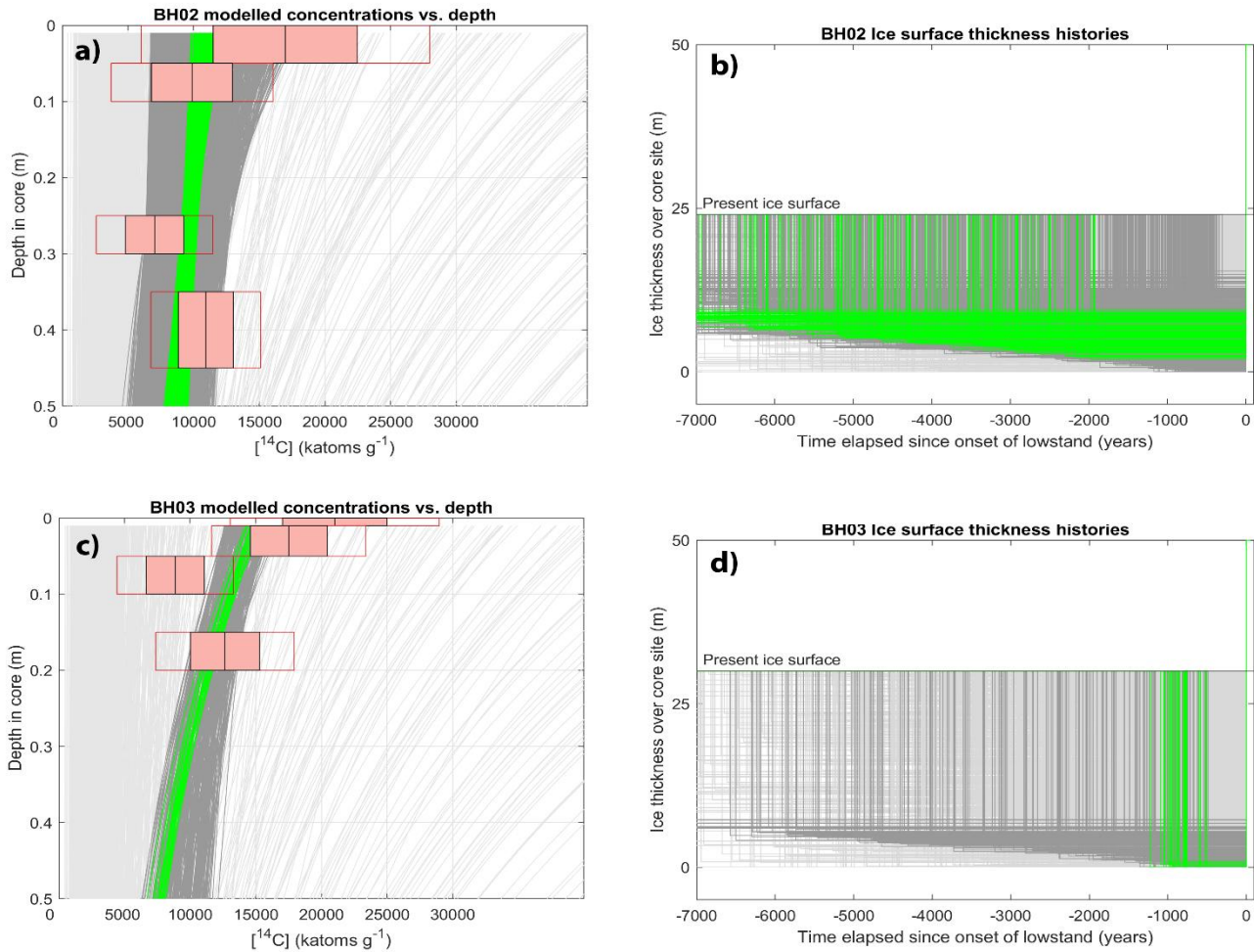
345 Figure. 8. a) Predicted nuclide concentrations plotted against depth in core BH02. Measured concentrations shown as in Fig. 7. Concentrations predicted by the best (10 th percentile) of fitting iterations shown in green, top 5% of all fitting iterations shown in dark grey, random selection (n = 1000) of all remaining iterations shown in light grey. b) Three stage ice histories used to produce modelled concentrations, colours correspond to the same sub-sets of iterations as panel (a). The histories, which all have different starting times in the model, have been aligned to the onset of the low stand for visualisation. c) and d) are the same figures but for BH03. 350
