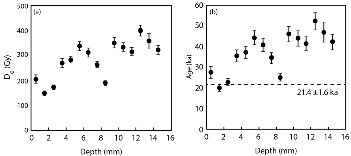
240 Figure 5. Luminescence depth plots for sample BH01 showing D_e values (a) and apparent burial ages (b) measured using the OSL signal of quartz. Note that only Discs 2 and 3 (depths 1.5 and 2.5 mm, respectively) were used for age calculation.
