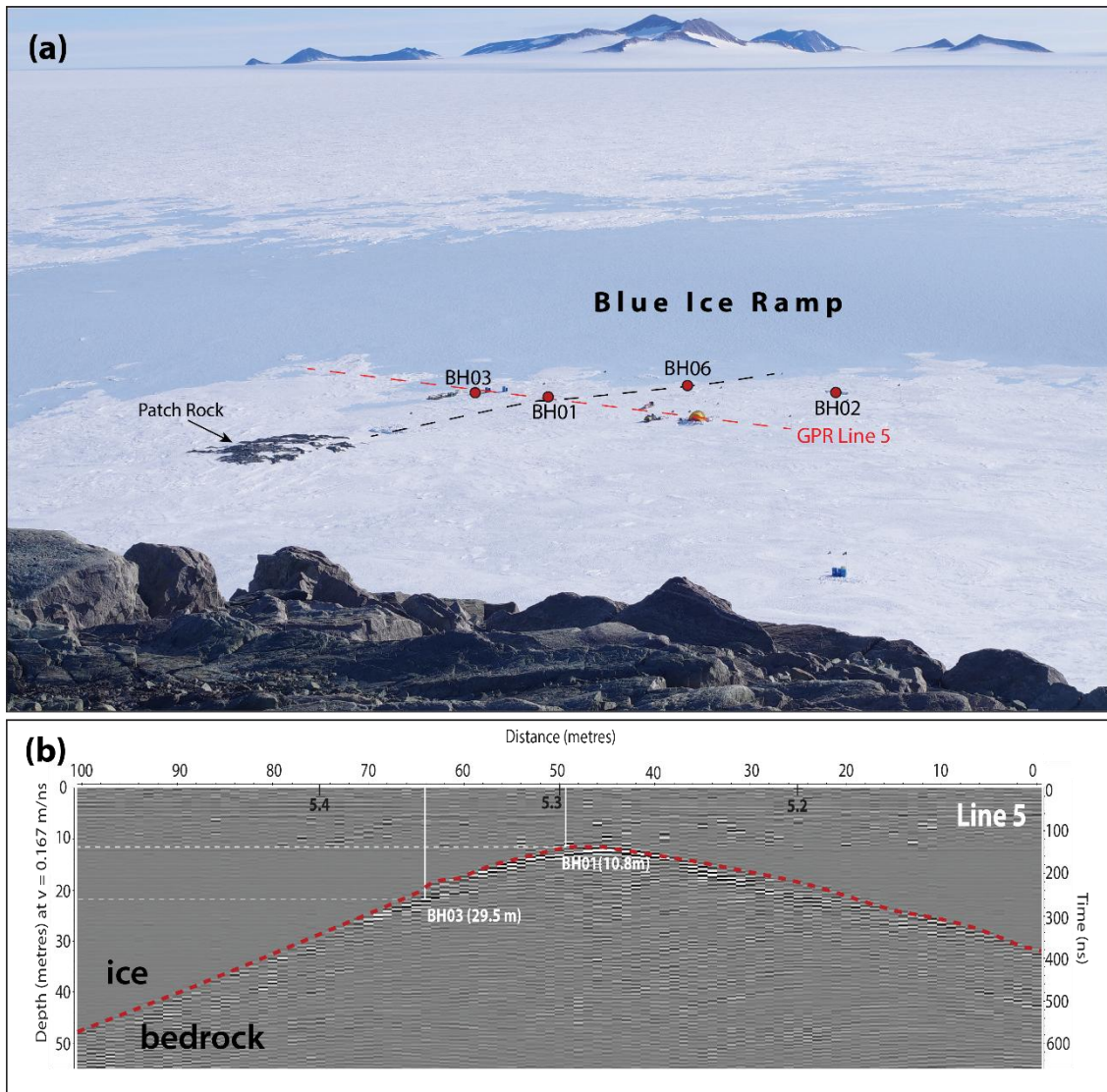
145 Figure 3. A) Patch Rock viewed from the top of Plummer Nunatak. The locations of the bedrock cores are shown. The black dashed line denotes the approximate trace of the subglacial ridge as surveyed before it passes underneath the blue ice ramp. Vertical relief of the ramp is c.10 m. GPR Line 5 is shown as a red dashed line in A). B) Interpreted radargram of GPR Line 5 showing locations of cores BH01 and BH03 along with measured depths to bedrock (n.b. for BH03 this is greater than depth extrapolated from two-way-travel time). The numbers 5.2 etc denote locations of flags used as fiducial markers. GPR Lines 1-4 were located at 10 m intervals in increasing proximity to Patch Rock (see supplemental).
