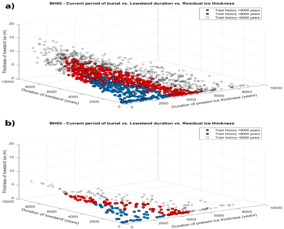
385 Figure 10. XYZ plot of durations of low stand (Stage 2) and period of present ice thickness (Stage 3) against residual ice thickness during Stage 2 for cores BH02 (a) and BH03 (b). Nearest exposure age data imply ice surface reached modern elevations at c. 6-4 ka thus total duration of Stage 2 and Stage 3 would be shorter than this. Such constraints narrow the range of possible low stand durations and residual ice thicknesses as shown for periods of 4000 years (blue markers) and 6000 years (red markers). Remaining accepted scenarios shown with white markers.
