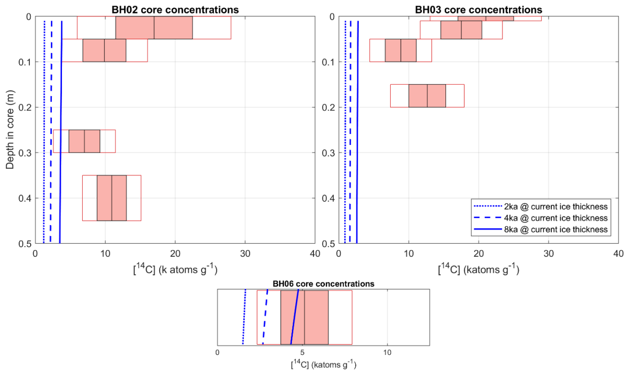
Figure 7. Downcore measured nuclide concentrations for and predicted depth profiles under invariant ice cover for durations of 2 ka, 4 ka, and 8 ka for samples from BH02 (a), BH03 (b) and the single sample from BH06 (c). Solid box and outline denote 68% and 95% uncertainties on measured nuclide concentrations respectively.
