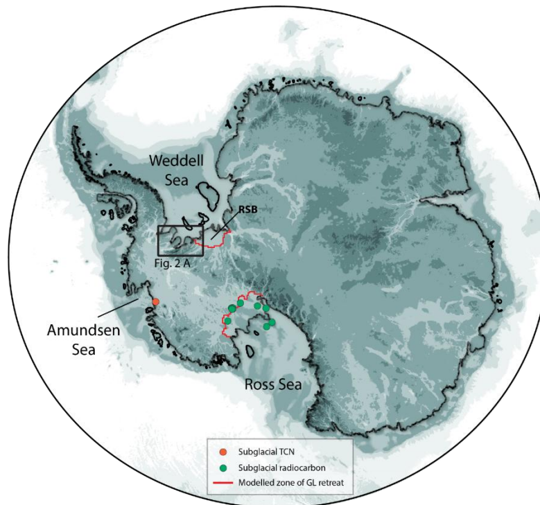
45 Figure 1. Overview map of Antarctica showing locations where geological evidence of Holocene retreat inboard of the present day grounding line has been recovered. Modelled zones of retreat in the Ross and Weddell Sea embayments are taken from Kingslake et al. (2018), other models show similar patterns. Black box shows location of Fig. 2a. RSB: Robin subglacial basin. Base image is BEDMAP3 subglacial topography (Pritchard et al., 2025).
