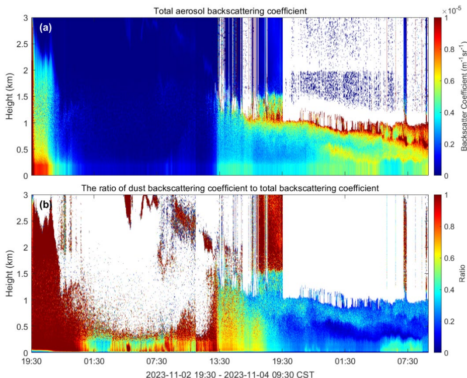
Figure 2: (a) the spatial-temporal evolution of the total aerosol backscattering coefficient at 532 nm wavelength from 19:30 on November 2, 2023, to 09:30 on November 4 (CST). (b) the ratio of dust backscattering coefficient to total backscattering coefficient. The white areas indicate the absence information.
