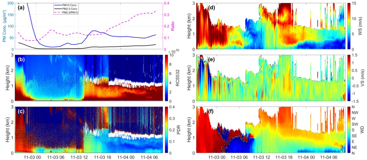
Figure 1: In-situ and lidar observation results over Beijing from 19:30 on November 2, 2023, to 09:30 on November 4, 2023 (CST). (a) Near-surface PM 2.5 and PM 10 concentrations and their ratio from 19:30 on November 2, 2023, to 09:30 on November 4, 2023; (b) Observational results of the temporal and spatial distribution of the REAL and wind profiler lidar from 19:30 on November 2, 2023, to 09:30 on November 4, 2023, in the 0-3 km atmospheric layer over Beijing (b) 532 nm lidar range-corrected signal (RCS, representing vertical distribution information of relative aerosol loadings); (c) 532 nm particle depolarization ratio; (d) Temporal
