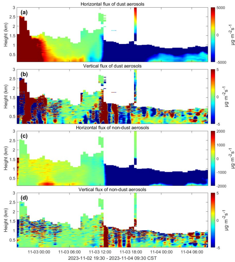
Figure 5: Aerosol flux results from 19:30 on November 2, 2023, to 09:30 on November 4, 2023 (China Standard Time, CST), in the 0.1-3 km atmospheric layer over Beijing. (a) Horizontal flux of dust aerosols; (b) Vertical flux of dust aerosols; (c) Horizontal flux of non-dust aerosols; (d) Vertical flux of non-dust aerosols.
