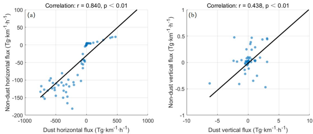
495 Figure 8: Correlation between Dust and Non-Dust Aerosol Fluxes. (a) Scatter plot showing the correlation between dust horizontal flux and non-dust horizontal flux. (b) Scatter plot illustrating the correlation between dust vertical flux and non-dust vertical flux.
