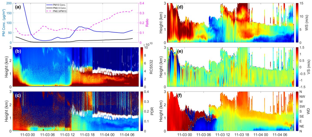
Figure 1: In-situ and lidar observation results over Beijing from 19:30 on November 2, 2023, to 09:30 on November 4, 2023 (CST). (a) Near-surface \text{PM}_{2.5} and \text{PM}_{10} concentrations and their ratio from 19:30 on November 2, 2023, to 09:30 on November 4, 2023; (b) Observational results of the temporal and spatial distribution of the REAL and wind profiler lidar from 19:30 on November 2, 2023, to 09:30 on November 4, 2023, in the 0-3 km atmospheric layer over Beijing (b) 532 nm lidar range-corrected signal (RCS, representing vertical distribution information of relative aerosol loadings); (c) 532 nm particle depolarization ratio; (d) Temporal
