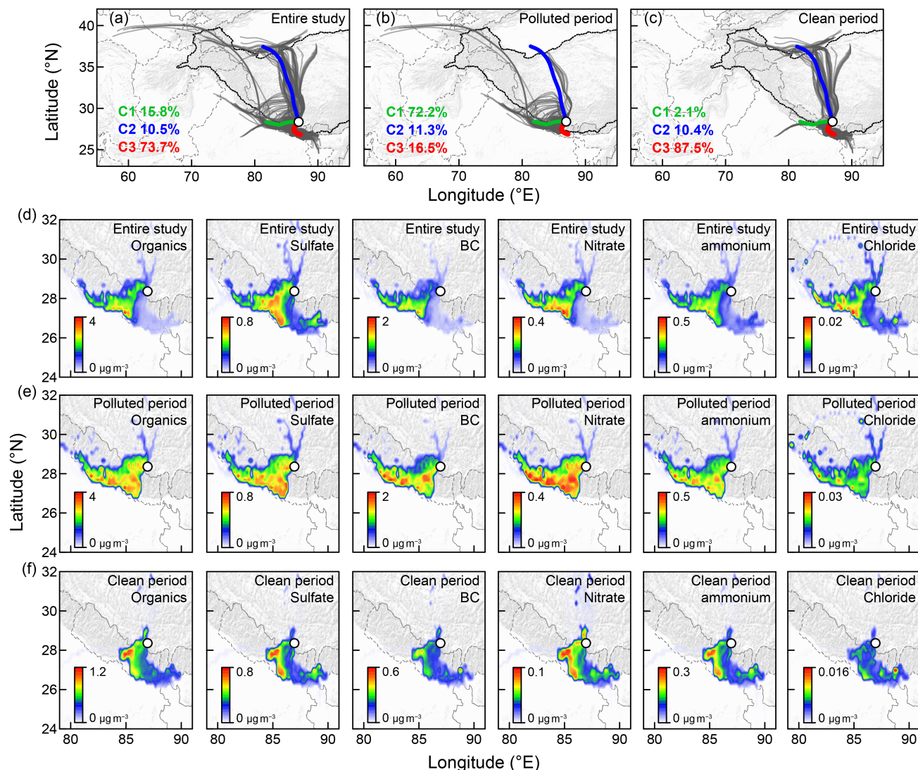
Figure 4. The 3-day backward air mass trajectories, trajectory clusters and CWT of PM_{10} species for the (a, d) entire study period, (b, e) polluted period and (c, f) clean period.
