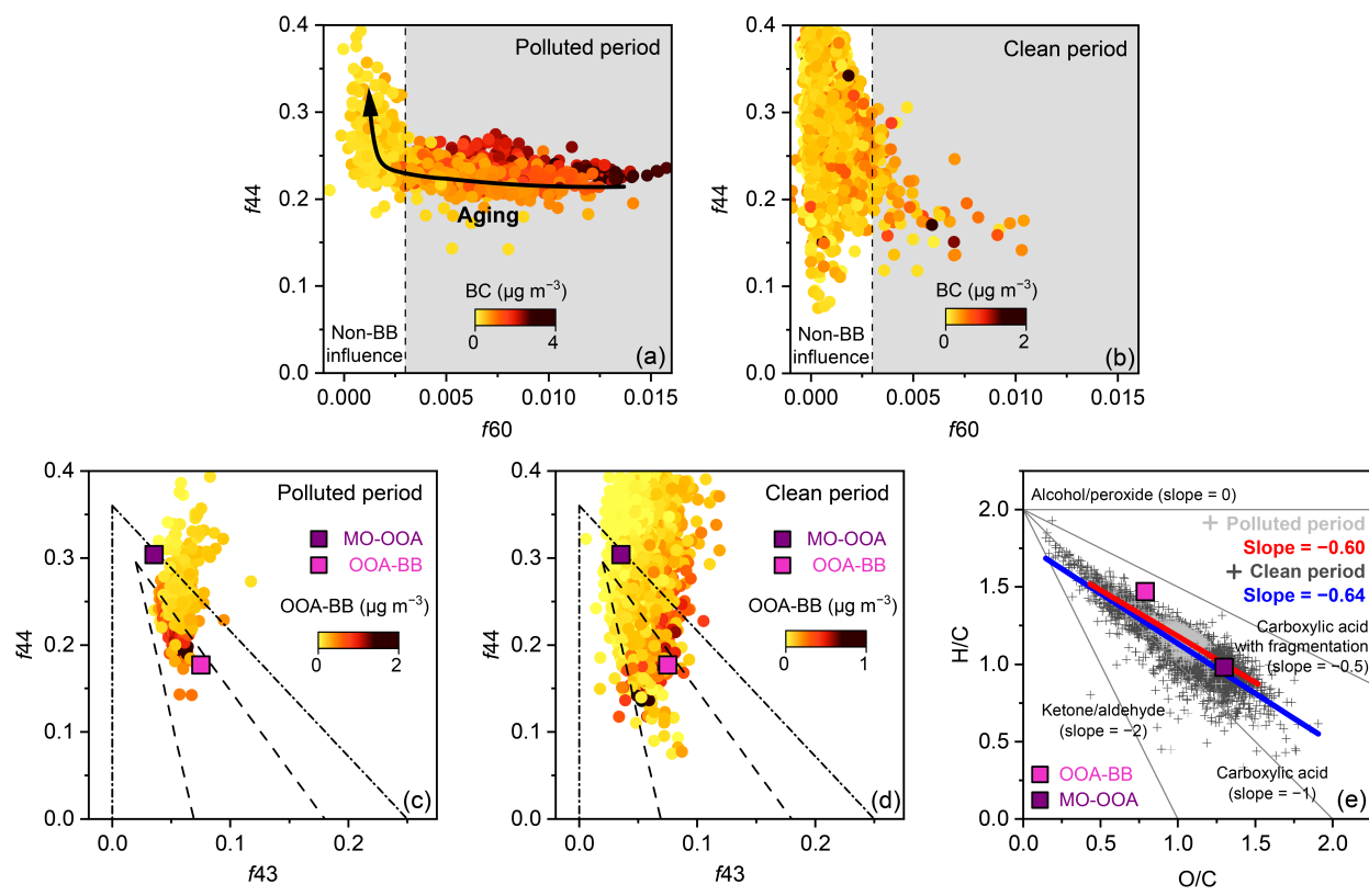
320 Figure 9. f_{44} versus f_{60} and f_{44} versus f_{43} during (a, c) polluted period and (b, d) clean period, as well as (e) Van Krevelen (VK) diagram of OA. The dashed lines and dashed-dotted lines in c–d refer to triangular regions that encompass ambient OOA (Ng et al., 2010) and laboratory measurements OOA (Lambe et al., 2011), respectively.
