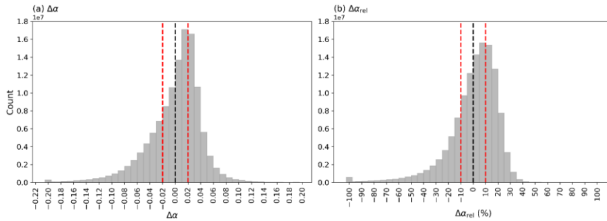
155 Figure 3. Distribution of the absolute difference ( \Delta\alpha ) (a) and the relative difference ( \Delta\alpha_{rel} ) (b) between the estimated (bin-averaged) and observed CERES albedo. The dashed black line marks zero difference, and the red dashed lines indicate the chosen accuracy thresholds ( \pm 0.02 for \Delta\alpha , \pm 10\% for \Delta\alpha_{rel} ).
