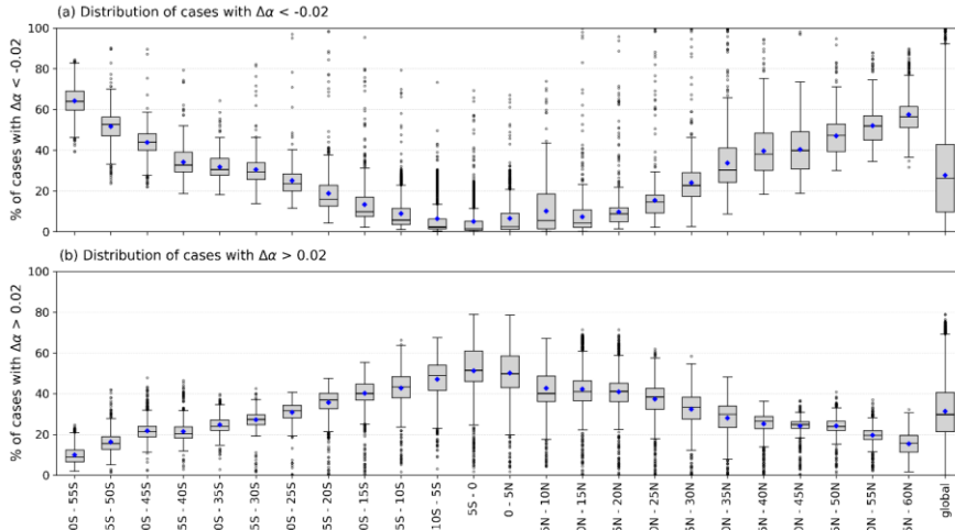
Figure 5. Distribution of (a) under- and (b) overestimated cases of albedo across 5° latitude bands. The boxes show the 25th–75th percentile range, with the line inside marking the median. The whiskers extend to the minimum and maximum values. Blue dots indicate the mean, and black dots mark outliers.
