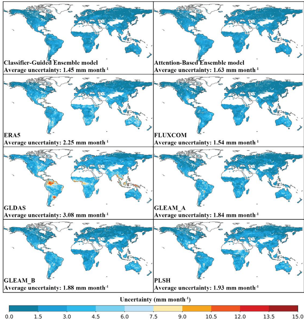
490 Figure 10. Average monthly uncertainty from 2005 to 2013 for Classifier-Guided Ensemble model, Attention-Based Ensemble model and other ET products.
