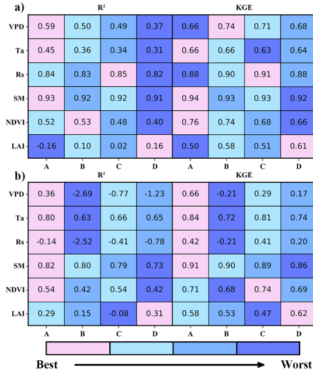
430 Figure 6. The comparison of different models (A Classifier-Guided Ensemble model, B Attention-Based Ensemble model, C ML model, D Hybrid model) under extreme conditions in the form of heatmaps. a) and b) represent the extreme samples sorted in ascending order within the 0th – 1st percentiles and 99th - 100th percentiles, respectively.
