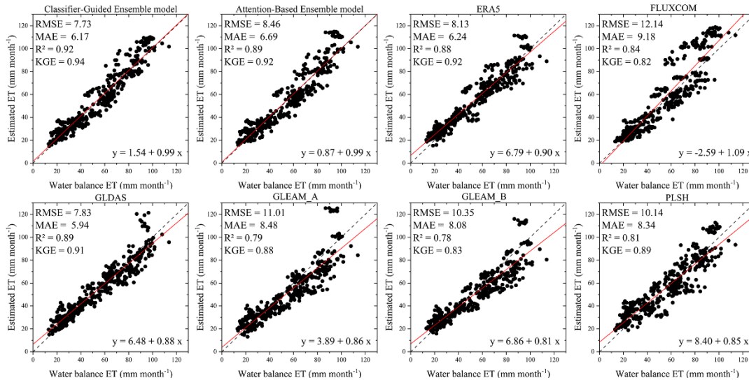
435 Figure 7. Scatterplot for the relationship between estimated ET and water balance ET (each point represents a catchment over a one-year period).
