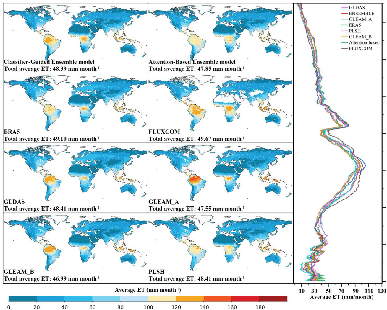
485 Figure 9. Average annual land evapotranspiration from 2005 to 2013 for Classifier-Guided Ensemble model, Attention-Based Ensemble model and other ET products. The latitudinal profiles of these datasets are shown in the right panel.
