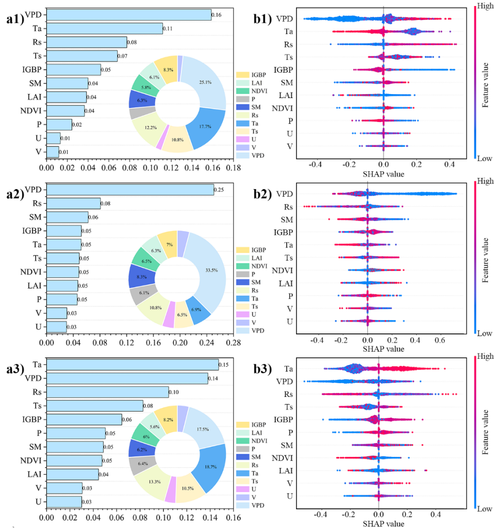
575 Figure 12. a) The bar plot and b) summary plot of the SHAP values for 1) ‘process-based algorithm-dominated’ type, 2) ‘Hybrid model-dominated’ type and 3) ‘ML model-dominated’ type. The bar plot exhibits the mean absolute SHAP values for each covariate and the summary plot exhibits the distribution of SHAP values.
