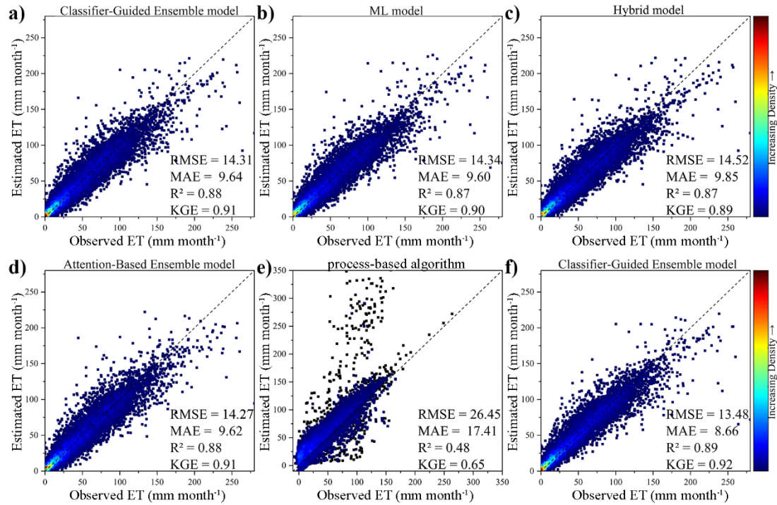
350 Figure 3. Performance of a) Classifier-Guided Ensemble model, b) ML model, c) Hybrid model, d) Attention-Based Ensemble model, e) process-based algorithm and f) Classifier-Guided Ensemble model (enhanced by additional global-scale training data) in ten-fold cross-validation.
