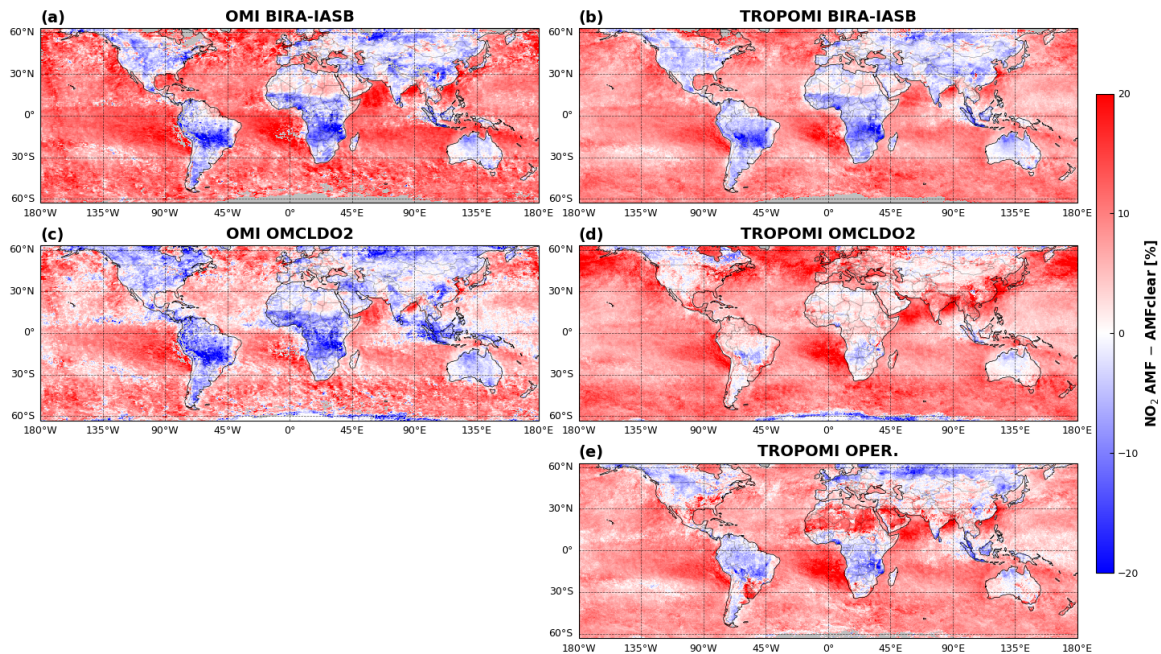
Figure A5. Monthly average impact of cloud corrections on the tropospheric NO 2 retrievals from OMI (left) and TROPOMI for October 2018. The NO 2 AMF is calculated using identical retrieval settings, differing only in the cloud correction approach applied. Data are gridded at a spatial resolution of 0.5°, including only observations with a cloud radiance fraction below 0.5.
