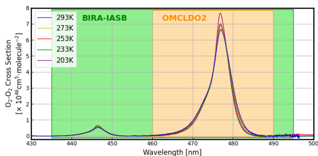
Figure 1. Temperature-dependent absorption cross-sections of O_2-O_2 collision pairs between 430 and 500 nm from Thalman and Volkamer (2013). The fitting window used for the OMCLDO2 retrieval is shown in orange; while the larger range used in this study is indicated in green.
