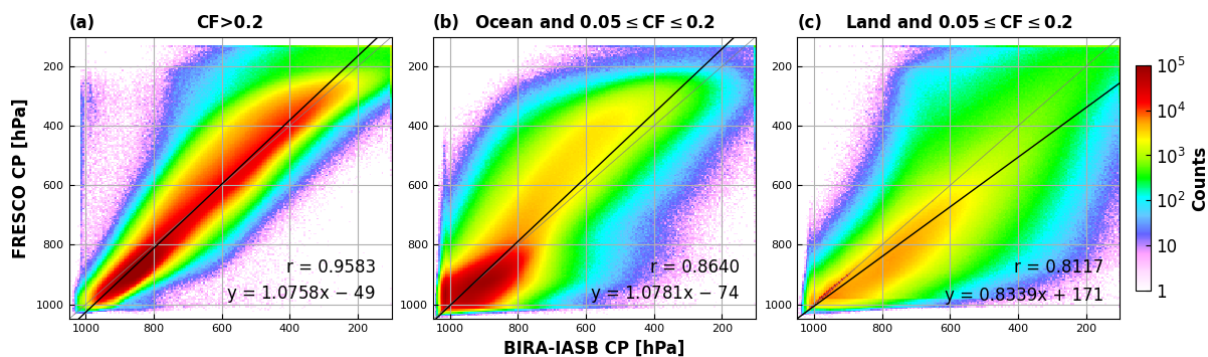
Figure A4. Similar as Fig. 13, but for comparison of TROPOMI cloud pressure retrievals between BIRA-IASB O 2 -O 2 and FRESKO.
