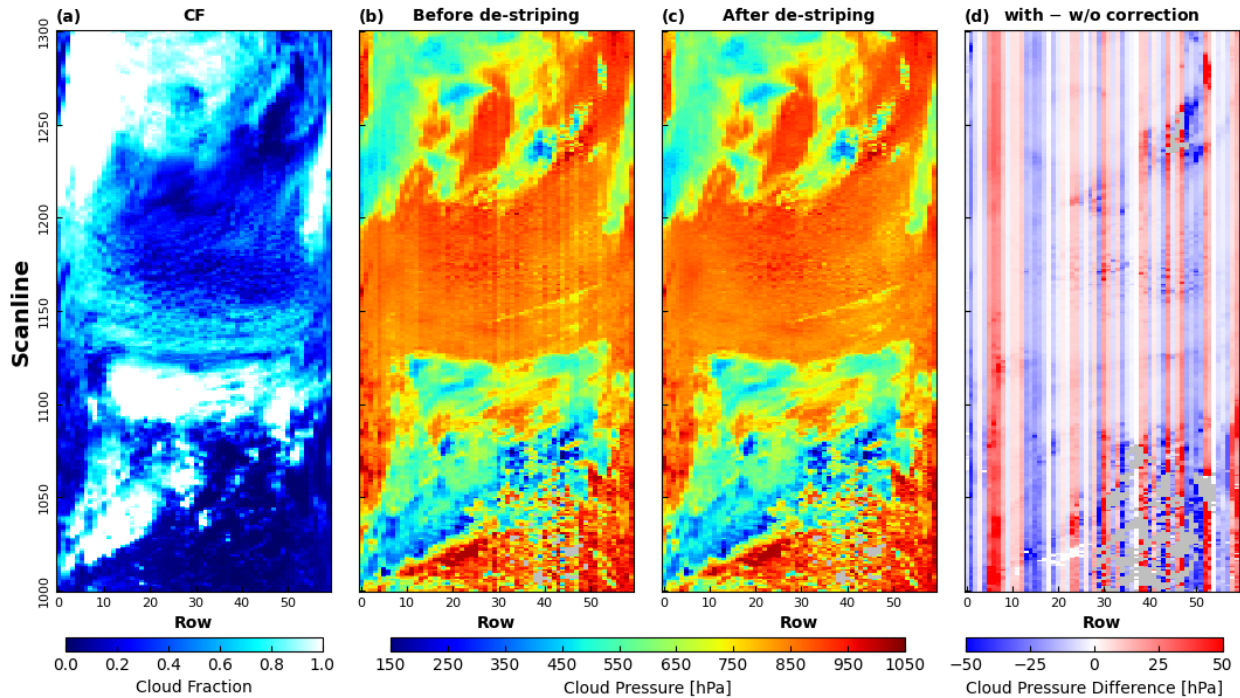
Figure 4. OMI O_2-O_2 cloud retrievals for BIRA-IASB cloud fraction (a), BIRA-IASB cloud pressure before (b) and after (c) de-stripping correction, and (d) difference between with and without correction. The data shown represent a segment of an OMI swath (scanlines 1000-1300) from orbit 1132 on 1 October 2004. Pixels with cloud fractions below 0.05 have been removed from the cloud pressure maps.
