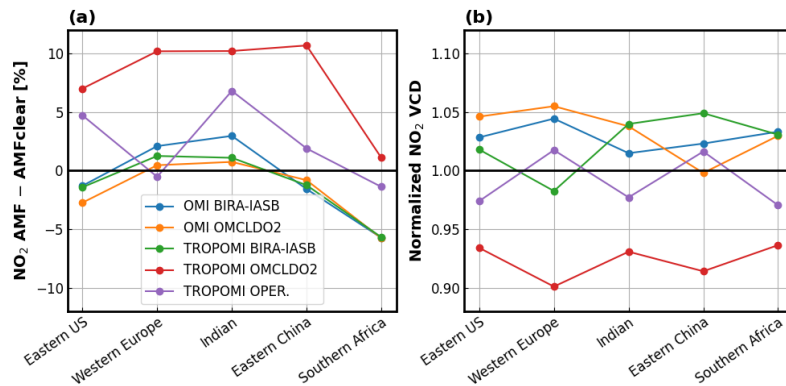
Figure 18. Impact of cloud corrections on \text{NO}_2 retrievals. Left panel: difference between the cloud-corrected AMF and the clear-sky AMF; right panel: difference in \text{NO}_2 VCD retrievals using the cloud-corrected AMF compared to those using the clear-sky AMF. Each \text{NO}_2 VCD value is normalized by the average of the five products for the corresponding region. Data analysis is based on monthly average maps for October 2018 over selected regions, as shown in Fig. 17. The colors represent \text{NO}_2 AMF calculations using various cloud correction methods and different sensors, while the x-axis indicates the selected regions.
