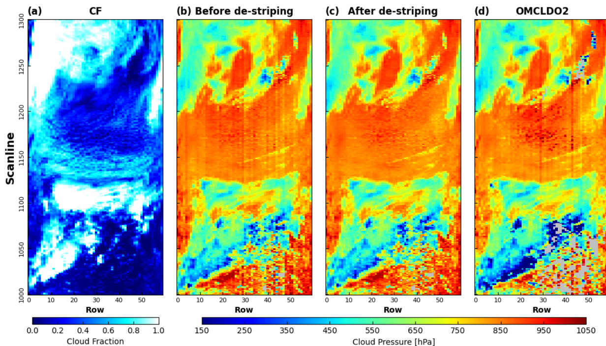
Figure 4. OMI O_2-O_2 cloud retrievals for BIRA-IASB cloud fraction (a), BIRA-IASB cloud pressure before (b) and after (c) de-striping correction, and (d) OMCLDO2 cloud pressure. The data shown represent a segment of an OMI swath (scanlines 1000–1300) from orbit 1132 on 1 October 2004. Pixels with cloud fractions below 0.01 have been removed from the cloud pressure maps.
