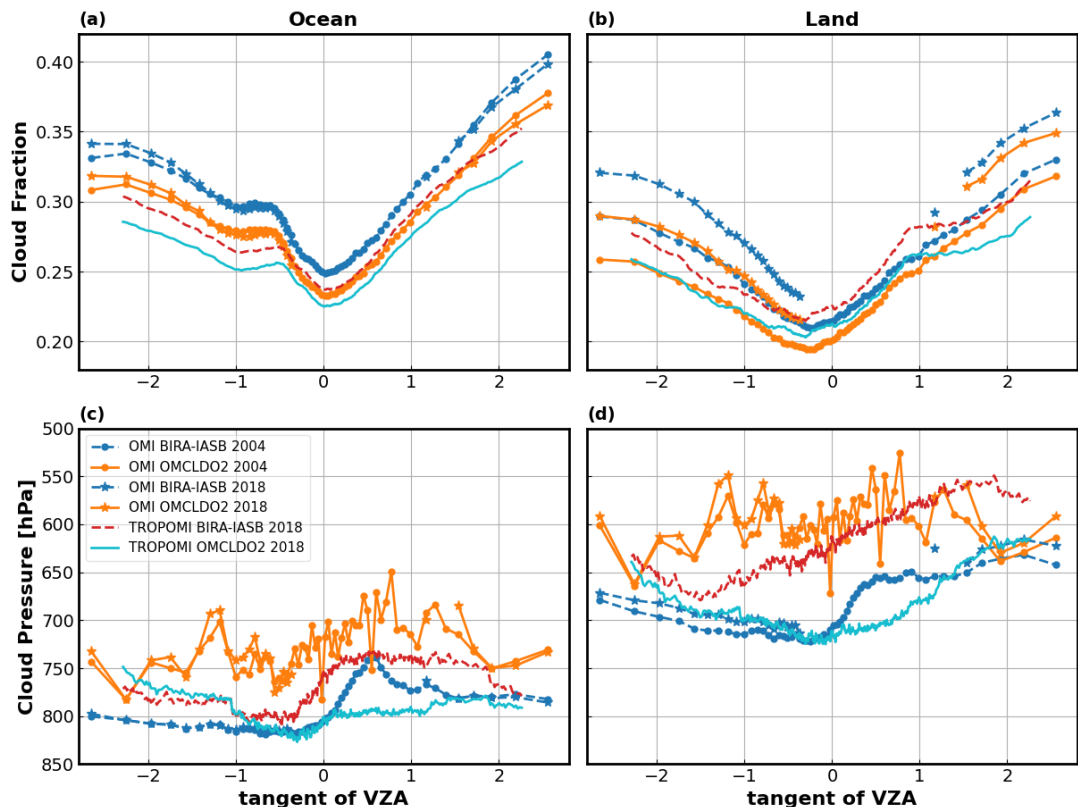
Figure 14. Across-track dependence of monthly-mean cloud retrievals from OMI and TROPOMI for October, based on the measurements between 50^{\circ}\text{S} and 50^{\circ}\text{N} latitudes. Panels show: (a) cloud fraction over oceans; (b) cloud fraction over land; (c) cloud pressure over oceans; (d) cloud pressure over land. The legend details the sensors, retrieval methods, and time periods included in the analysis.
