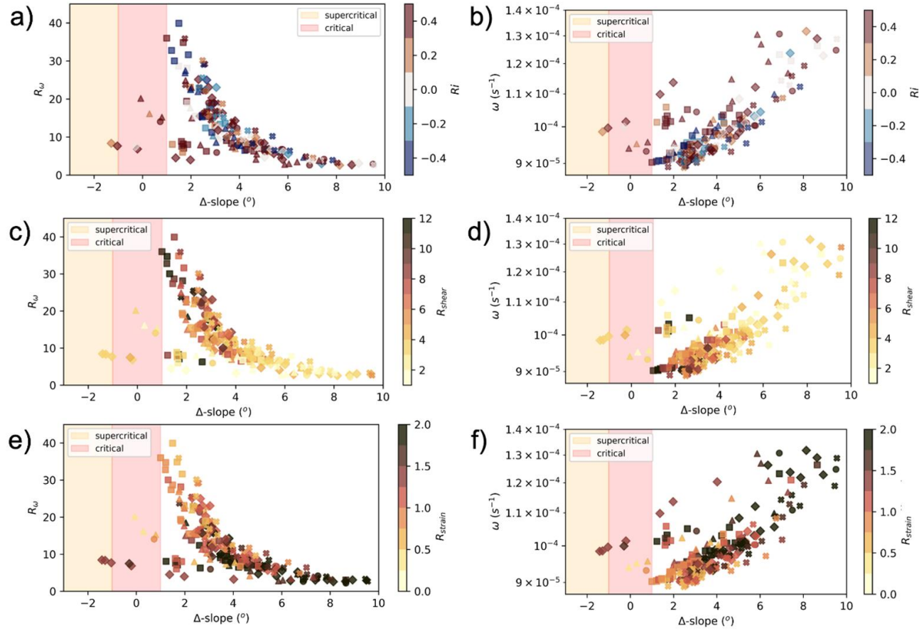
Figure 4. Distributions of R_\omega (left) and \omega (right) in the layer 360-920m distant from the bottom, in function of the difference between the associated beam angle and the bathymetry slope angle. Colours are used to indicate (a,b) a bulk Richardson number (in logarithmic scale), (c,d) the shear-to-shear-GM ratio, (e,f) the strain-to-strain-GM ratio. Higher values on the x-axis indicate a beam angle steeper, relative to the bathymetry slope, while lower values indicate a beam aligning with the slope. The critical range where the alignment is close to be parallel to the slope is arbitrarily marked by the shaded red area from -1 to 1 degrees, out of which a supercritical range is indicated in orange.
