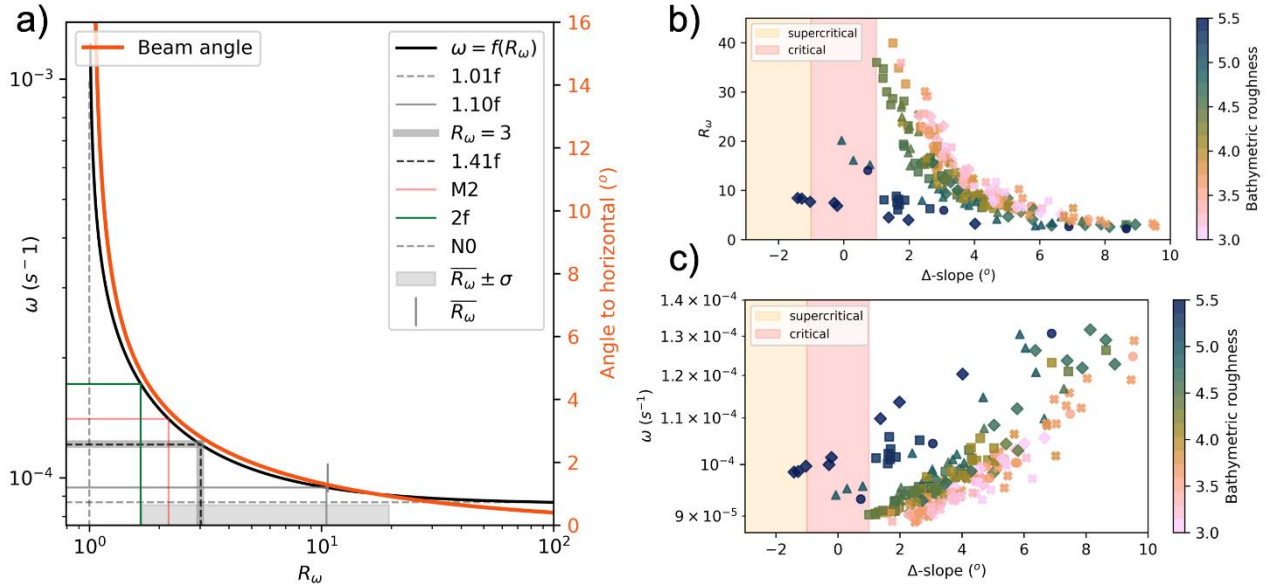
Figure 2. a) Correspondence between R_\omega and \omega (black), and the beam angle associated with R_\omega (orange), computed at the average latitude of the study (36.75°N). Typical values, from high to low R_\omega , are reported. The average R_\omega value of our study is indicated with the vertical line marker, and its distribution range is indicated by the gray area. b) Distributions of R_\omega and c) \omega in the layer 360-920 m distant from bottom, in function of the difference between the associated beam angle and the bathymetry slope ( \Delta -slope). Roughness is indicated in color. Higher values on the x-axis indicate a beam angle steeper, relative to the bathymetry slope, while lower values indicate a beam aligning with the slope. The critical range where the alignment is close to be parallel to the slope is arbitrarily marked by the shaded red area from -1 to 1 degrees, out of which a supercritical range is indicated in orange.
