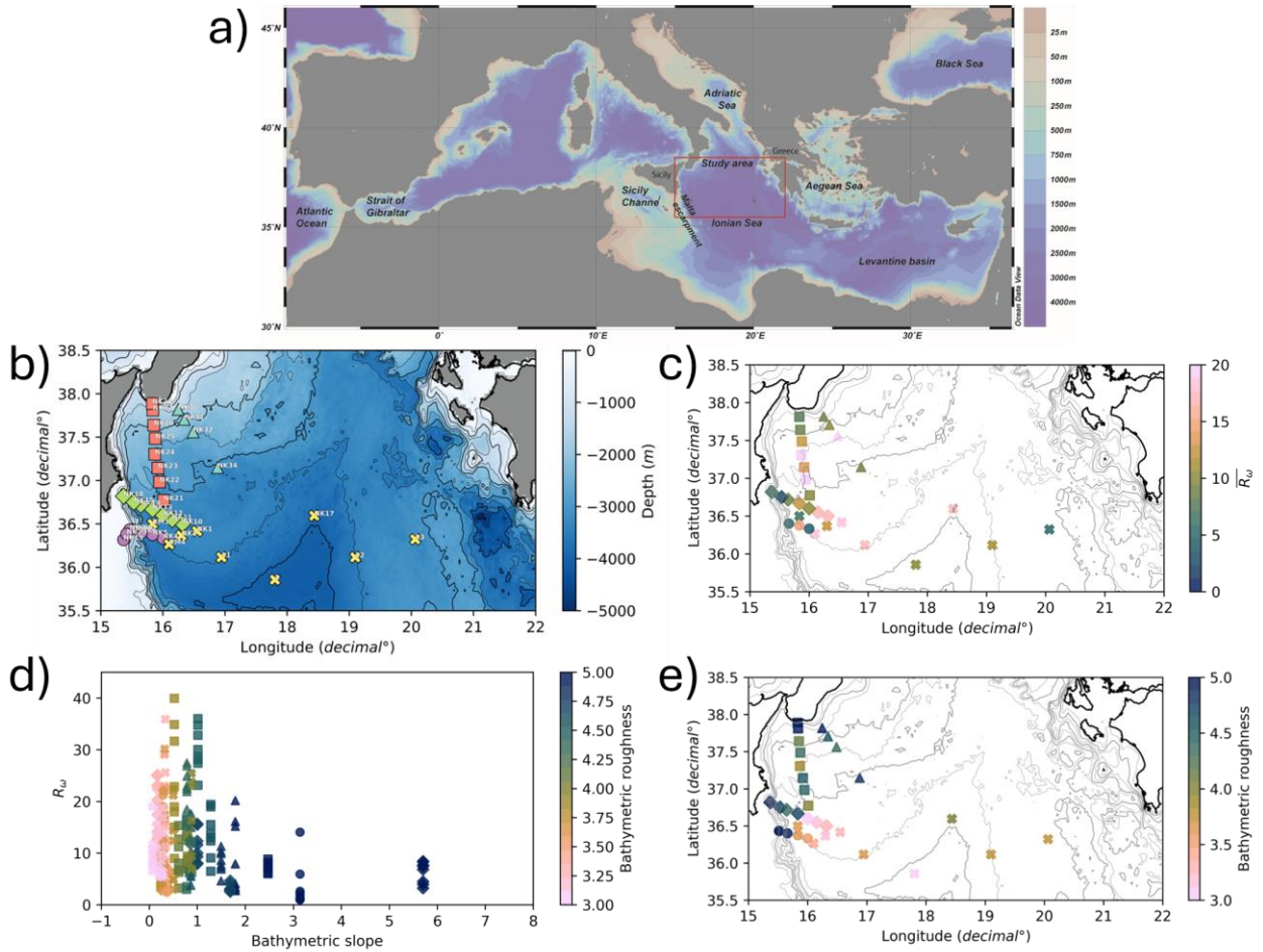
Figure 1. a) The Mediterranean Sea bathymetry and the main regional features that are discussed within the text; the red box indicates the study area. b) The Ionian Sea bathymetry and the main regional features that are discussed within the text; LADCP-CTD casts are grouped in five main hydrological transects: four shelf-to-plain transects, i.e., T1 ( \blacktriangle ), T2 ( \blacksquare ), T3 ( \blacklozenge ), T4 ( \bullet ), and one abyssal transect T5 ( \times ). c) Shear-to-strain ratio R_\omega at the bottom of the LADCP-CTD profiles, averaged from bins of 80m in the layer 360-920m distant from the bottom. d) Bottom roughness ( \log_{10} of \text{var}(z) ) at the cast sites. e) R_\omega as a function of bathymetric slope (x-axis), and roughness (in color).
