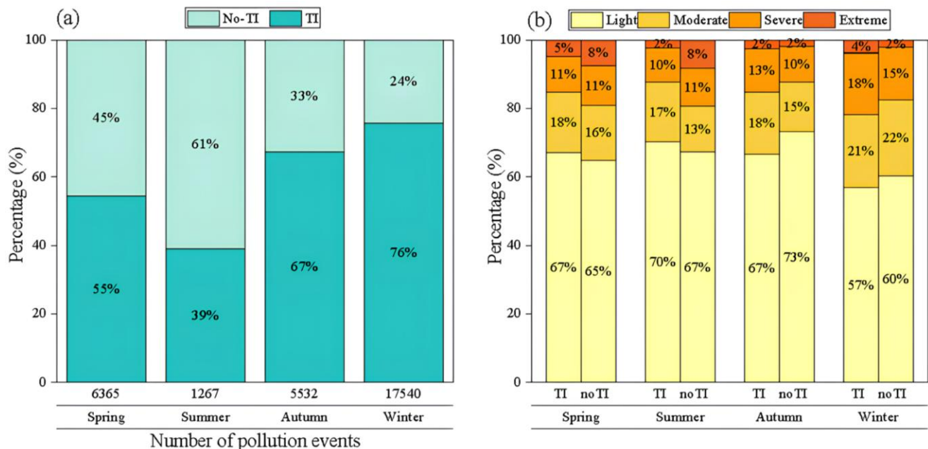
Fig. 7 (a) Frequency of inversion occurrence during polluted periods and (b) distribution of pollution levels in China (2016–2021).
