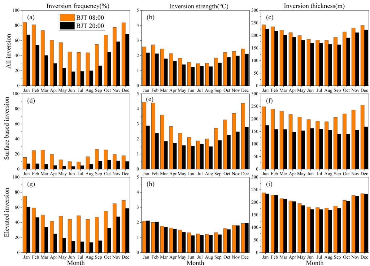
Fig. 4 Monthly variations of TI parameters in China (2016–2021).
