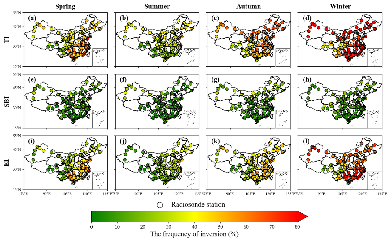
Fig. 3. Spatial and seasonal distribution of occurrence frequency for different types of TI. For more details about SBI, please refer to Fig. S15.
