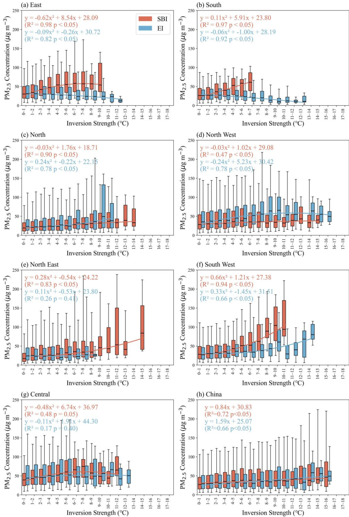
Fig.9 Fitting relationship between inversion strength and PM 2.5 concentration across seven regions of China from 2016 to 2021. The ends of the boxes, the ends of the bars, and the short line across each box represent the 25th and 75th percentiles, the 5th and 95th percentiles, and the median, respectively. Each strength interval contains a sample size \geq 10 .
