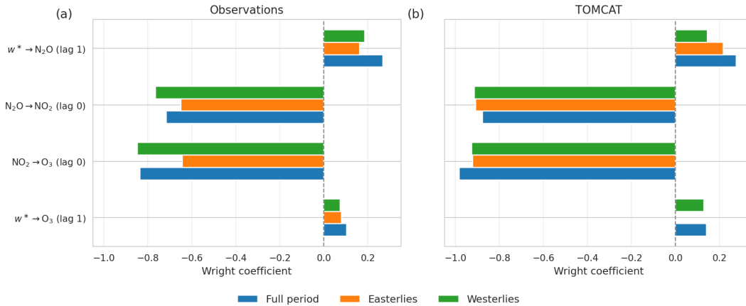
Figure 6. Regime-oriented direct causal effects from observations (a) observations and (b) the TOMCAT CTM simulation ( b ) for the full 2004-2021 period (blue), and for easterly (orange) and westerly (green) QBO regimes.
