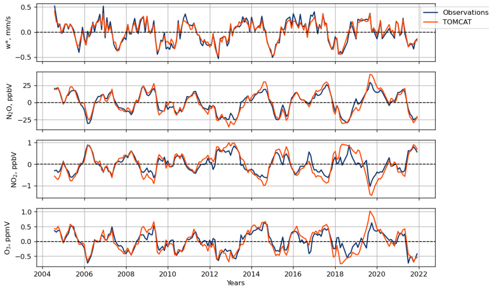
Figure B1. Monthly mean detrended anomalies over-in the tropical middle stratosphere during 2004-2021 in observations (blue) and the TOMCAT CTM simulation (orange). The TOMCAT CTM data is masked to match the occurrence of the observations.
