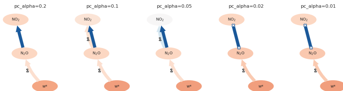
Figure C2. Causal graphs detected by the causal discovery algorithm from the TOMCAT CTM simulation for the period 2004-2021 with different significance level-levels \alpha_{pc} and \tau_{max}=2 .
