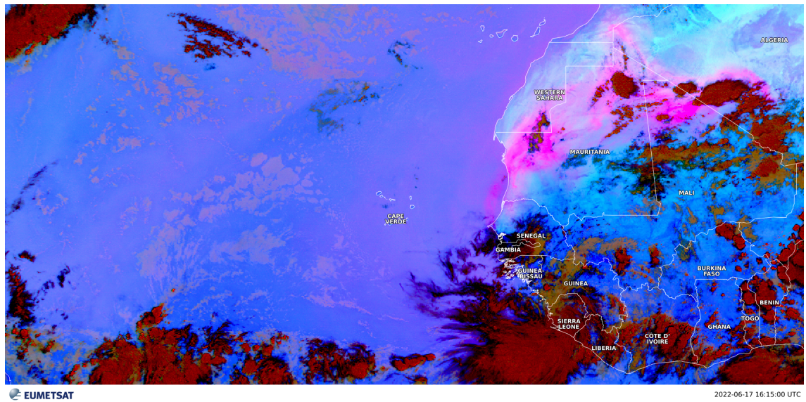
Figure D1. Same as Fig. 8, but for 17 June 2022 at 16:15 UTC.
