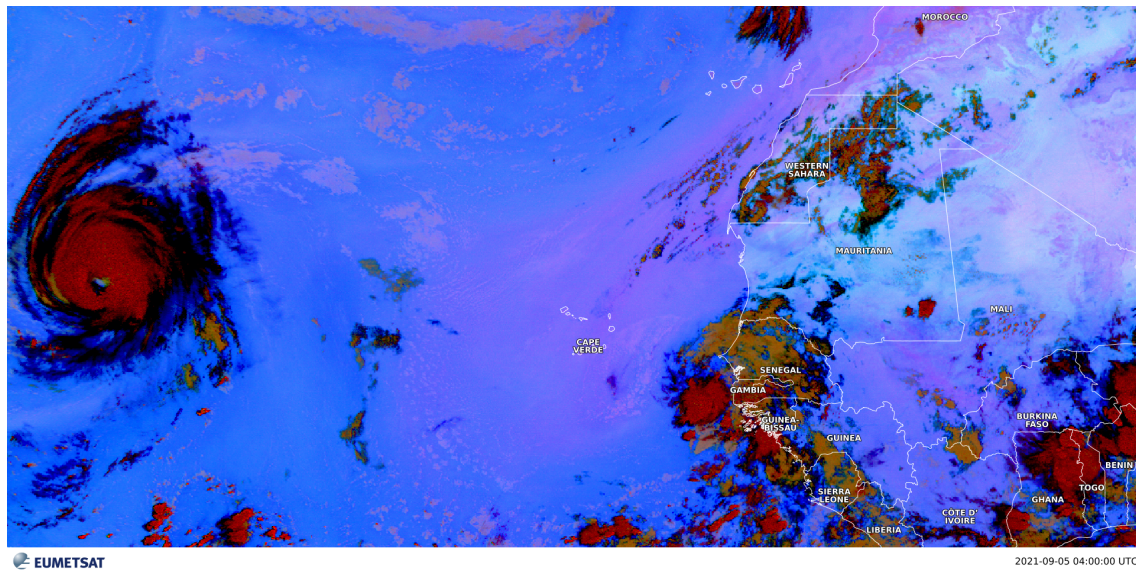
Figure 8. MSG-SEVIRI Dust product for 5 September 2021 at 04:00 UTC. Pink to violet colors indicate dust layers. Data accessed via the Eumetview platform ( https://view.eumetsat.int/ ; last access: 17 February 2026).
