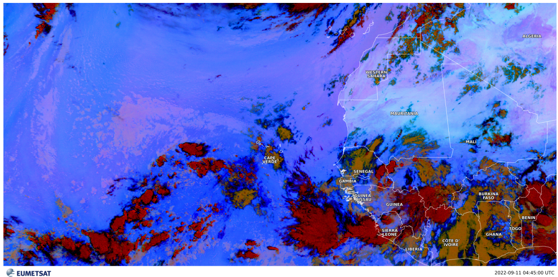
Figure D2. Same as Fig. 8, but for 11 September 2022 at 04:45 UTC.
