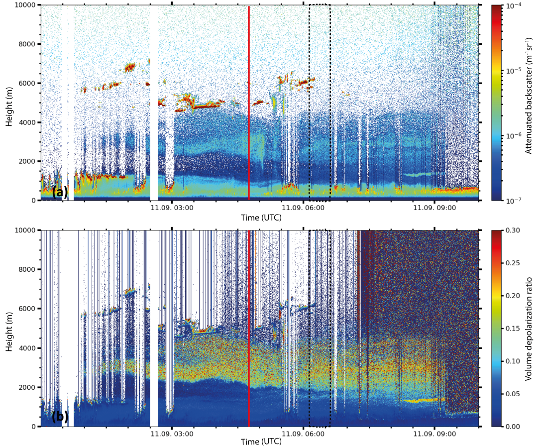
Figure 12. Similarly to Fig. 7, but for on 11 September 2022 between 00:00 and 10:00 UTC.
