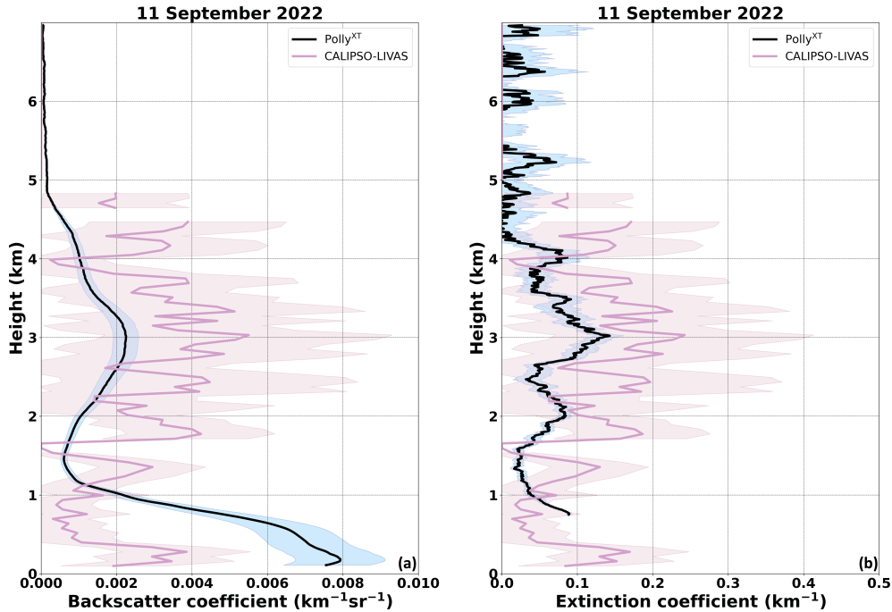
Figure 13. Same as Fig. 9, but for the case of 11 September 2022.
