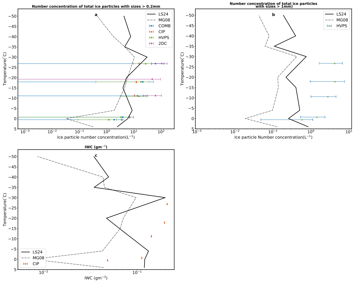
Figure 3. Predicted (a) concentration of ice particles with sizes > 0.2mm compared with observations from the 2DC, CIP, HVPS-3 probe and COMB, LS24 average bias is -58% and MG08 is -84.0%, normalized Root Mean Square Error (RMSE) for LS24 is 66% and for MG08 is 97% (b) ice number concentrations of all ice particles with size > 1 mm compared with aircraft observations from the HVPS-3 probe, LS24 average bias is -86% and MG08 is -95%, normalized RMSE for LS24 is 103% and for MG08 is 113% and (c) total IWC from the MG08 (dashdotted black line with square) and LS24 (solid black line) simulations, LS24 average bias is -32% and MG08 is -66%, normalized RMSE for LS24 is 43% and for MG08 is 65%. Error bars shown are standard errors of observation samples.
