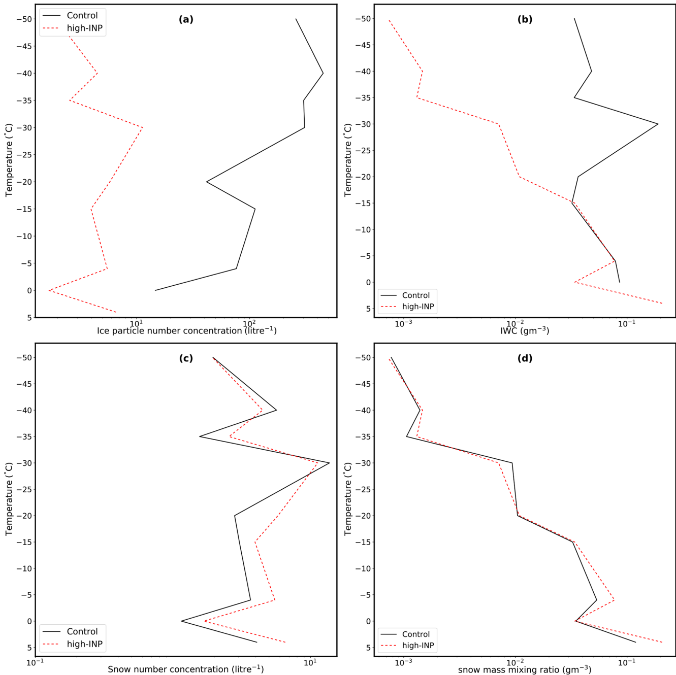
Figure 7. Predicted (a) ice particle number concentration ( L^{-1} ), (b) IWC ( g\ m^{-3} ), (c) snow number concentration ( L^{-1} ), and (d) snow mass content ( g\ m^{-3} ). The cloud microphysical properties are conditionally averaged (over stratiform cloud regions only) over the entire simulation period.
