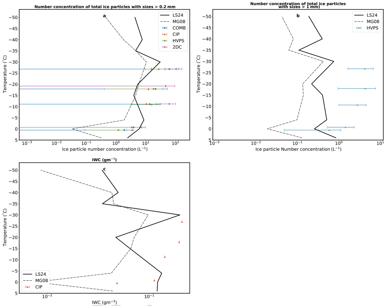
Figure 3. Predicted (a) concentration of ice particles with sizes > 0.2 mm compared with observations from the 2DC, CIP, HVPS-3 probe and COMB, LS24 average bias is -58\% and MG08 is -84.0\% , normalized Root Mean Square Error (RMSE) for LS24 is 66\% and for MG08 is 97\% (b) ice number concentrations of all ice particles with size > 1 mm compared with aircraft observations from the HVPS-3 probe, LS24 average bias is -86\% and MG08 is -95\% , normalized RMSE for LS24 is 103\% and for MG08 is 113\% and (c) total IWC from the MG08 (dash-dotted black line with square) and LS24 (solid black line) simulations, LS24 average bias is -32\% and MG08 is -66\% , normalized RMSE for LS24 is 43\% and for MG08 is 65\% . Error bars shown are standard errors of observation samples.
