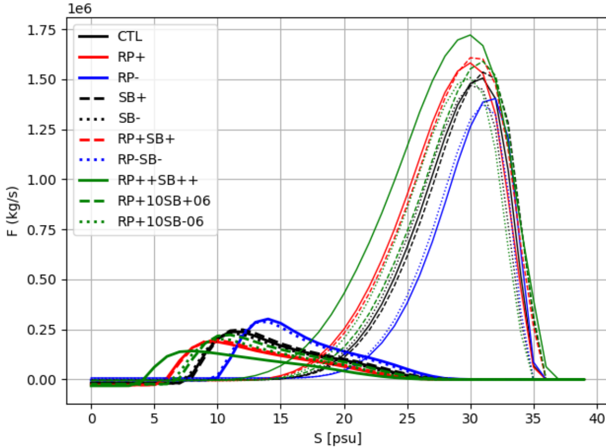
Figure 9: Cumulated inflows of salt, F , in water with salinity larger than s as defined in (9), and for the period 1990 - 2017. Thick lines are for transports through the sill transect, and thin lines are for transports through the northern Kattegat transect. Inflows happen at salinity intervals with negative gradient of F , whereas outflows happen at salinity intervals with positive gradient.
