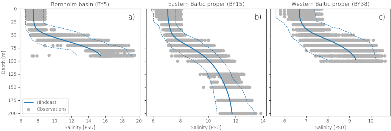
205 Figure 2: Salinity profiles at three selected stations in the Baltic Sea for the period 1970 to 2017. The blue solid lines represent the temporal mean of the hindcast experiment, and the dashed lines the 5th and 95th percentiles. The grey dots represent observed salinity from the SHARK database.
