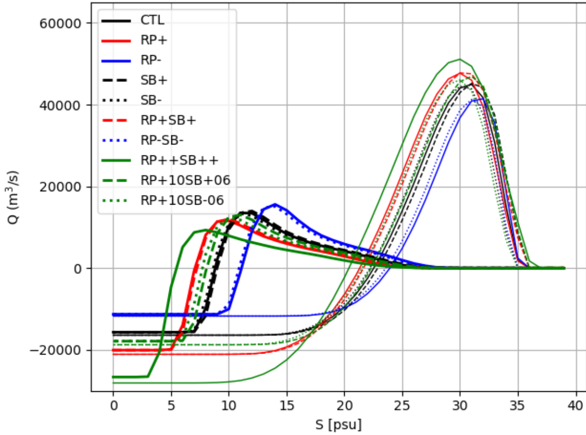
Figure 8: Cumulated inflows of volume, Q , of water with salinity larger than s as defined in (8), and for the period 1990 - 2017. Thick lines are for transports through the sill transect, and thin lines are for transports through the northern Kattegat transect. Inflows happen at salinity intervals with negative gradient of Q , whereas outflows happen at salinity intervals with positive gradient.
