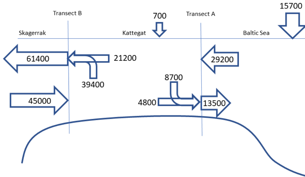
Figure 10: Mean volume fluxes for the period 1990 - 2017 in m³/s. The vertical arrows show the net inputs of freshwater to the Baltic Sea inside transect A and to the region between transects A and B. Large horizontal arrows show in- and outflows through the transects. Smaller horizontal and bended arrows show the contributions from inflow (outflow) through transect B (A), and recirculated outflow (inflow) from transect A (B) to the inflow (outflow). The recirculation fluxes are calculated with \gamma = 0 , in equations (20) and (21), i.e. assuming that the local freshwater contribution between transects A and B are added to the outflow through transect B.
