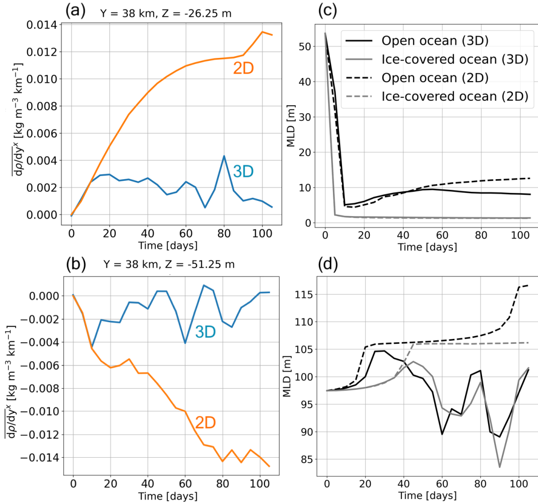
Figure 3. (a,c) Arctic summer, (b,d) Arctic winter. The left panels (a,b) display the time evolution of the zonally averaged meridional density gradient in 2D and 3D simulations at y = 38 km, and z = -26.25 m (summer) and z = -51.25 m (winter). The right panels (c,d) display the time evolution of ice-covered and open ocean spatially averaged MLDs for 3D (solid lines) and 2D (dashed lines) simulations.
