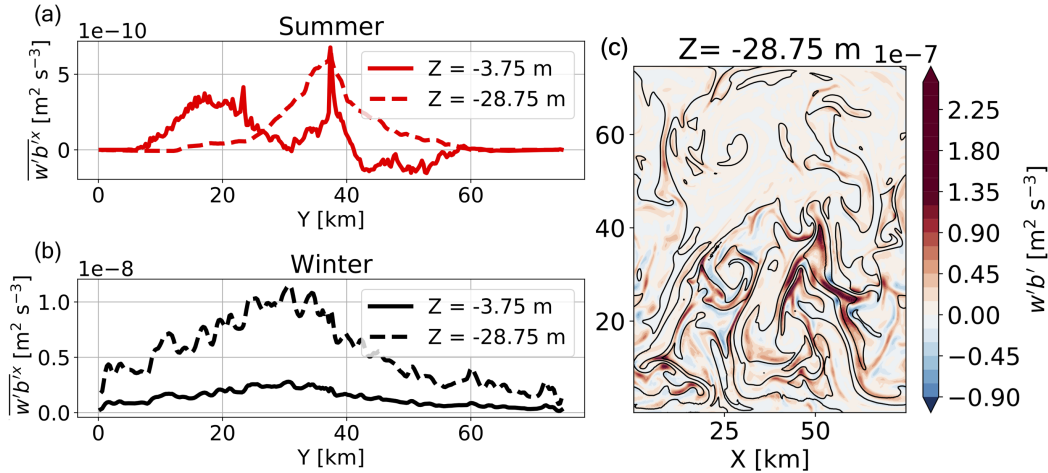
Figure 5. Time-averaged \overline{w'b'^x} at the surface and at z = -28.75 m for (a) Arctic summer and (b) Arctic winter. Averages are taken over the full simulation length of 110 days. Note the different scales on the y-axis between (a) and (b). (c) spatial variations of w'b' in the Arctic winter simulation at day 110, with salinity contours, spaced at 0.02 \text{ g kg}^{-1} , shown in black.
