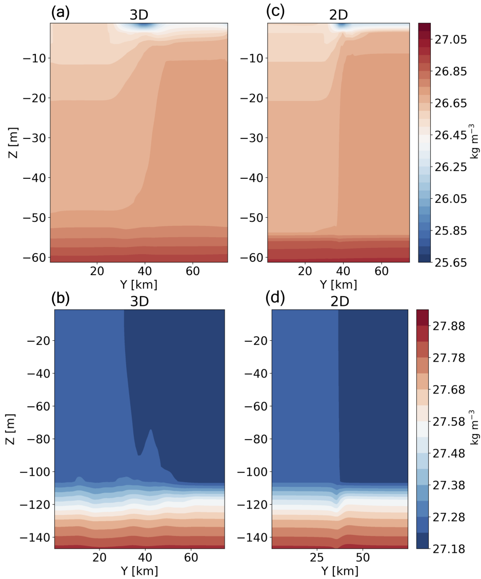
Figure 2. (a,c) Arctic summer and (b,d) Arctic winter. Snapshots of potential density (referenced at the surface) for the (a,b) 3D (zonal mean) and (c,d) 2D simulations at day 50.
