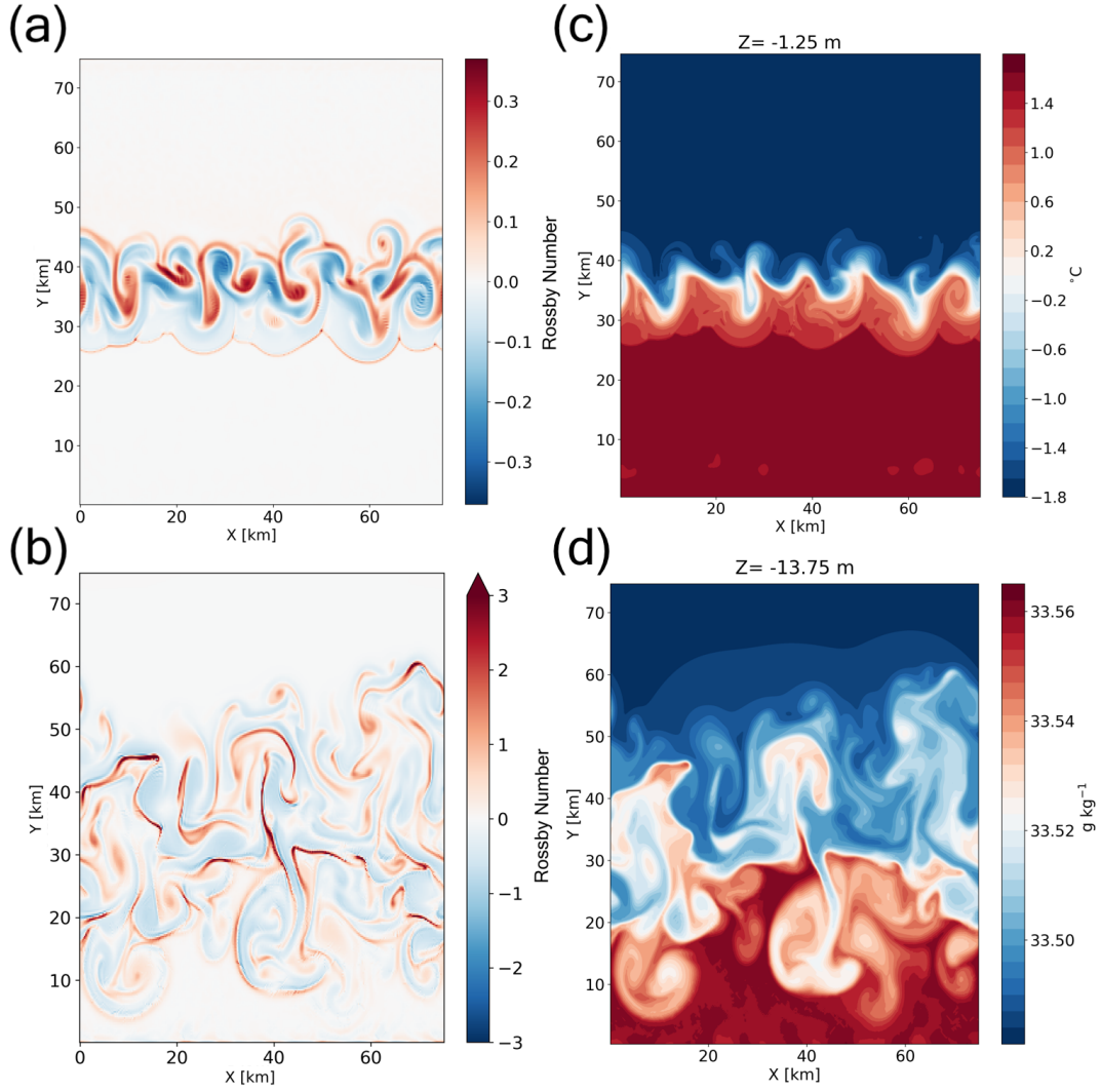
Figure 4. Snapshots of properties at day 50 for the Arctic case: (a,c) summer, (b,d) winter. The left panels (a,b) display the Rossby number ( =|\zeta|/f ) at the surface (note the differing colourbars). The top right panel (c) displays the sea surface temperature, and the bottom right panel (d) displays the salinity at a depth of z = -13.75 m.
