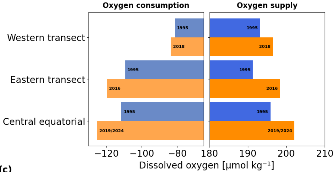
Figure 8: Mean oxygen supply (oxygen due to mixing), measured oxygen, and biological oxygen consumption averaged over (a) Arabian Sea OMZ (AS OMZ, \text{O}_2 < 20 \mu\text{mol kg}^{-1} , depth range 150–1000 m), (b) Bay of Bengal OMZ (BoB OMZ, \text{O}_2 < 20 \mu\text{mol kg}^{-1} , depth range 150–700 m), The measured oxygen values represent average dissolved oxygen within the OMZs at the same depth range above (c) comparing oxygen supply and consumption across the western (WIO, 1995 and 2018), eastern (EIO, 1995 and 2016), and central equatorial transects (CIO, 1995 and 2019/2024).
