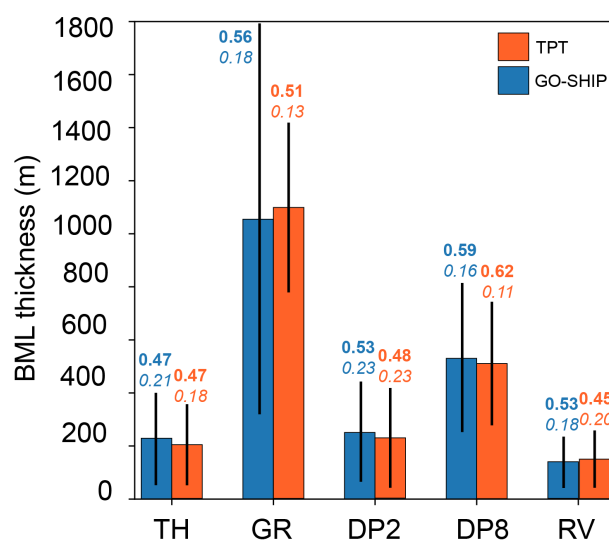
Figure 4. Average bottom mixed layer (BML) thickness (m) for the threshold method (TH), gradient method (GR), Douglas-Peucker method using an \epsilon of 0.002 (DP2), Douglas-Peucker method using an \epsilon of 0.080 (DP8) and the relative variance method (RV). The BML thickness is calculated using the TPT Expedition profiles (orange) and GO-SHIP profiles (blue) with the length of the line indicating the range of the thickness. Bold values above the bars are the mean quality index (QI) and the italicised values are the standard deviation of the QI.
