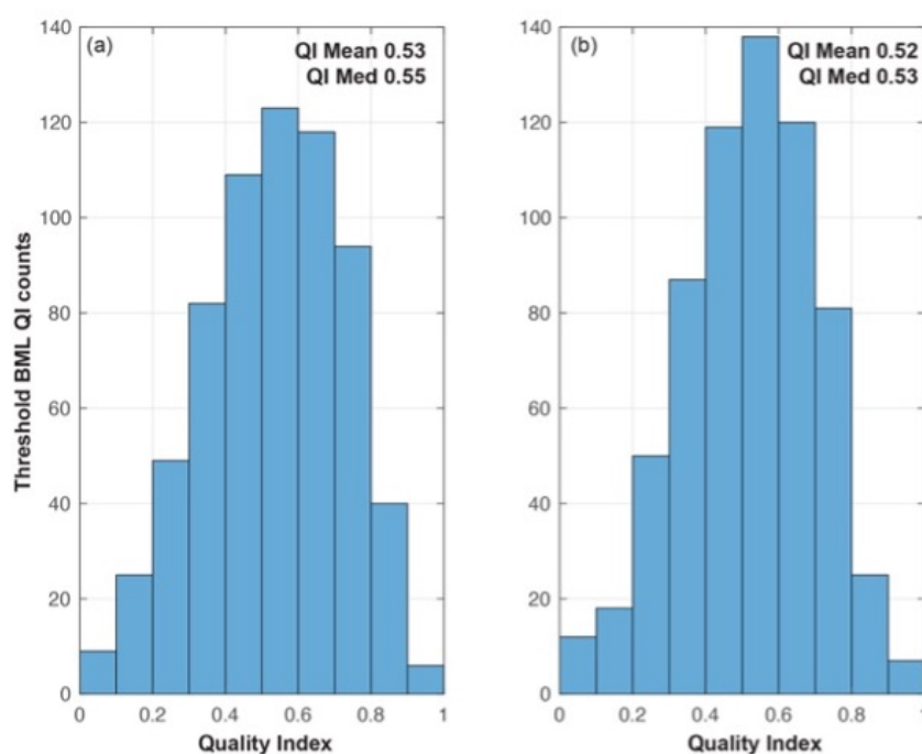
Figure A2. Histogram plots of the quality index values from the threshold BML height based on different threshold values of conservative temperature ( \Theta ) as (a) 0.001°C, (b) 0.002°C, (c) 0.003°C, (d) 0.004°C and (e) 0.005°C
