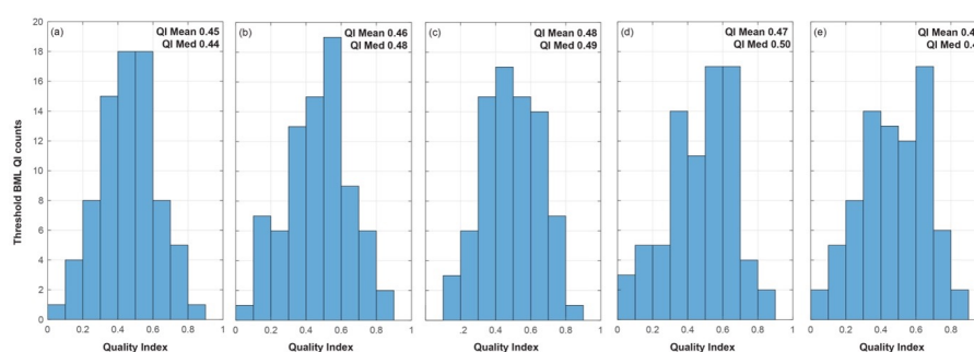
Figure A1. Histogram plots of the quality index values from the threshold BML height based on different threshold values of conservative temperature ( \Theta ) as (a) 0.001°C, (b) 0.002°C, (c) 0.003°C, (d) 0.004°C and (e) 0.005°C
