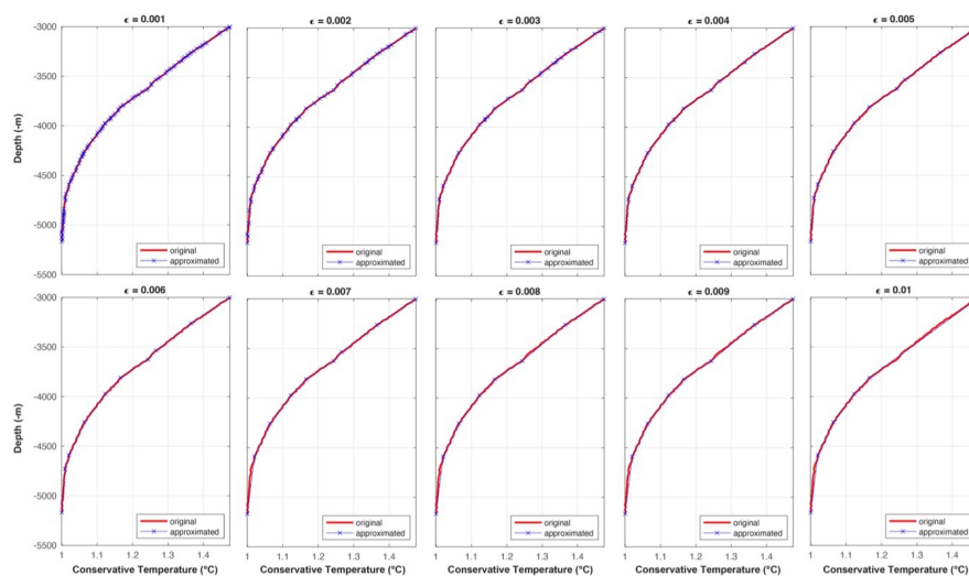
Figure A3. Douglas-Peucker Algorithm output (approximated, in blue) for different values of \epsilon and original profile of TP2OM35400 in red as an example
