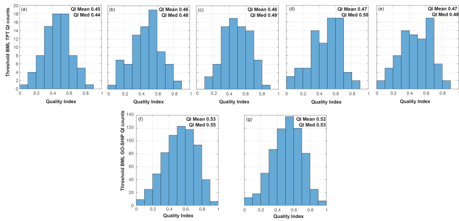
Figure A2. Histogram plots of the quality index values from the threshold BML height based on different threshold values of conservative temperature ( \Theta ) for TPT profiles as (a) 0.001^{\circ}\text{C} , (b) 0.002^{\circ}\text{C} , (c) 0.003^{\circ}\text{C} , (d) 0.004^{\circ}\text{C} and (e) 0.005^{\circ}\text{C} and for the GO-SHIP profiles as (f) 0.003^{\circ}\text{C} and (g) 0.005^{\circ}\text{C}
