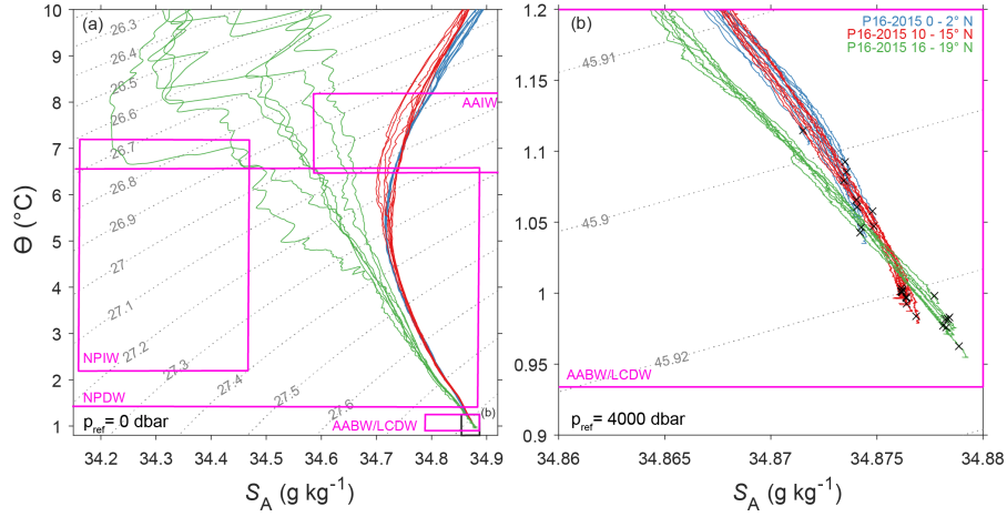
Figure 10. Conservative temperature ( \Theta , °) - Absolute Salinity ( S_A , \text{g kg}^{-1} ) plots for latitudinal sections of the P16 line for the 2015 occupation between 0 - 2°N (blue), 10 - 15°N (red) and 16 - 19°N (green). (a) Wider portion of the water column with the (b) limits outlined. In (a) the dashed contour lines show the potential density referenced to the 0 dbar ( \sigma_0 ) and in (b) the dashed lines show the potential density referenced to 4000 dbar ( \sigma_4 ). \Theta - S_A North Pacific water mass properties are shown in magenta Fuhr et al. (2021) and the BML for the profile is displayed with a black X. NPIW = North Pacific Intermediate Water, AAIW = Antarctic Intermediate Water, NPDW = North Pacific Deep Water, AABW = Antarctic Bottom Water, used here interchangeably with Lower Circumpolar Deep Water (LCDW). Displayed and calculated with the TEOS-10 toolbox McDougall and Barker (2011)
