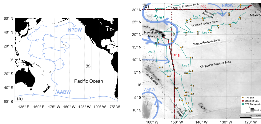
Figure 1. (a) Bottom water circulation pathways through the Pacific Ocean based on existing research (Kawabe and Fujio (2010); Oka and Niwa (2013); Hautala (2018)) with (b) insert as the extent of the study region. AABW = Antarctic Bottom Water, NPDW = North Pacific Deep Water (b) Study region boundary, locations, and features, including a regional bathymetric grid. Orange triangles are the Trans-Pacific Transit Expedition deployment locations with numbers as the site number within the associated leg. The R/V Dagon multibeam echosounder coverage is displayed in green. Note that Leg 1 is not used in this analysis. The GO-SHIP repeat hydrographic lines and deployment locations are marked with red circles (P16 and P02). Blue arrows are bottom water circulation pathways adapted from previous studies. Background regional bathymetry is from the Global Multi-Resolution Topography (GMRT) Synthesis (Ryan et al. (2009)) Released CC BY 4.0 Deep | Attribution 4.0 International | Creative Commons.
