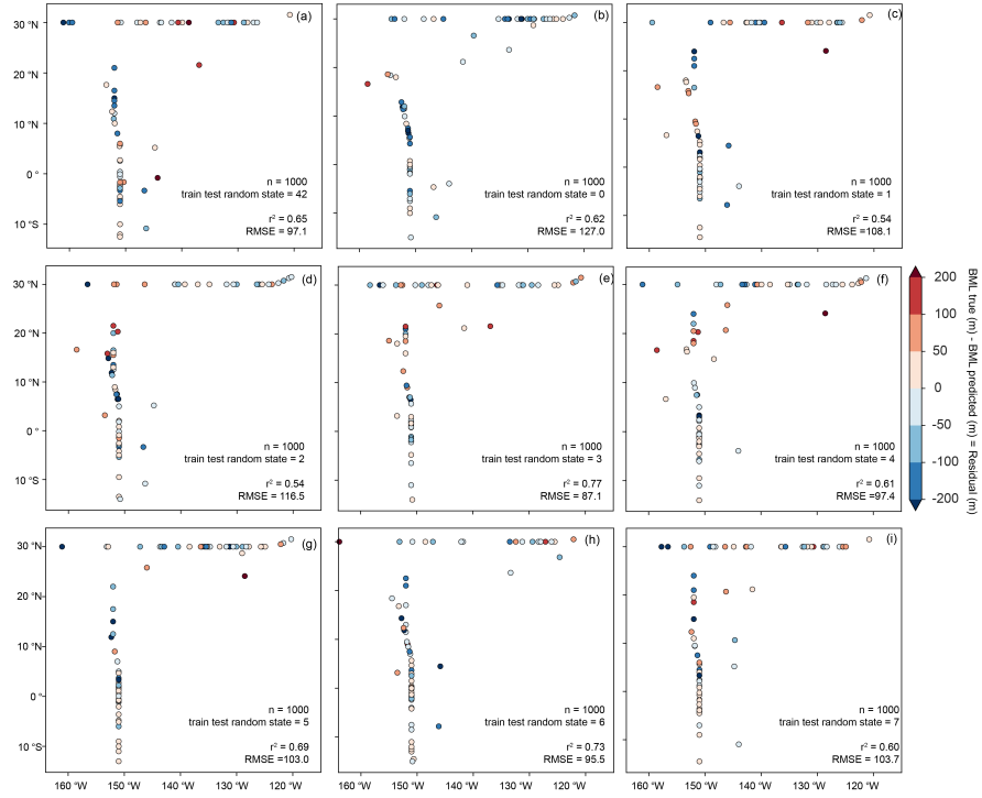
Figure 9. Spatial plots of the BML residual (m) (BML true - BML predicted) for the train test random_state values used to train the Random Forest Regressor with the number of iterations = 1000, generating a spread of the data for random_state equal to (a) 42 and (b) - (i) for 0 to 7. The correlation coefficient and the Root Mean Squared Error (RMSE) is displayed on each figure.
