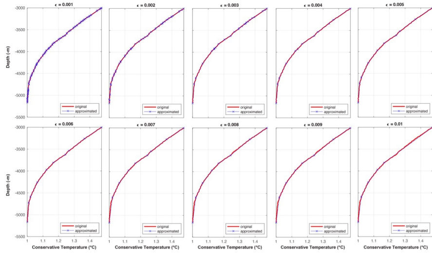
Figure A3. Douglas-Peucker Algorithm output (approximated, in blue) for different values of \varepsilon and original profile of TP2_O M3_5 400 in red as an example
