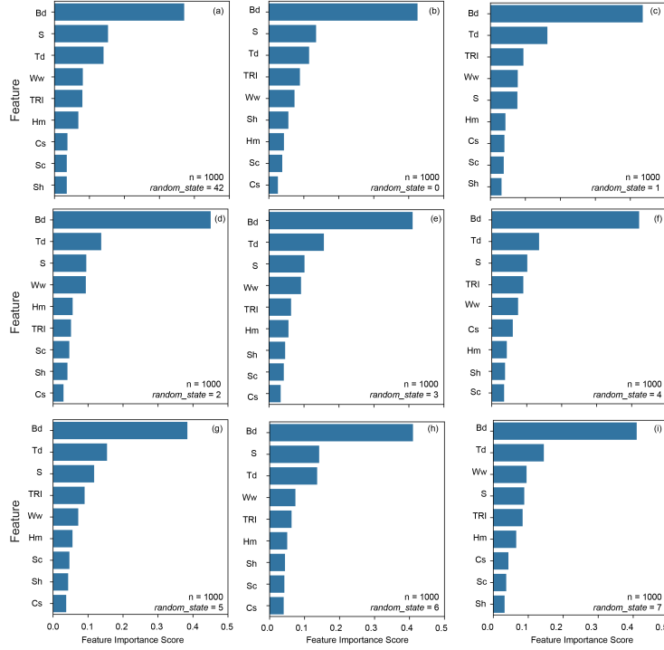
Figure 8. Feature importance scores for each feature output from the number of iterations ( n ) = 1000 for the train test split random_state values of the 80-20 data split for (a) 42 and (b) - (i) for 0 to 7 for the Random Forest Regressor. Bd = bottom depth, S = slope, TRI = terrain roughness index, Td = total internal tide energy dissipation, Sh = low-mode dissipation from shoaling, Ww = low-mode dissipation from wave-wave interaction, Cs = low-mode dissipation from critical slopes, Sc = low-mode dissipation from scattering and Hm = high-mode dissipation from local processes.
