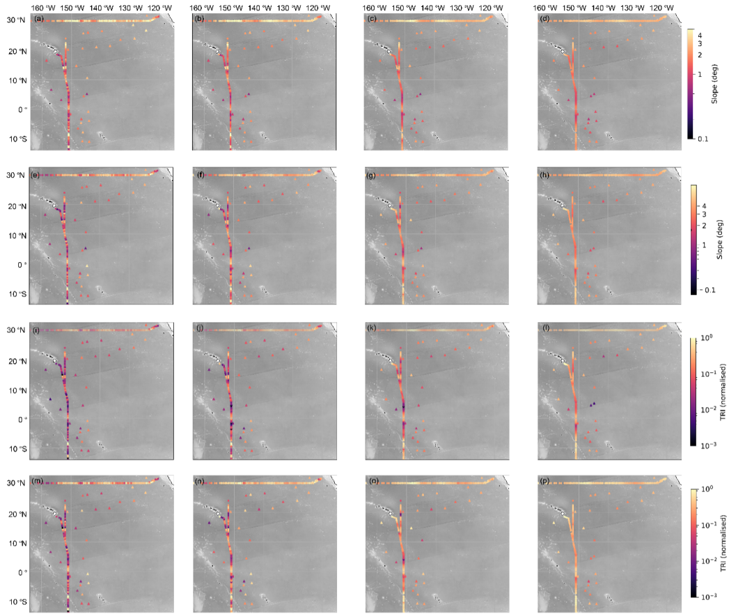
Figure A4. GO-SHIP (circle) and TPT (triangle) site variables of the (a) – (d) mean slope over 25, 50, 100 and 200 km buffer zones respectively (deg) and the (e) - (h) standard deviation of slope over the 25, 50, 100 and 200 km buffer zones respectively, (i) – (l) the mean normalised terrain roughness index (TRI) over the 25, 50, 100 and 200 km buffer zones respectively and (m) – (p) displaying the normalised standard deviation of the TRI. For the multiple TPT sites within close proximity ( \leq 3 km), TRI and slope are on the centre point. The background regional bathymetry is from the Global Multi-Resolution Topography (GMRT) Synthesis Released CC BY 4.0 Deep | Attribution 4.0 International | Creative Commons Ryan et al. (2009)
