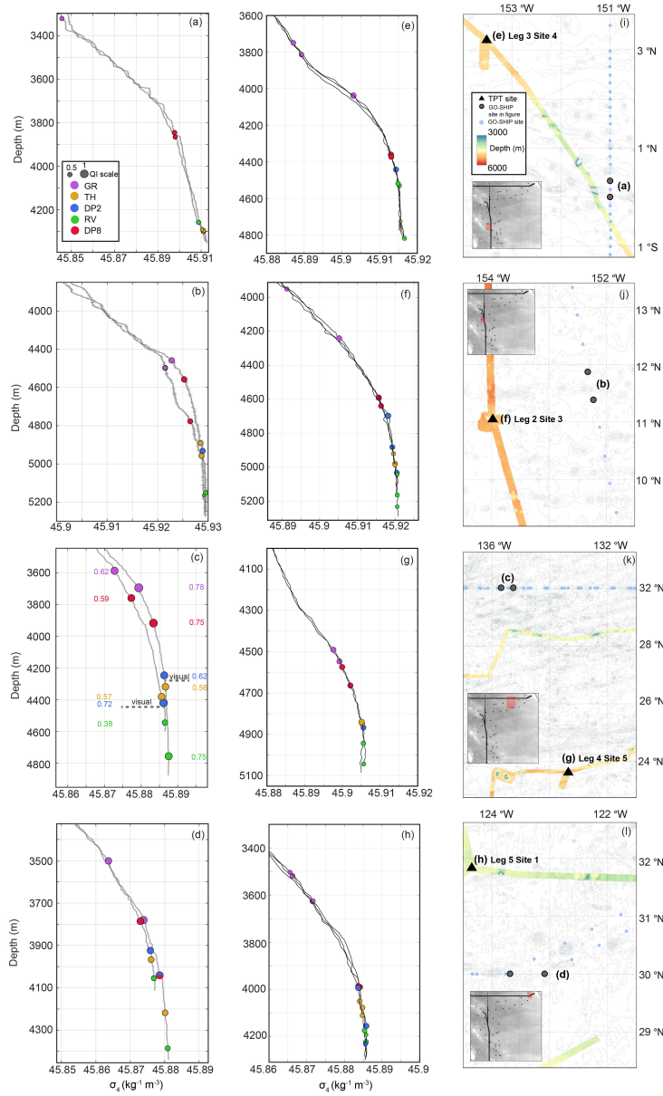
Figure 2. Example profiles of \sigma_4 and BML thickness outputs from (a) to (h). Color and size of the marker correspond to the method and the quality index (QI) of the BML (a). The map and inserts in (i) to (l) detail the locations of the profiles shown in the respective subplot. Grey map shows the study region with GEBCO bathymetry and sites (key in (i); see Figure 1 for more detail), the red region the extent of the figure and black points indicating all profiles used. Blue circles are GO-SHIP with light blue indicating profiles used but not displayed, black triangles are TPT locations. (a) P16 GO-SHIP profiles in 2002 between 0^\circ and 0.5^\circ N and (b) in 2015 between 12^\circ and 13^\circ N, (c) P02 GO-SHIP profiles in 2022 between 135^\circ and 136^\circ W and (d) in 2022 between 124^\circ and 123^\circ W. (e) TPT voyage Leg 3 Site 4, (f) Leg 2 Site 3, (g) Leg 4 Site 5, and (h) Leg 5 Site 1. Figure (c) includes a line of visual interpretation and the exact values of the quality index, as also indicated by the marker size at the BML thickness for each method.
