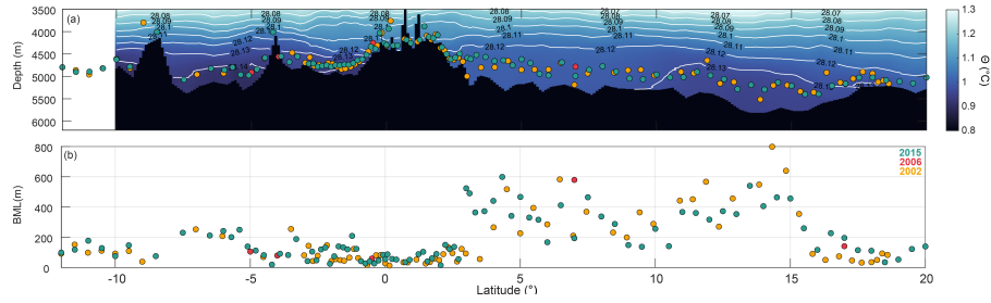
Figure 5. The P16 repeat hydrographic line nominally along 150^{\circ} W with (a) conservative temperature ( \Theta ) with neutral density ( \gamma_n ) as the white contours and the BML thickness for 2015 (green), 2006 (red), and 2002 (orange). Note the seafloor, \Theta and \gamma_n are from the gridded data product available from Katsumata et al. (2022) and therefore may not be an exact representation of the seafloor depth, (b) BML thickness above the seafloor with color representation as in (a).
