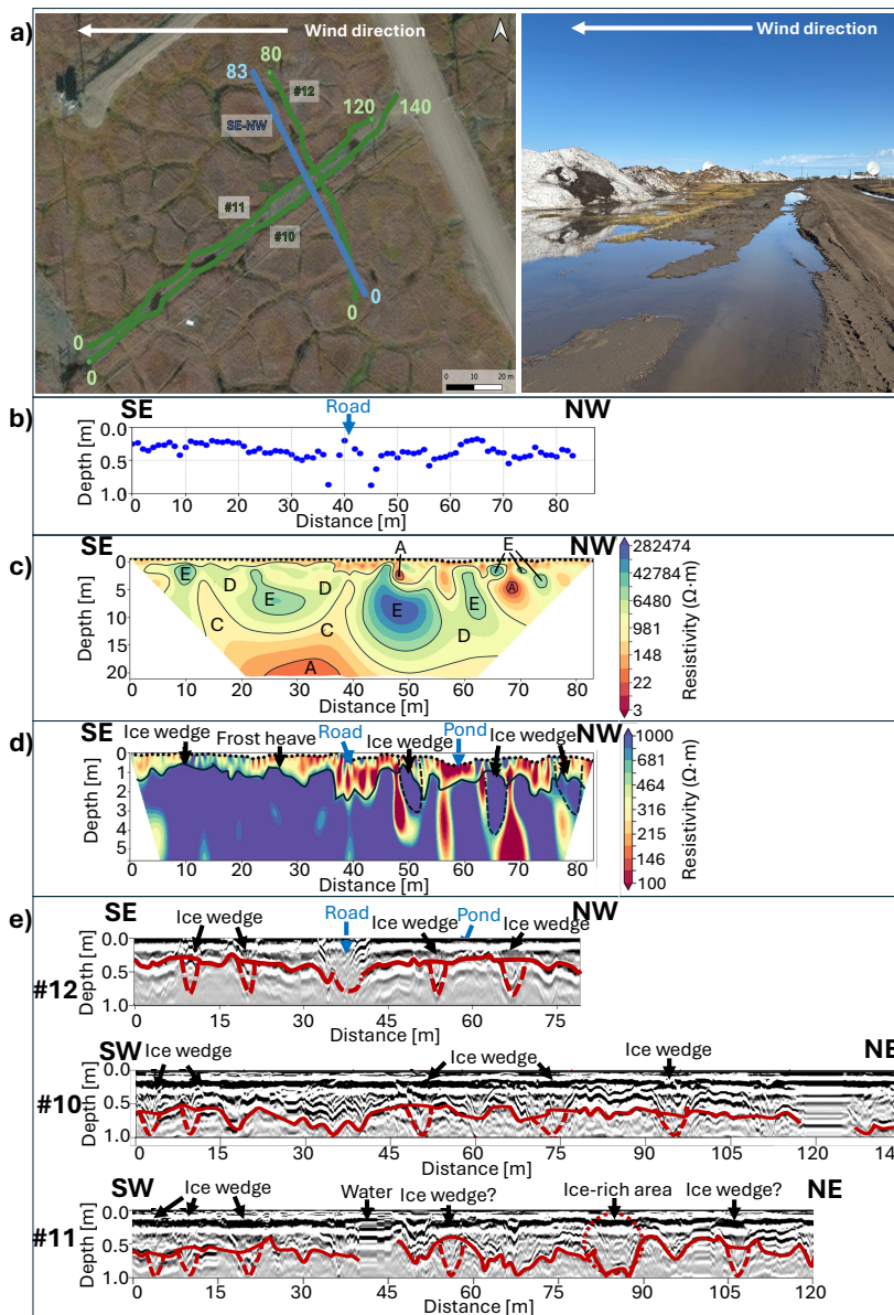
Figure 4: (a) Left - Location of ERT (blue, SE–NW) and GPR (green) profiles near the old section of Cakeeater Road, shown on 300 ESRI satellite imagery, © ESRI (QGIS). Right – Photo of the similar site with snow accumulation and melt water ponding along the Imaiqaun Road (photo by Valentina Ekimova, May 2025); (b) Thaw probe measurements along the ERT profile and GPR profile #12; (c) Coarse-scale SE–NW ERT resistivity cross-section (~0–20 m depth), with black dots indicating electrode positions and zones A–E denoting approximate permafrost features based on resistivity values; (d) Fine-scale SE–NW ERT profile (~top 5.7 m), showing thaw depth variability; (e) GPR profiles: #12 (aligned with the ERT transect) shows thaw depths (red line) and 305 hyperbolic reflections interpreted as ice wedges (red dashed lines), while profiles #10 and #11 (parallel to the road) show similar features, with #11 also indicating a possible ice-rich zone (red dashed circle).
