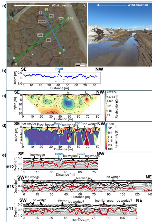
Figure 4: (a) Left - Location of ERT (blue, SE–NW) and GPR (green) profiles near the old section of Cakeeater Road, shown on ESRI satellite imagery (QGIS). Right – Photo of the similar site with snow accumulation and melt water ponding along the Imaigsau Road (photo by Valentina Ekimova, May 2025); (b) Thaw probe measurements along the ERT profile and GPR profile #12; (c) Coarse-scale SE–NW ERT resistivity cross-section (~0–20 m depth), with black dots indicating electrode positions and zones A–E denoting approximate permafrost features based on resistivity values; (d) Fine-scale SE–NW ERT profile (~top 5.7 m), showing thaw depth variability; (e) GPR profiles: #12 (aligned with the ERT transect) shows thaw depths (red line) and hyperbolic reflections interpreted as ice wedges (red dashed lines), while profiles #10 and #11 (parallel to the road) show similar features, with #11 also indicating a possible ice-rich zone (red dashed circle).
