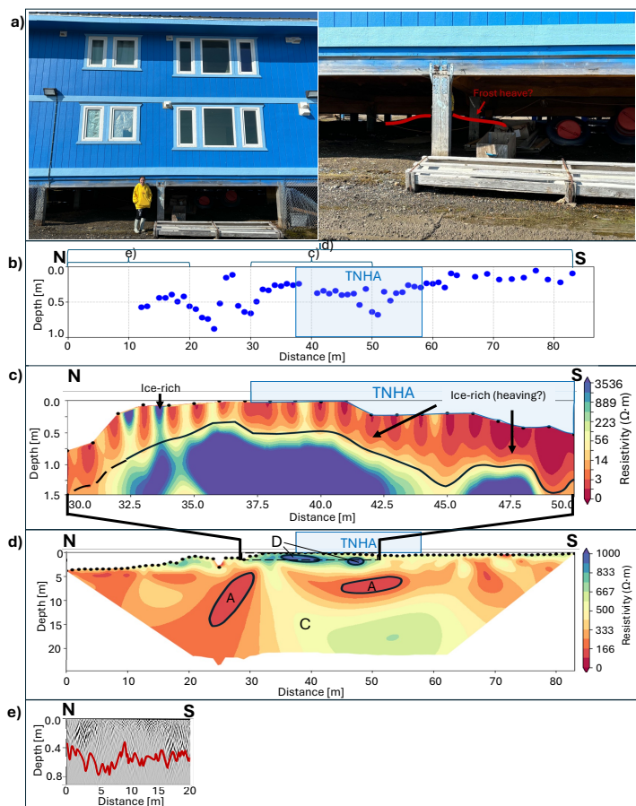
250 Figure 3: (a) Left – Photograph of the TNH building (June 2024). Photo: MacKenzie Nelson. Right – Surface elevation beneath the building at the TNH site, outlined by the red line, indicating possible frost heave features (28 June 2024); (b) Thaw probe measurements along the N–S ERT transect at the TNH site; (c) Small-scale view of the upper 3 m between 30–50 m profile distance, including the building footprint, with thaw depth indicated by solid black line; (d) N–S coarse-scale resistivity cross- section (–0–15 m depth), showing approximate interpretive zones A–D; A – cryopegs (0.5–10 \Omega\cdot m ), C – transition zone (400– 1,000 \Omega\cdot m ), D – ice-rich permafrost (>1,000 \Omega\cdot m ); (e) N–S GPR profile, showing thaw depths (red line). Elevation shown in meters above sea level.
