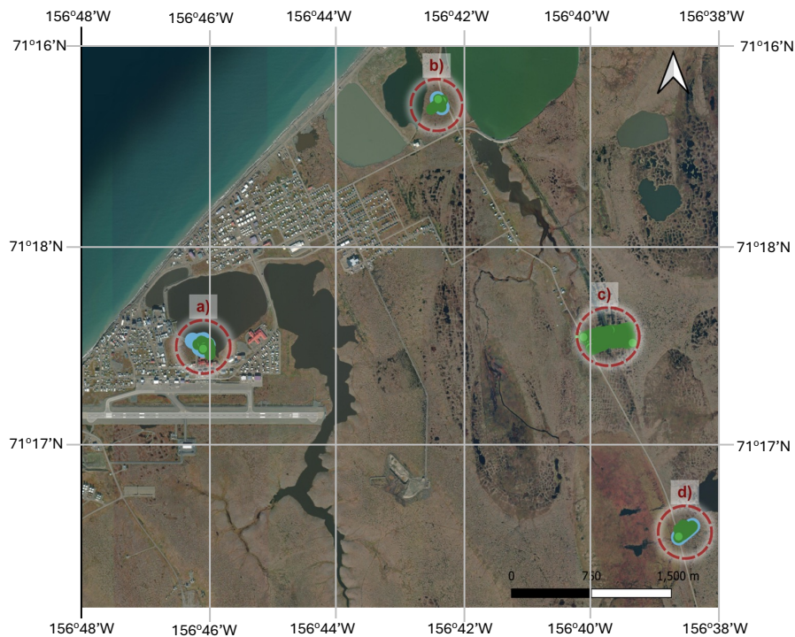
Figure 1: Location of geophysical survey (ERT - blue dots, GPR - green dots) sites in Utqiagvik, Alaska, shown on ESRI satellite imagery in QGIS. Sites include (a) the Tagiugmiullu Nunamiullu Housing Authority (TNHA) residential facility, (b) the old section of Cakeeater Road, (c) a snow fence location near Cakeeater Road, and (d) the Barrow Environmental Observatory (BEO).
