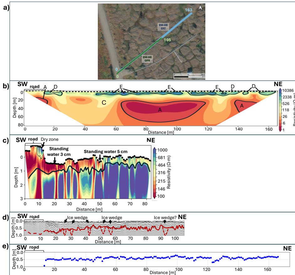
Figure 6: (a) Location of SW-NE ERT (blue) and GPR (green) profiles at the BEO site in Utqiagvik, Alaska (ESRI satellite imagery); (b) Coarse-scale view of the SW-NE ERT profile; (c) Fine-scale view of the SW-NE ERT profile; (d) SW-NE GPR profile showing thaw depths (solid red line) and hyperbolic reflections was interpreted as ice wedges (red dashed lines); (e) Thaw probe measurements along the ERT profile.
