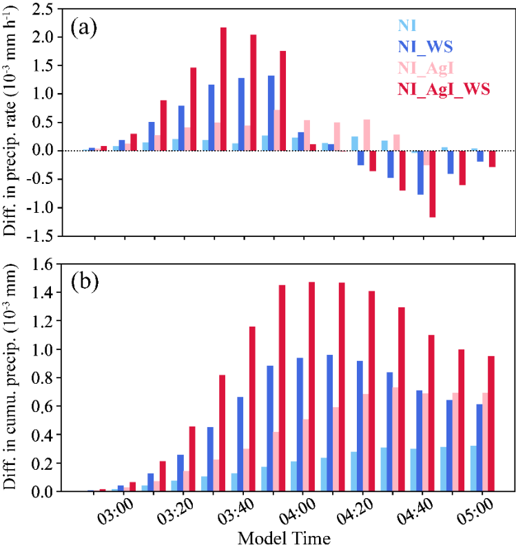
335 Figure 10. Temporal variations of the differences in (a) precipitation rates and (b) cumulative precipitation between SEED and NOSEED areas.
