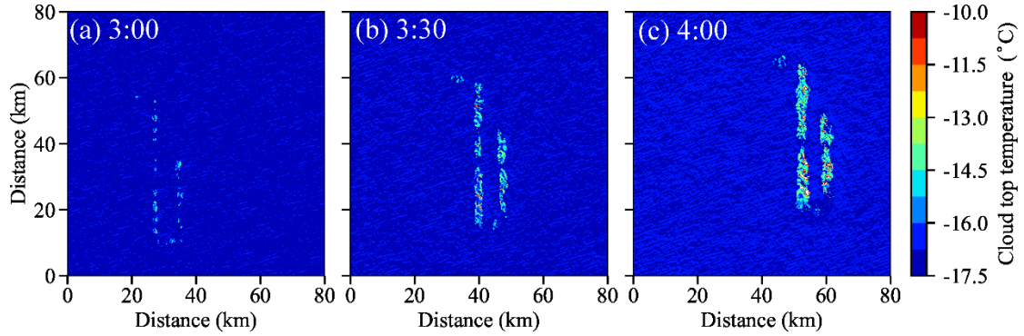
250 Figure 6. Maps of cloud top temperature in the Control experiment from 03:00 to 04:00 Model Time.
