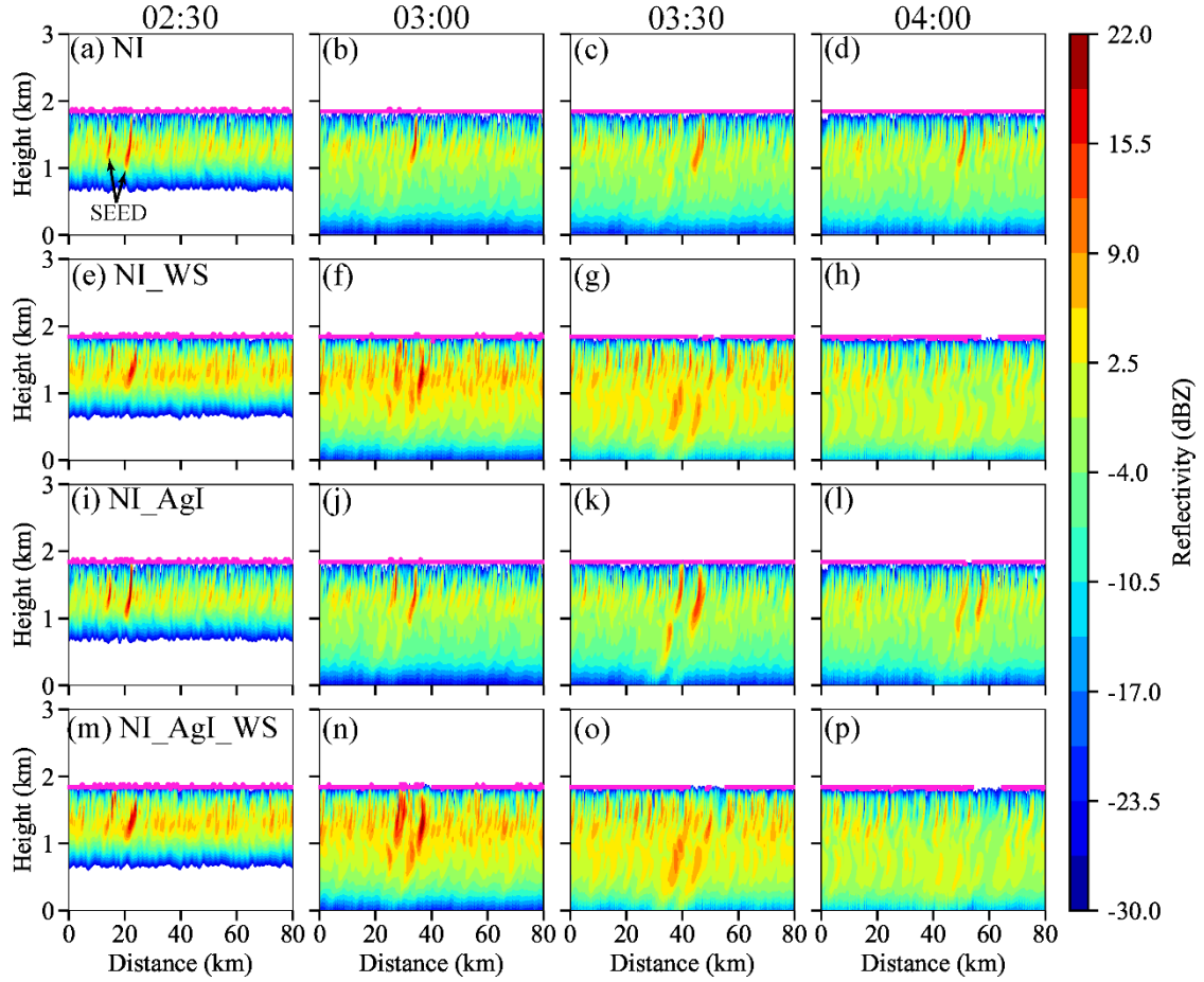
Figure 7. East-west cross-sections of reflectivity from (a-d) NI, (e-h) NI_WS, (i-l) NI_AgI, and (m-p) NI_AgI_WS experiments from 02:30 to 04:00 Model Time. The magenta lines indicate the top of the liquid layer. Natural ice nucleation is allowed in the simulations. The cross-sections are selected at y = 20 km, y = 20 km, y = 40 km, and y = 50 km at 02:30, 03:00, 03:30, and 04:00 MT, respectively.
