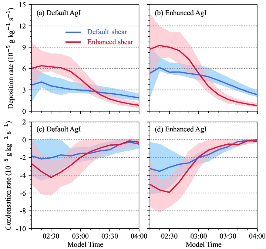
315 Figure 9. Temporal variations of (a, b) ice depositional growth rate and (c, d) droplet condensation rate in SEED areas at different AgI concentrations and shear intensities. The upper and lower boundaries of the shaded areas indicate the 75 th and 25 th percentiles and the solid lines represent the mean values.
