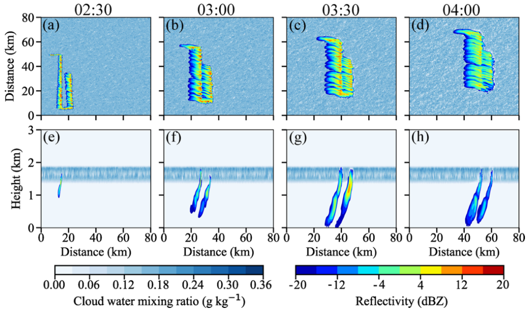
245 Figure 5. (a-d) Maps of composite reflectivity and cloud water mixing ratio from the Control experiment at seeding height from 02:30 to 04:00 Model Time. (e-h) Cross-sections of reflectivity and cloud water mixing ratios from the Control experiment along y = 40 km from 02:30 to 04:00 Model Time.
