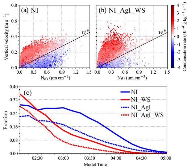
Figure 13. Condensation rates in SEED areas under different vertical velocities and N_l r_l from (a) NI and (b) NI_AgI_WS experiments at 03:30 MT. The black lines are the minimum vertical velocity for which both liquid and ice can grow, which are calculated using Eq. 3 at 700 hPa and -15^\circ\text{C} . (c) The fraction of area with positive condensation rate in SEED areas.
