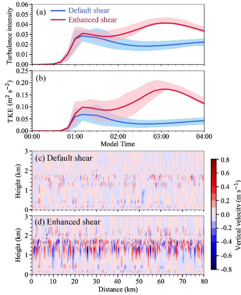
220 Figure 4. Temporal variations of turbulence intensity (a) and TKE (b) from the simulations with default and enhanced wind shear. The upper and lower boundaries of the shaded areas respectively indicate the 75 th and 25 th percentiles, and the solid lines indicate the mean values. (c) and (d) are the cross-sections of vertical velocity at 03:00 Model Time from the simulations with default and enhanced wind shear, respectively.
