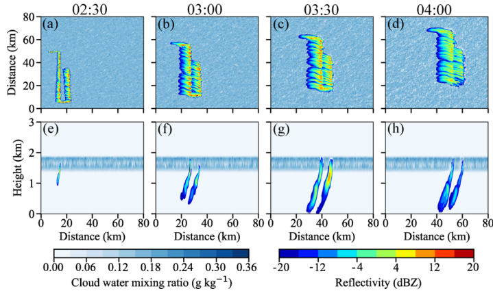
Figure 5. (a-d) Maps of composite reflectivity and cloud water mixing ratio from the Control experiment at seeding height from 02:30 to 04:00 Model Time. (e-h) Cross-sections of reflectivity and cloud water mixing ratios from the Control experiment along y = 40 km from 02:30 to 04:00 Model Time.
