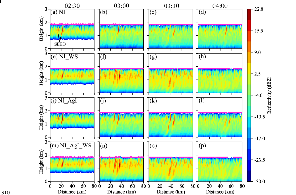
Figure 7. East-west cross-sections of reflectivity from (a-d) NI, (e-h) NI_WS, (i-l) NI_AgI, and (m-p) NI_AgI_WS experiments from 02:30 to 04:00 Model Time. The magenta lines indicate the top of the liquid layer. Natural ice nucleation is allowed in the simulations. The cross-sections are selected at y = 20 km, y = 20 km, y = 40 km, and y = 50 km at 02:30, 03:00, 03:30, and 04:00 MT, respectively.
