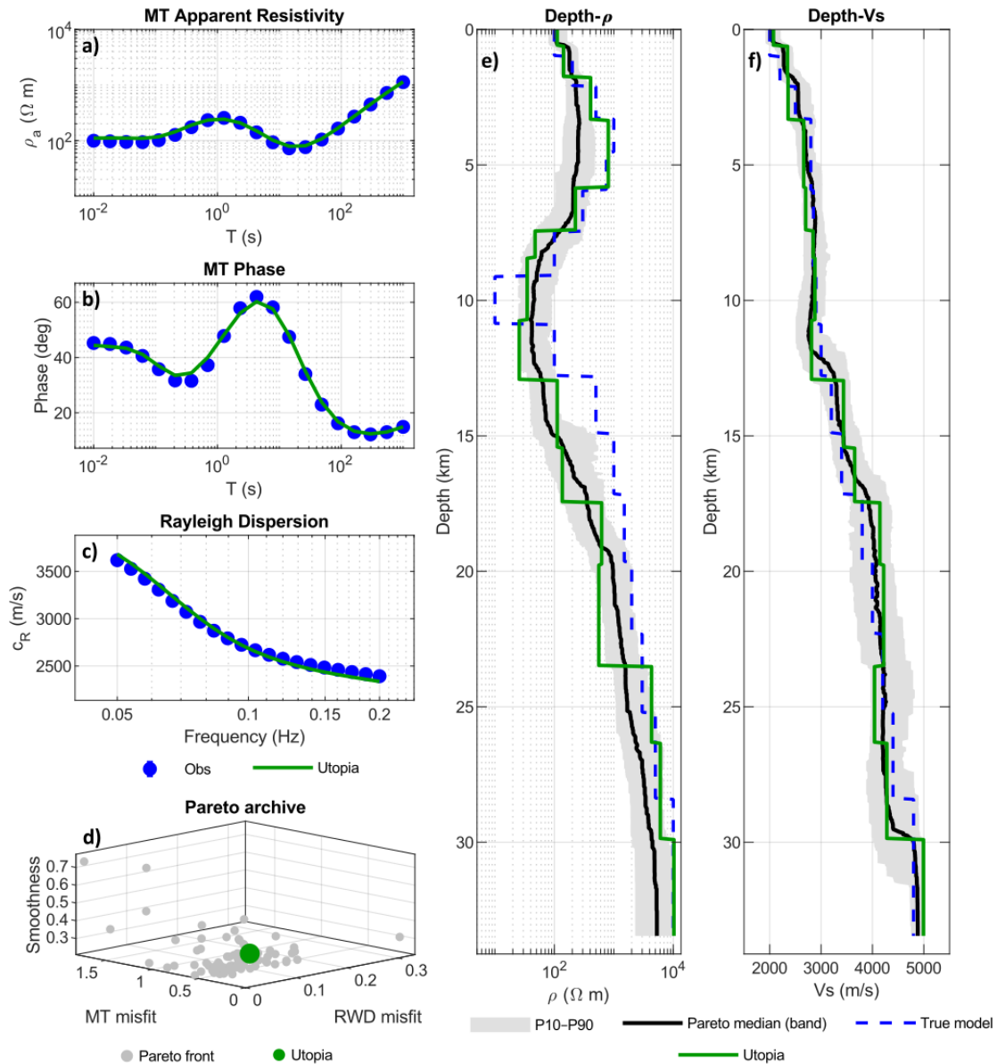
Figure 12: Results of the noise-free decoupled case#1. a) Apparent resistivity and b) Phase data and c) RWD fit with the predicted responses of the utopia solution. d) Three-objective Pareto archive, highlighting the utopia solution. e) \rho(z) and f) V_s(z) models for the true model and the selected utopia solution, together with the P10–P90 envelope and the Pareto-median profile from the repository.
