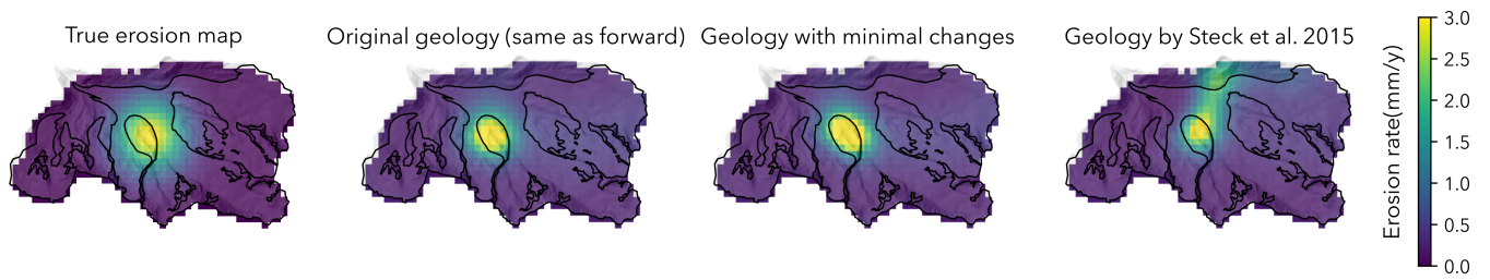
Figure B1. Scenario 1: geological map uncertainty and its impact on posterior erosion rate maps.
