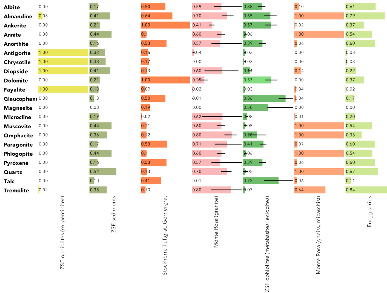
Figure 11. Normalised FDD XRD-based mineralogical fingerprints of the different source areas of the Gornergletscher catchment. From left to right: ZSF ophiolites (serpentinites), ZSF sediments, Stockhorn-Tuffgrat-Gornergrat, Monte Rosa (granite), ZSF ophiolites (metabasites, eclogites), Monte Rosa (gneiss, micaschist), Furgg series. Errorbars indicate the variability of the mineralogical signal between different samples for the same lithological unit. FDD
