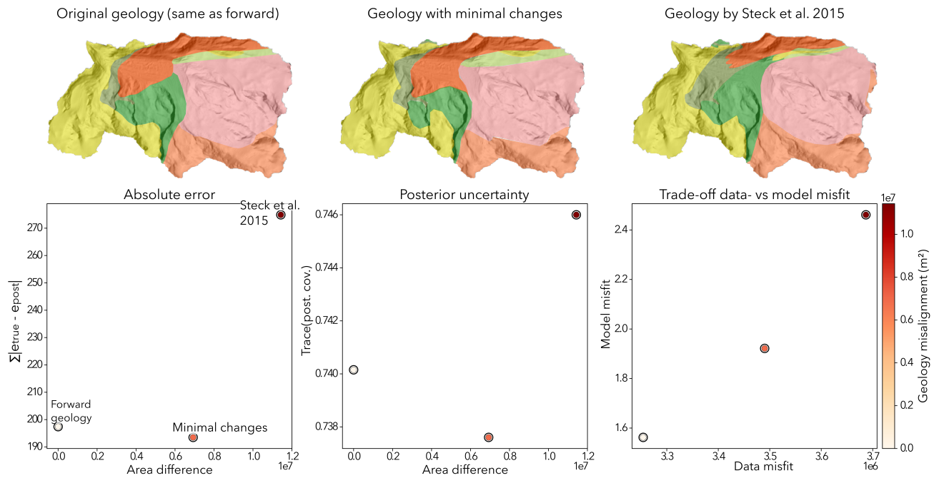
Figure 7. Scenario 1: geological map uncertainty (the colour on the scatterplot indicates area difference (m 2 ) between the lithological map used to generate the synthetic data and the one used in the inversion). In the left scatterplot, the labels correspond to the maps above.
