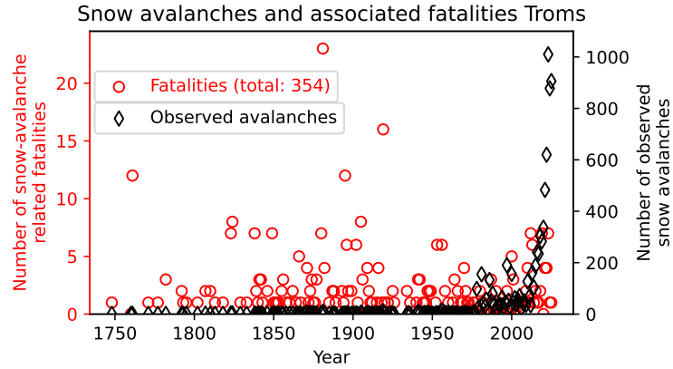
Figure 1. Time series of (red) snow-avalanche related fatalities and (blackred) and observed snow avalanches (black) in Troms county, Norway. The data are provided by the Norwegian Water Resources and Energy Directorate (NVE) and can be downloaded from https://nedlasting.nve.no/gis/ (last access 29-January 5 August 2025).
