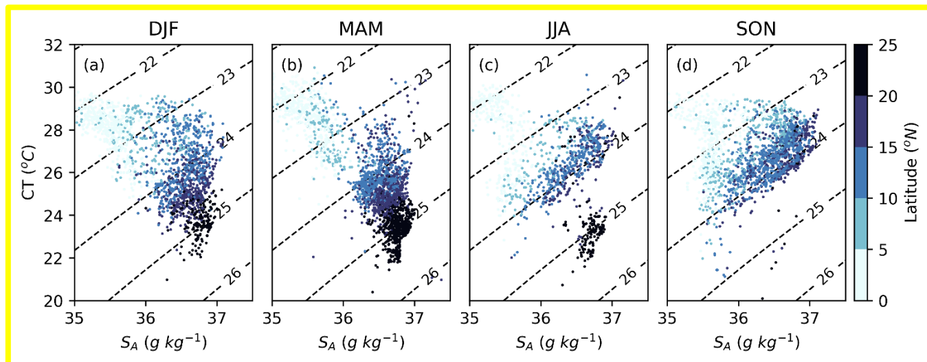
Figure 2. Mode Water seasonal and spatial variability. Mode water core T-S diagram from all available float profiles in the Arabian Sea for (a) winter (DJF, December-January-February), (b) spring (MAM, March-April-May), (c) summer (JJA, June-July-August), and (d) fall (SON, September-October-November) colored by latitude. Isopycnals (dashed black) are shown for all panels.
