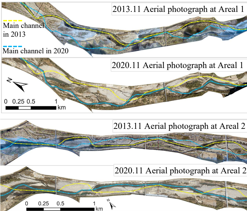
85 Figure 1: An outline of the study area. (a) and (b) show the location of the target site in Japan (Esri, HERE, Garmin, FAO, NOAA, USGS) and the watershed (Digital Elevation Model (DEM) from the Geospatial Information (GSI) Authority of Japan), respectively; (c) shows the morphology (DEM from the GSI) of the target site; and (d) provide orthophotos from 2013 and 2020 (Copyright © Ministry of Land, Infrastructure, Transport and Tourism (MLIT) in Japan), respectively.
