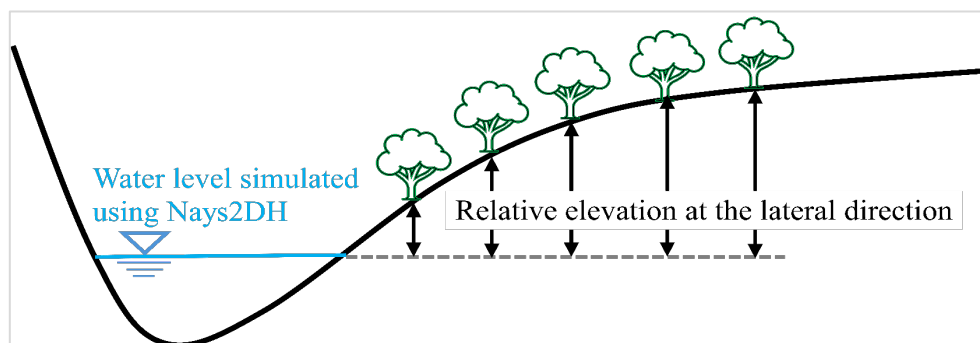
Figure 6: Conceptual diagram of relative elevation in the lateral direction.
