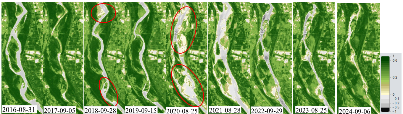
Figure 7: NDVI from 2016 to 2024 at the representative Area 1 (the vegetation mortality area after the largest flood and second-largest flood was marked with red polygon).
