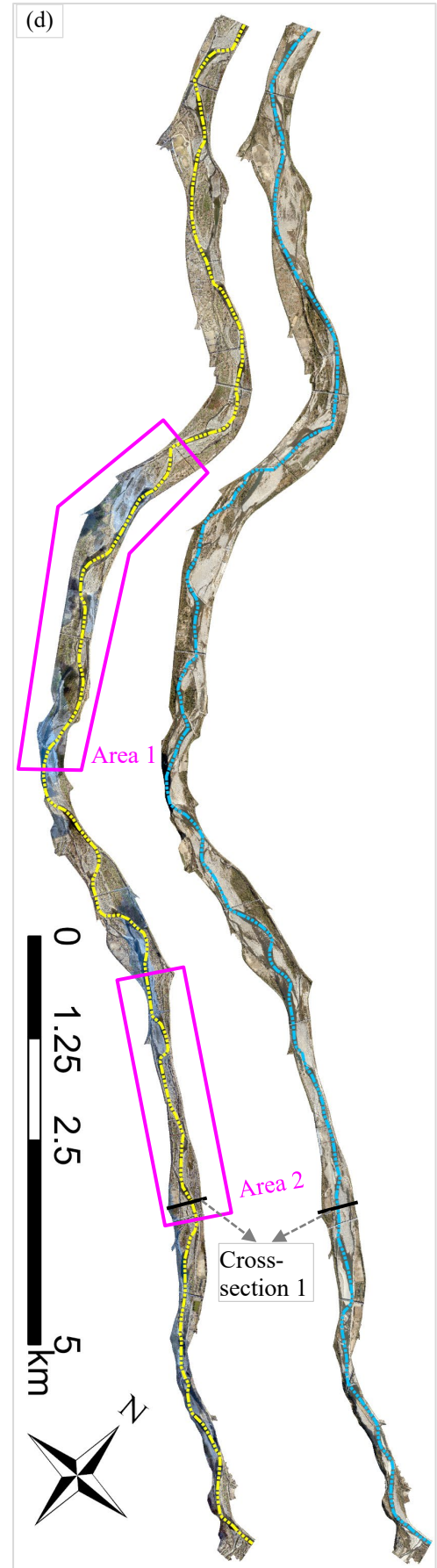
85 Figure 1: An outline of the study area. (a) and (b) show the location of the target site in Japan (Esri, HERE, Garmin, FAO, NOAA, USGS) and the watershed (Digital Elevation Model (DEM) from the Geospatial Information (GSI) Authority of Japan), respectively; (c) shows the morphology (DEM from the GSI) of the target site; and (d) provide orthophotos from 2013 and 2020 (Copyright © Ministry of Land, Infrastructure, Transport and Tourism (MLIT) in Japan), respectively.
