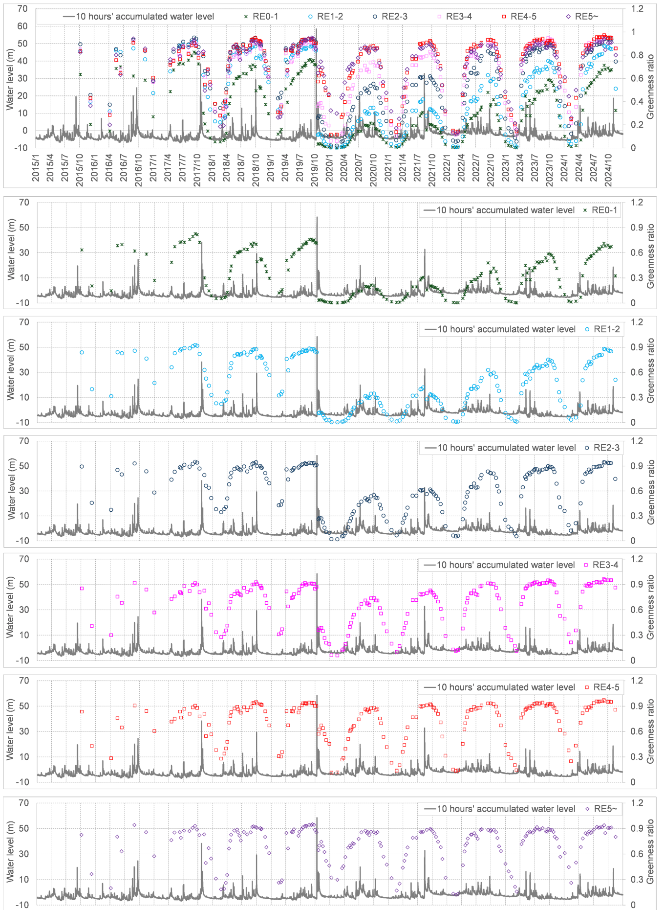
Figure 8: Spatiotemporal vegetation greenness and hydro-morphological dynamics (RE0-1, RE1-2, RE2-3, RE3-4, RE4-5, and RE5~ denote relative elevation classes of 0–1 m, 1–2 m, 2–3 m, 3–4 m, 4–5 m, and \geq 5 m, respectively. “10-hour accumulated water level” refers to the water level accumulated over a 10-hour period).
