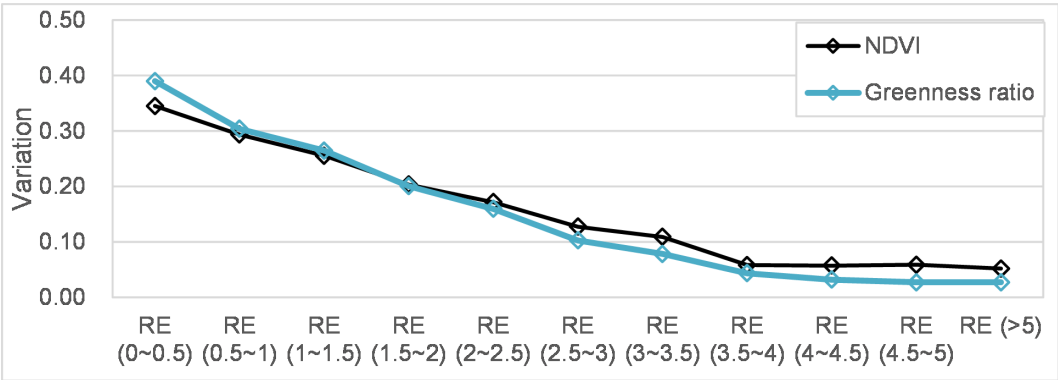
Figure 14: Averaged variation of NDVI and greenness ratio from 2016 to 2024.
