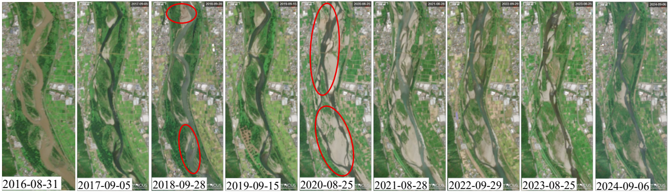
Figure 2: Sentinel-2 imagery from 2016 to 2024 at representative Area 1
