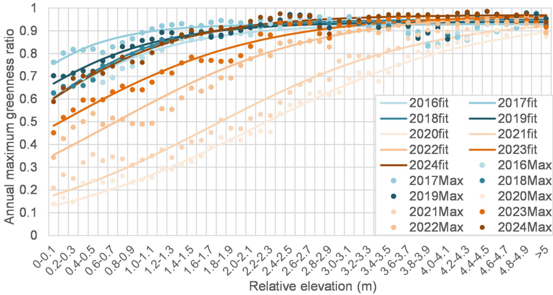
Figure 9: Annual maximum greenness ratio along the transect.
