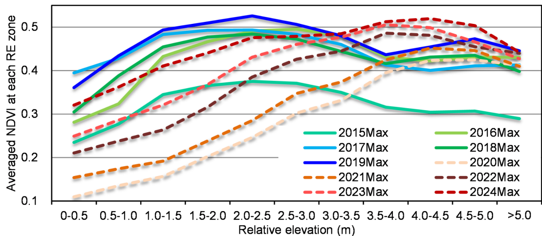
Figure 10: Annual maximum NDVI averaged within each 0.5m relative elevation zone along the transect.
