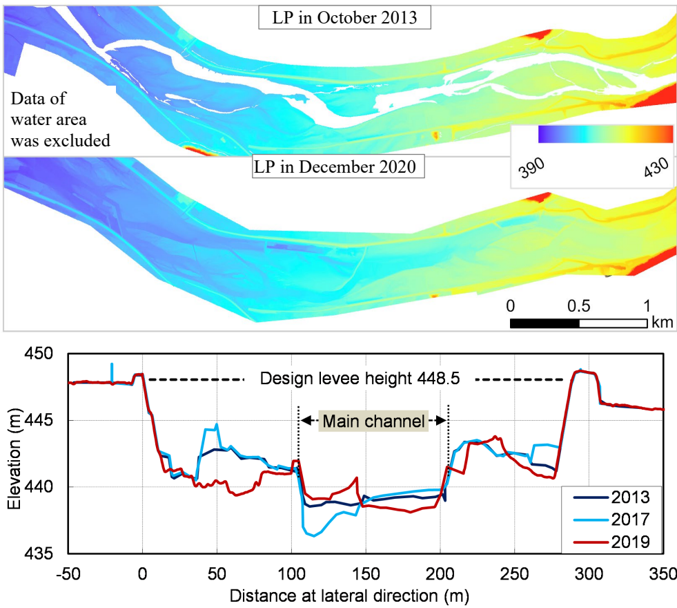
Figure 4: LP survey data at representative Area 1 and one cross-sectional profile of morphology at Cross-section 1.
