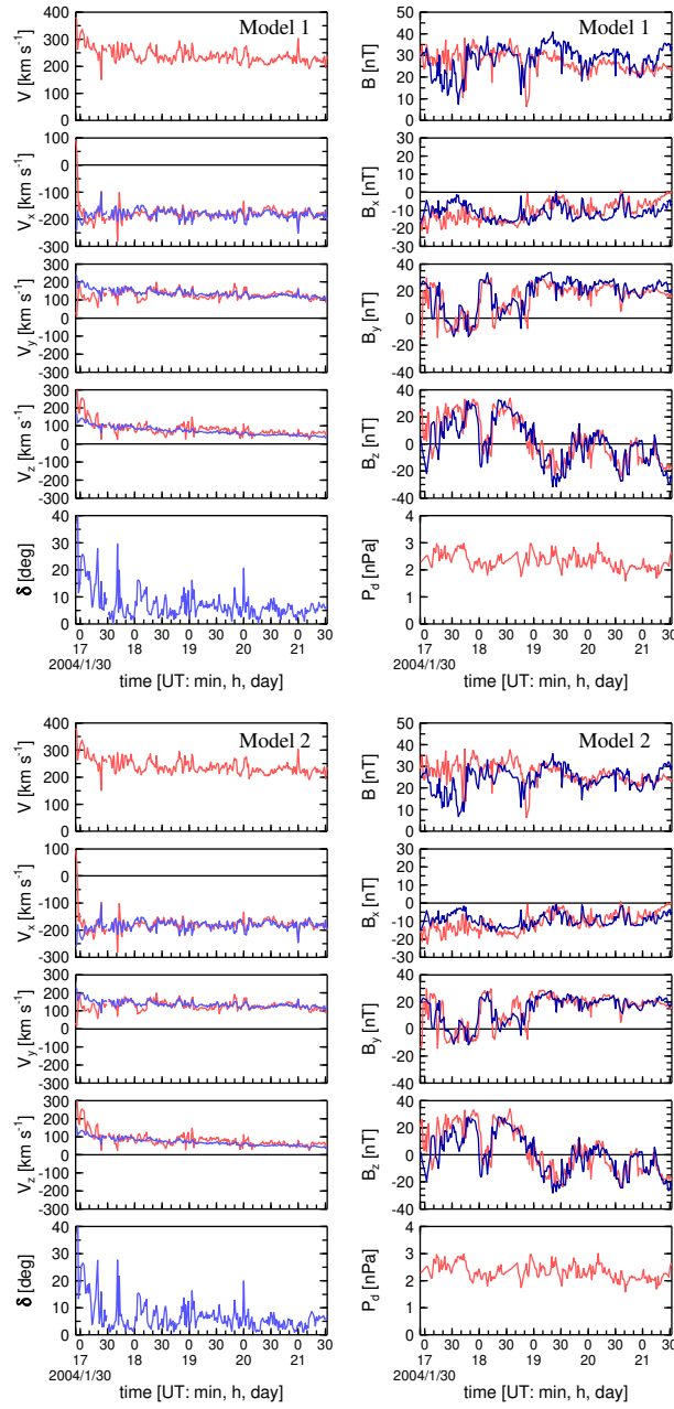
Figure 1. Observed (red lines) and modeled (blue lines) quantities for the passage through the Earth's MSH in case 7. Left panels: from top the velocity magnitude V , GSE velocity components V_x , V_y , and V_z , and the angle \delta between the observed and modeled velocity vectors; right panels: from top the magnetic field magnitude B , GSE magnetic field components B_x , B_y , and B_z , and upstream dynamic pressure P_d . Upper panels are for Model 1, bottom panels for Model 2. The left-hand-side panel model velocity components (light blue) are proxy values, created using an artificial radial upstream magnetic field, while the model MSH magnetic field components on the right-hand-side panels (dark blue) use the actual upstream IMF observations.
