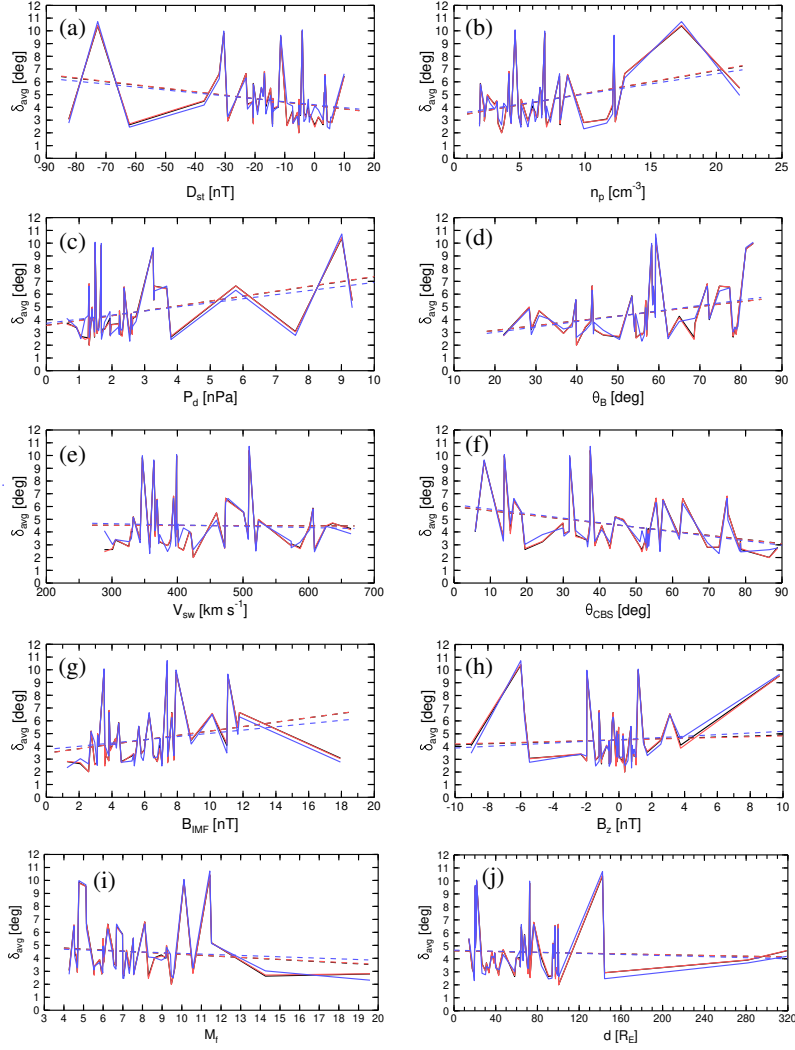
Figure 6. Dependencies of \delta_{\text{avg}} on various quantities. The details are given in the text. Model 1 is drawn in the black lines, Model 2 in the red lines, and Model 3 in the blue lines.
