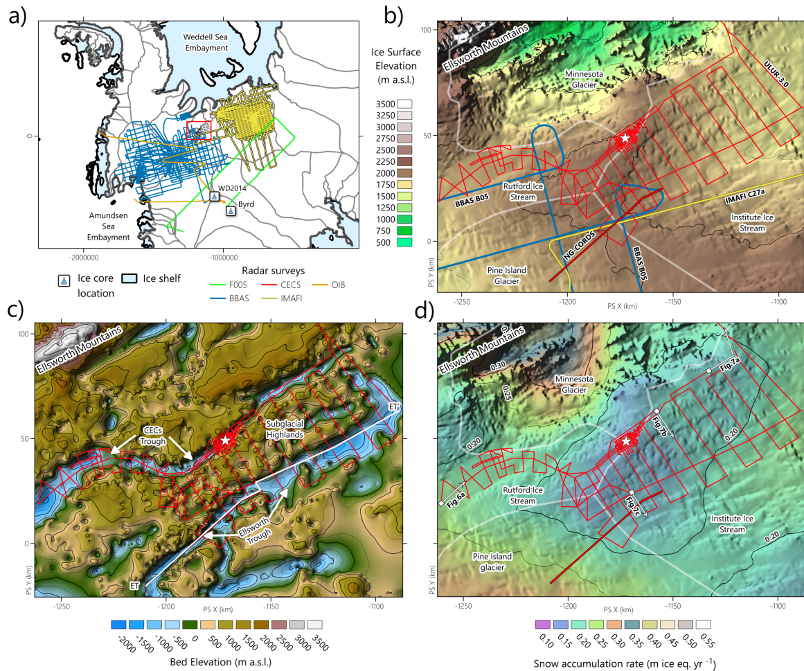
Figure 1. (a) Location of the Ellsworth Subglacial Highlands (ESH) relative to the West Antarctic Ice Sheet (WAIS) and the radio-echo sounding (RES) surveys used in this study. The red box outlines the area shown in panels (b), (c), and (d). Coloured lines indicate different RES campaigns: BBAS in blue (Corr et al., 2021), IMAFI in yellow (Ross et al., 2021), and CECS in red. These campaigns were used to extend the radiostratigraphy from two dated ice cores: Byrd and WAIS Divide (WAISD-2014). (b) Ice surface elevation from BedMachine Antarctica v3 (Morlighem et al., 2020), overlain on the Radarsat Antarctic Mapping Project (RAMP) mosaic (Liu et al., 2015) with black contour lines indicating elevation isolines every 250 m. Coloured lines show the different RES surveys and their intersection along the ice divide between Pine Island Glacier and Institute Ice Stream, as well as in Rutford Ice Stream. (c) CECS RES survey lines across the ESH, shown over basal topography from Napoleoni et al. (2020). Locations of main topographic features are indicated, and RES control lines ET and ET' (see Figure 2a) are also highlighted. (d) Snow accumulation rates derived from statistically downscaled regional climate model output (27 km to 2 km resolution; Noël et al. 2023), overlain on RAMP imagery with black contour lines indicating accumulation isolines every 0.05 m ice eq. yr -1 . The locations of profiles shown in Figure 6 and Figure 7 are also indicated by white segments with corresponding labels. All panels: White lines denote ice catchment boundaries from the MEaSUREs dataset (Mouginot et al., 2017), and a white star indicates the location of Subglacial Lake CECs (SLC).
