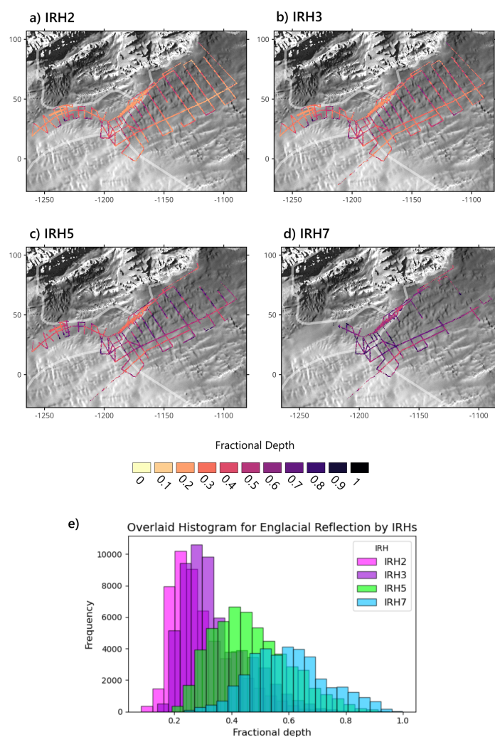
Figure B2. Spatial distribution and fractional depth histograms of internal reflecting horizons (IRHs). Panels (a–d) show mapped IRHs across the Ellsworth Subglacial Highlands, overlaid on Radarsat Antarctic Mapping Project (RAMP) topography. Thin white lines delineate the ice catchment boundaries (Mouginot et al., 2017). Colours denote fractional depth within the ice column, ranging from 0 (surface; yellow) to 1 (bed; black). (a) IRH2, (b) IRH3, (c) IRH5, and (d) IRH7. Panel (e) presents overlaid histograms of fractional depths for each IRH. The shallower horizons (IRH2, IRH3) cluster at fractional depths of 0.15–0.35, whereas deeper horizons (IRH5, IRH7) extend more evenly through the ice column, with IRH7 reaching depths approaching the bed.
