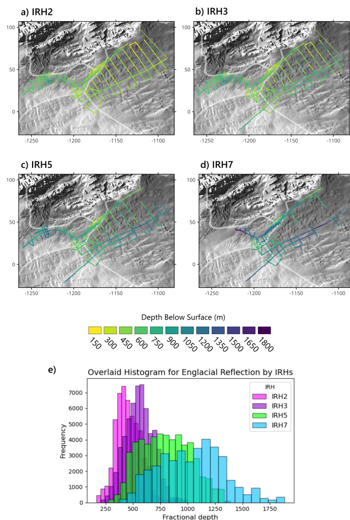
Figure B1. Spatial distribution and depth histograms of internal reflecting horizons (IRHs). Panels (a–d) show mapped IRHs across the Ellsworth Subglacial Highlands, overlaid on Radarsat Antarctic Mapping Project (RAMP) topography. Thin white lines delineate the ice catchment boundaries (Mouginot et al., 2017). Each colour corresponds to depth below the ice surface, ranging from 150 m (yellow) to 1800 m (dark purple). (a) IRH2, (b) IRH3, (c) IRH5, and (d) IRH7. Panel (e) displays overlaid histograms of fractional depths for each IRH, illustrating their relative depth distributions. Shallower horizons (IRH2, IRH3) are concentrated between 250–700 m, while deeper horizons (IRH5, IRH7) extend to >1500 m.
