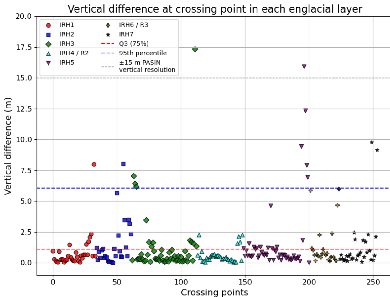
Figure 8. Vertical difference between crossovers of CECs Internal Reflection Horizon (IRH). Differences among IRH depth are presented for each IRHs in different colour and shape from the shallowest (IRH1) to the deepest one (IRH7). Additionally, we also marked the vertical resolution calculated for PASIN1 (Bodart et al., 2021) and key statistical percentiles.
