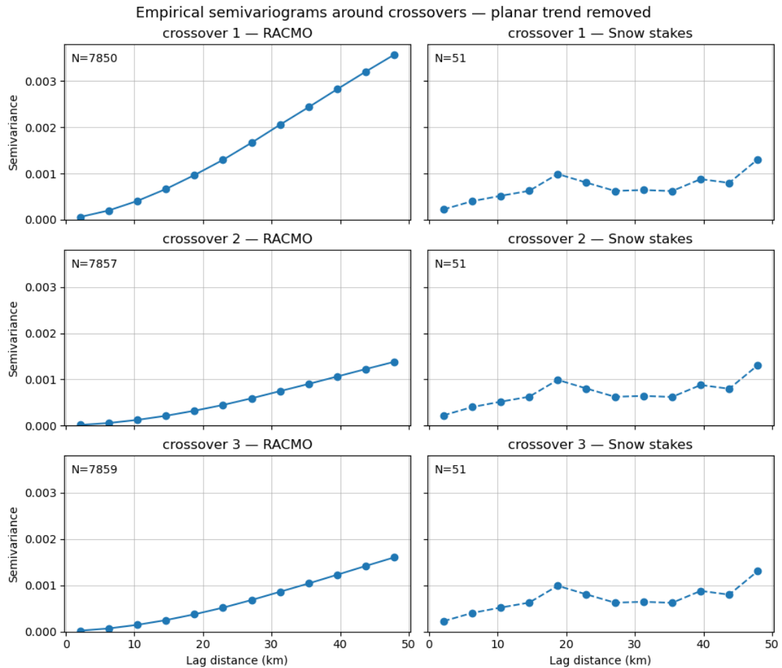
Figure B4. Empirical semivariograms of annual mean surface accumulation around three crossover locations, calculated after removal of a planar trend. Left panels show RACMO2.3p2 estimates and right panels show snow-stake measurements. Stake-derived accumulation exhibits stronger short-range variability (~15–20 km), whereas RACMO2.3p2 displays smoother spatial structure over longer length scales. Numbers indicate the number of data pairs contributing to each semivariogram.
