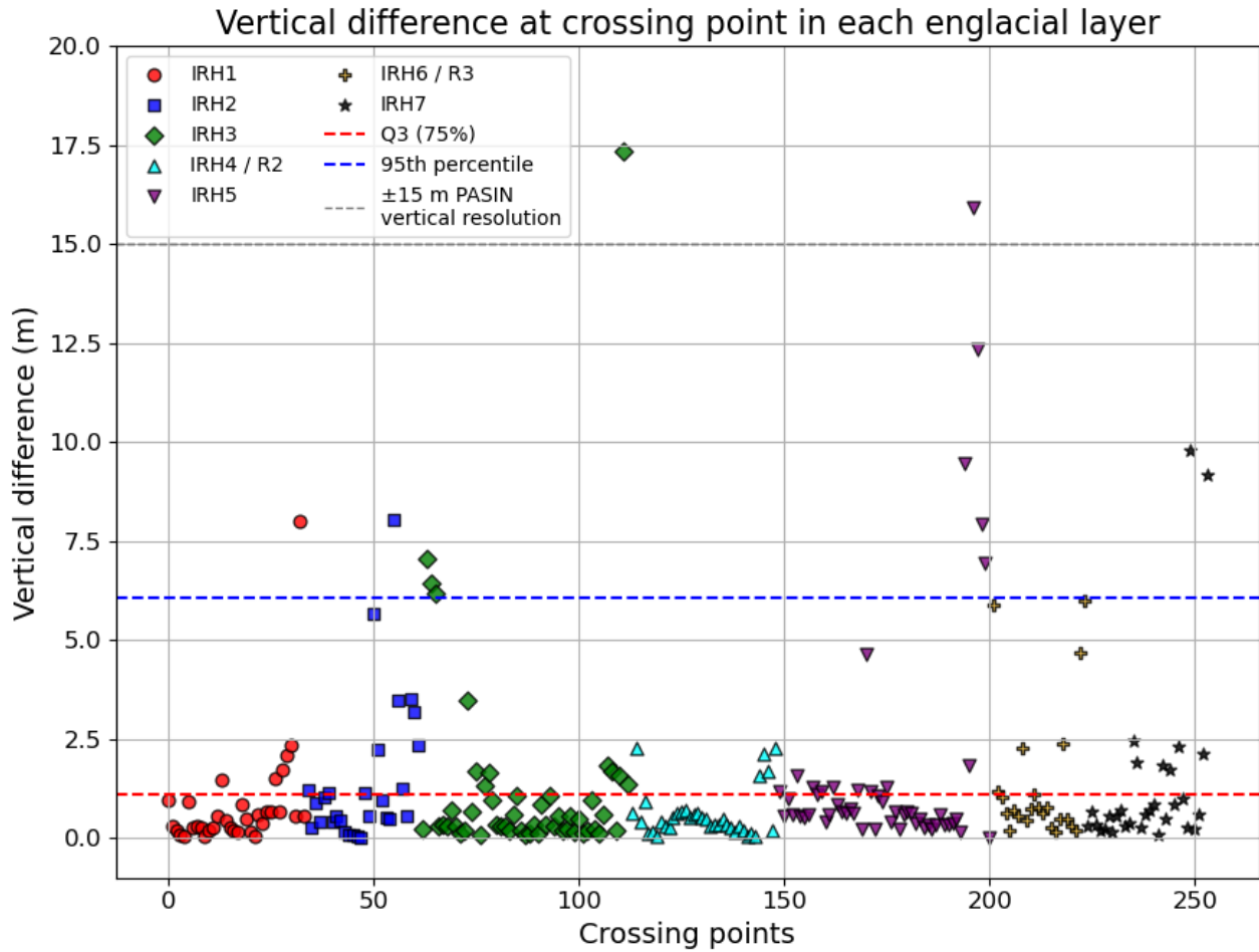
Figure B3. Vertical difference between crossovers of CECs Internal Reflection Horizon (IRH). Differences among IRH depth are presented for each IRHs in different colour and shape from the shallowest (IRH1) to the deepest one (IRH7). Additionally, we also marked the vertical resolution calculated for PASINI (Bodart et al., 2021) and key statistical percentiles.
