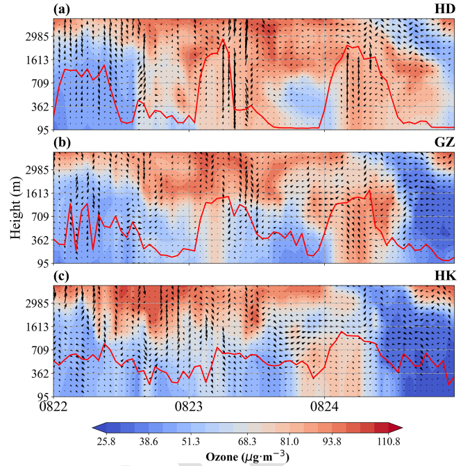
Figure 11. The figure displays time series of the simulated ozone and wind profile between 00:00 LT on 22 August and 00:00 LT on 25 August at three sites (Huadu, Guangzhou and Hong Kong). The vertical wind speed has been amplified by a factor of 10 to enhance clarity. In the figure, the red line indicates the height of the boundary layer.
