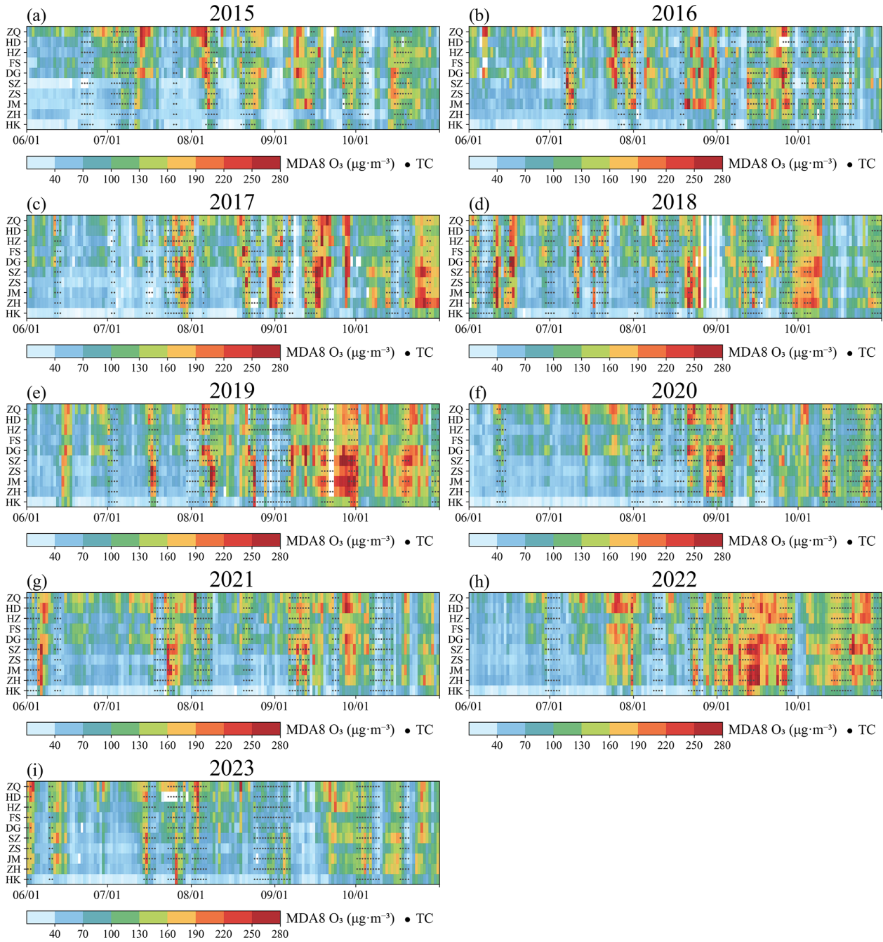
Figure 3. The maximum daily 8 h average (MDA8) O 3 in 10 cities in the GBA in (a) 2015, (b) 2016, (c) 2017, (d) 2018, (e) 2019, (f) 2020, (g) 2021, (h) 2022, and (i) 2023 from June to October. The national standard for ambient air quality for MDA8 O 3 is 160\mu\text{g}\cdot\text{m}^{-3} in China. These cities are sorted by latitude. The black dots represent the days of TC, where the TC track enters (10–30° N, 100–130° E).
