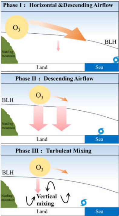
Figure J5. A schematic diagram illustrating the dynamic response of airflow and O 3 within the height of the boundary layer height (BLH) of the GBA to the approaching tropical cyclone (TC). (a) Phase I: Horizontal & Downdraft Control - The pink arrows represent the downdraft airflow from the periphery of the TC, the orange arrows indicate the
