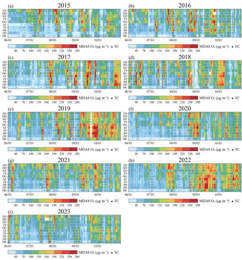
Figure 3. The maximum daily 8-hour average (MDA8) O 3 in 10 cities in the GBA in (a) 2015, (b) 2016, (c) 2017, (d) 2018, (e) 2019, (f) 2020, (g) 2021, (h) 2022, and (i) 2023 from June to October. The national standard for ambient air quality for MDA8 O 3 is 160 μg m -3 in China. These cities are sorted by latitude. The black dots represent the days of TC, where the TC track enters (10°N-30°N, 100°E-130°E).
