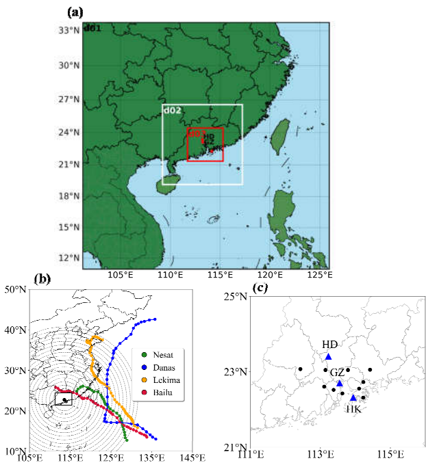
Figure 1. (a) the simulation domain is illustrated, with three monitoring sites annotated: Huadu (23.4°N, 113.2°E), Guangzhou (22.7°N, 113.5°E) and Hong Kong (22.3°N, 114.2°E). These locations are strategically positioned to capture spatial variations within the study area. (b) Tropical Cyclone Nesat, Lekima, Danas, Bailu. The gray dashed circles are centered on the wind profiler radar in the middle of the GBA at GZ (black dot; 22.7°N, 113.55°E), representing distances of 300-2000 km from the GBA, with intervals of 100 km between concentric circles. (c) Locations of the HD, GZ, and HK stations in the GBA. The black box indicates the location of the GBA. The black dots indicate the locations of the 10 cities shown in Figure 3.
