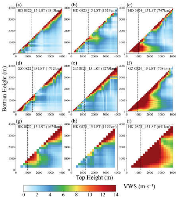
455 | Figure 13. Vertical Wind Shear (VWS) from 22 to 24 August at (a-c) HD station, (d-f) GZ station, and (g-i) HK station. The black dashed line represents the height of the boundary layer. The distance in character brackets at the top left of the subplot indicated the distance from TC Bailu to the wind profile radars at that moment.
