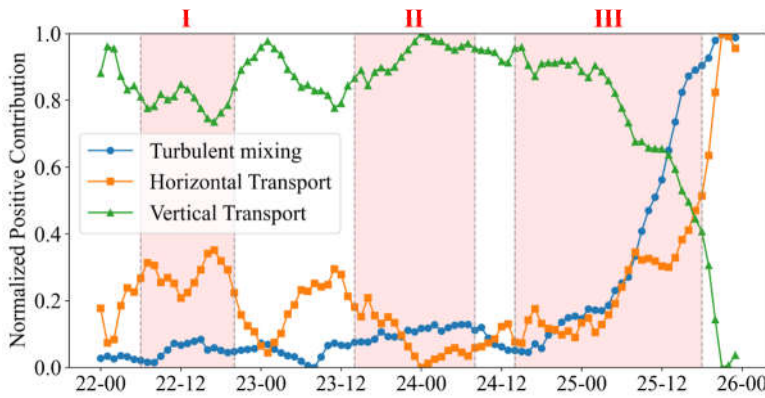
Figure 14. This normalized time series shows the contributions of three dynamical processes (horizontal transport, vertical transport, and turbulent mixing) to ozone pollution in the Pearl River Delta region. The dashed lines divide the processes into three distinct periods: a period dominated by horizontal and descending transport (Period I), a period with enhanced descending transport (Period II), and a period characterized by increased turbulent mixing (Period III).
