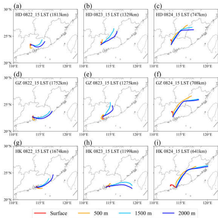
Figure 8. 24-hour backward trajectories of (a-c) HD station, (d-f) GZ station, and (g-i) HK station at different vertical heights. (Heights of 0, 500, 1500, and 2000 m represent the surface, the middle of the boundary layer, the top of the boundary layer, and above the boundary layer, respectively. The distance in the character brackets on the top left of the subplot indicated the distance from TC Bailu to the wind profile radars at that moment.)
