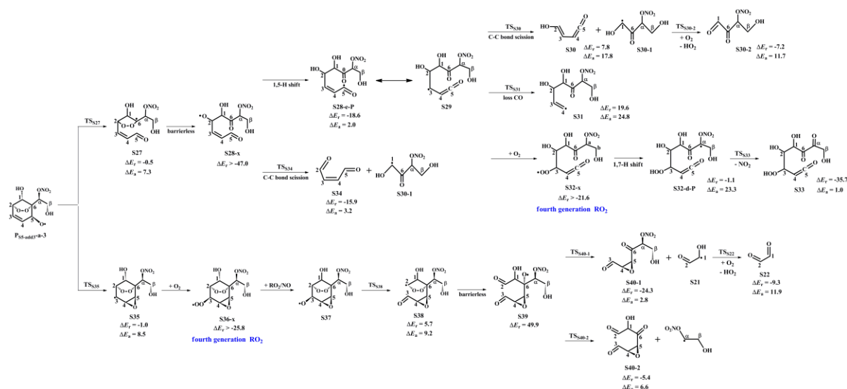
Figure 5. PES for the unimolecular decomposition of P S5-add3-a-3 and its subsequent reactions at the M06-2X/6-311++G(3df,3pd)//M06-2X/6-31+g(d,p) level
