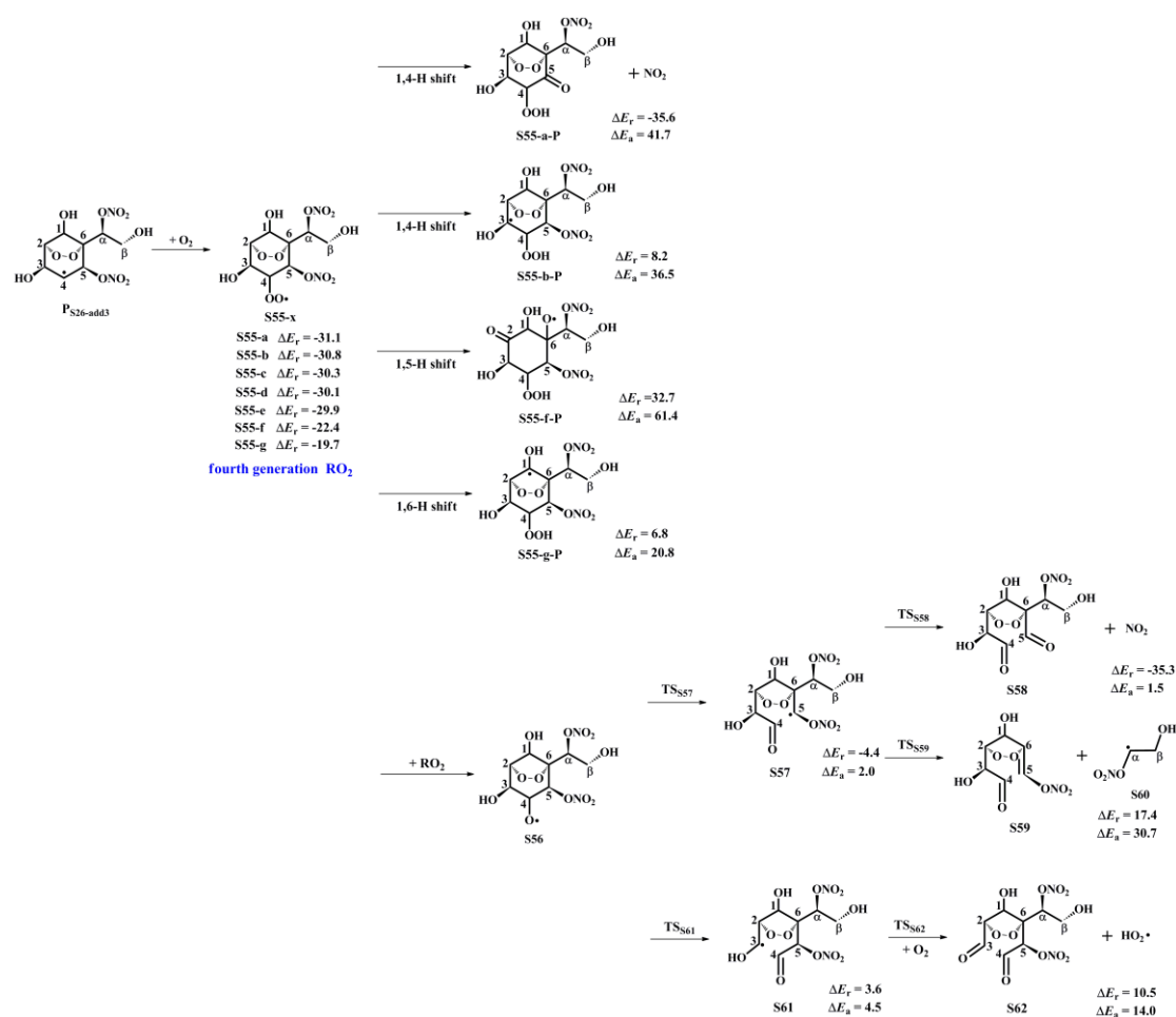
Figure 7. PES for the subsequent reactions of P_{S26-add3} in the presence of O_2 at the M06-2X/6-311++G(3df,3pd)//M06-2X/6-31+g(d,p) level
