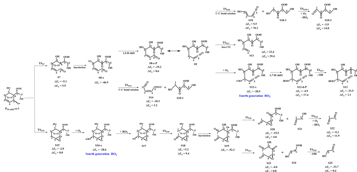
Figure 3. PES for the unimolecular decomposition of P S4-add3-a-3 and its subsequent reactions at the M06-2X/6-311++G(3df,3pd)//M06-2X/6-31+g(d,p) level
