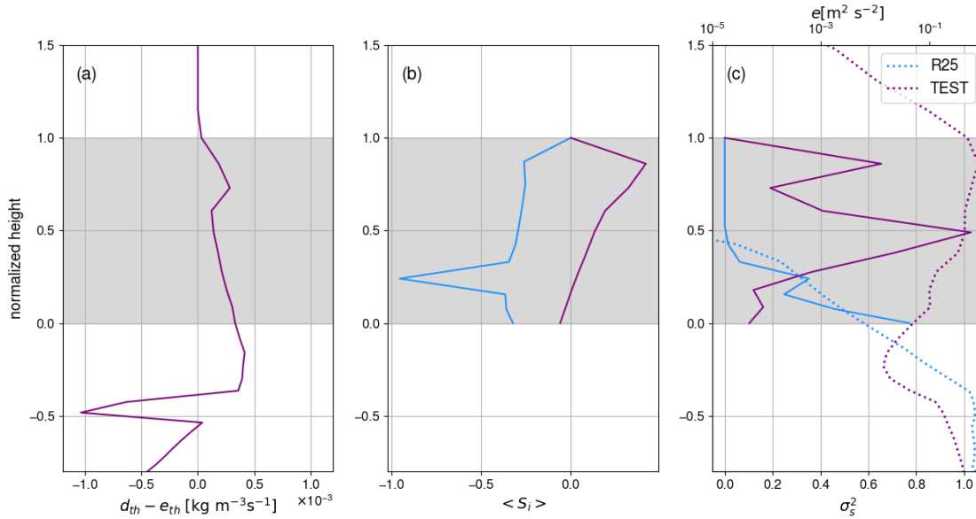
Figure 3. (a): Vertical profile of net detrainment rate in the TEST simulation (solid line, bottom x-axis). (b): Vertical profile of the mean in-cloud supersaturation in the R25 (blue) and TEST (purple) simulation. (c): Vertical profile of the variance of the in-cloud supersaturation (solid lines, bottom x-axis) and of the TKE in the R25 and TEST simulations (dotted lines, top x-axis). In all panels, the vertical axis is the normalized height and grey shading indicates the cloudy area. The profiles shown correspond to the median profiles over the well-developed phase of the clouds, namely between 01:00 and 05:00, 10 October 2024.
