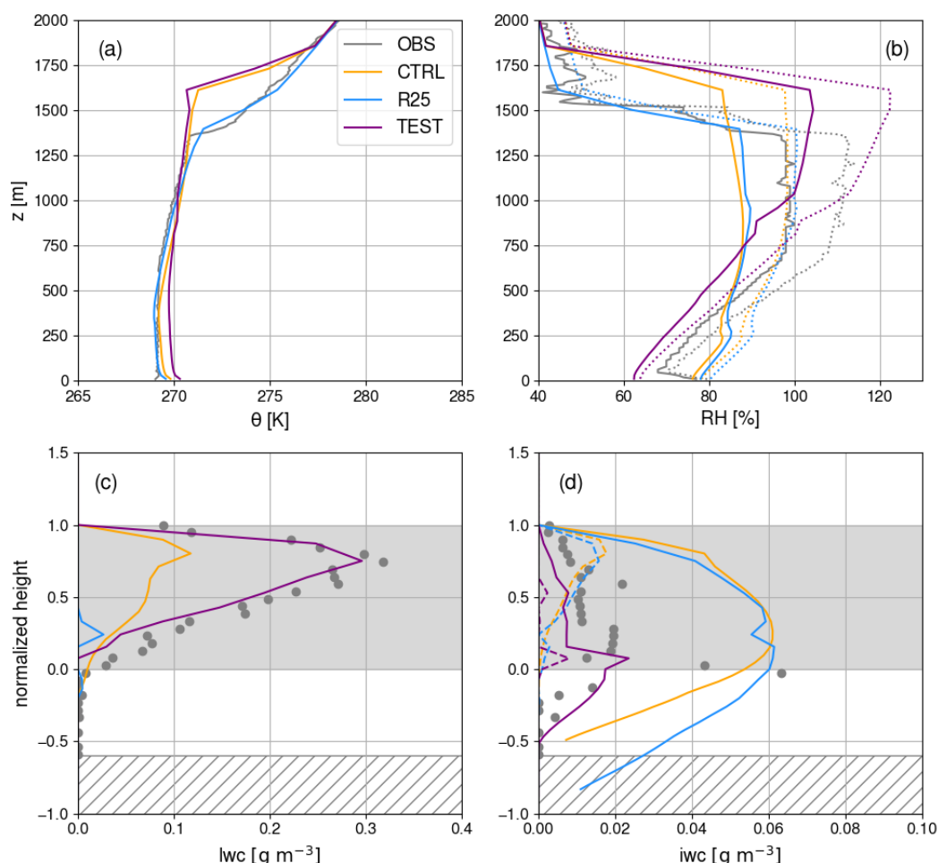
Figure 2. Vertical profiles of potential temperature (a), relative humidity with respect to liquid (panel b, solid lines) and ice (panel b, dotted lines), liquid water content (panel c) and ice water content including (resp. excluding) snow precipitation in solid (resp. dashed) lines (panel d). CTRL, R25 and TEST simulations are shown in orange, blue and purple respectively and simulation profiles are averaged over the well-developed phase of the clouds, namely between 01:00 and 05:00, 10 October 2024. In panel a and b, observations (in grey) correspond to the radiosonde launched at Utqiagvik, Alaska at 17:00 UTC, 9 October. In panels c and d, the vertical axis used is the normalized height – where -1 is the surface, 0 is cloud base, and 1 is cloud top – for consistency with Klein et al. (2009) and grey shading indicates the location of the cloud. Observations (grey dots) correspond to airborne measurements that do not extend below -0.6 in normalized height, hence the hashed area in panel c and d.
