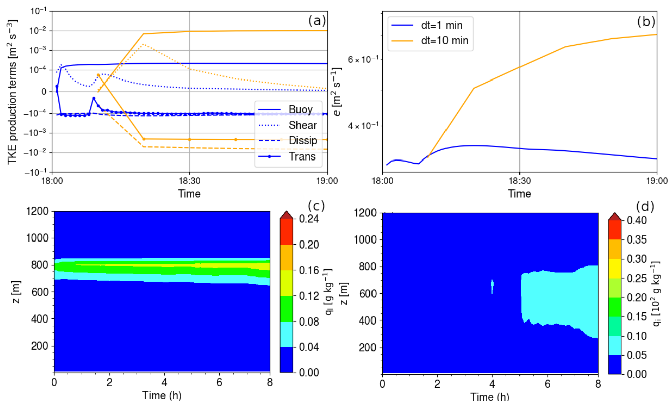
Figure A1. Evolution of the TKE production and loss terms (panel a) and of the TKE (panel b) during the first hour of ISDAC simulations at the model level corresponding to cloud top. Yellow (resp. blue) curves correspond to the simulation with a time step of 10 (resp. 1) min. Panels c and d are the same as panels c and d in Figure 5 but for simulations with a time step of 10 min.
