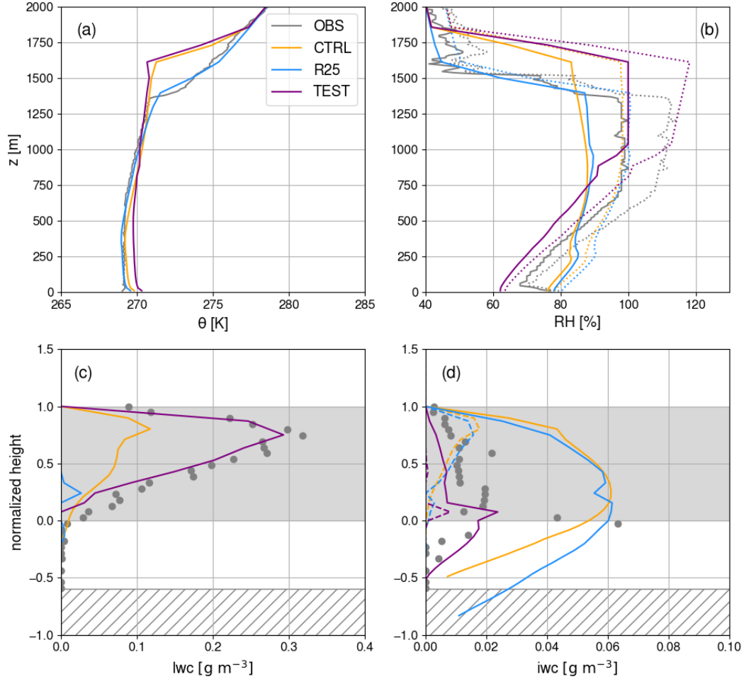
Figure 2. M-PACE vertical profiles of potential temperature (a), relative humidity with respect to liquid (panel b, solid lines) and ice (panel b, dotted lines), liquid water content (panel c) and ice water content including (resp. excluding) snow precipitation in solid (resp. dashed) lines (panel d). CTRL, R25 and TEST simulations are shown in orange, blue and purple respectively and simulation profiles are averaged over the well-developed phase of the clouds, namely between 01:00 and 05:00, 10 October 2024. In panel a and b, observations (in grey) correspond to the radiosonde launched at Utqiagvik, Alaska at 17:00 UTC, 9 October. In panels c and d, the vertical axis used is the normalized height – where -1 is the surface, 0 is cloud base, and 1 is cloud top – for consistency with Klein et al. (2009) and grey shading indicates the location of the cloud. Observations (grey dots) correspond to airborne measurements that do not extend below -0.6 in normalized height, hence the hashed area in panel c and d. Note that in LMDZ, the relative humidity corresponds to a diagnostic variable computed as the ratio of the mean specific humidity in the mesh to the saturation specific humidity at the mean temperature in the mesh, the relative humidity with respect to liquid being capped at 100% as cloud liquid water forms through adjustment process.
