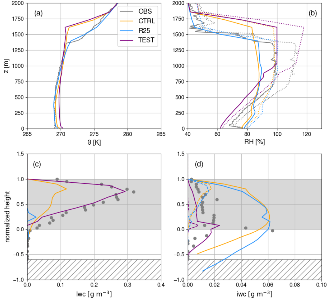
Figure 2. M-PACE vertical profiles of potential temperature (a), relative humidity with respect to liquid (panel b, solid lines) and ice (panel b, dotted lines) , liquid water content (panel c) and ice water content including (resp. excluding) snow precipitation in solid (resp. dashed) lines (panel d). CTRL, R25 and TEST simulations are shown in orange, blue and purple respectively and simulation profiles are averaged over the well-developed phase of the clouds, namely between 01:00 and 05:00, 10 October 2024. In panel a and b, observations (in grey) correspond to the radiosonde launched at Utqiagvik, Alaska at 17:00 UTC, 9 October. In panels c and d, the vertical axis used is the normalized height – where 1 is the surface, 0 is cloud base, and 1 is cloud top – for consistency with Klein et al. (2009) and grey shading indicates the location of the cloud. Observations (grey dots) correspond to airborne measurements that do not extend below -0.6 in normalized height, hence the hashed area in panel c and d. Note also that in LMDZ profiles of, the relative humidity correspond corresponds to a diagnostic variable computed as the ratio of the mean specific humidity in the mesh to the saturation specific humidity at the mean temperature in the mesh, the relative humidity with respect to liquid being capped at 100% as cloud liquid water forms through adjustment process.
