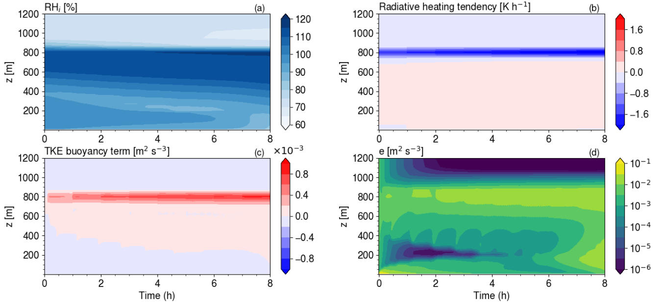
Figure 6. Time height plots of the relative humidity with respect to ice (a), radiative heating tendency (b), TKE production term by buoyancy (c) and TKE (d) in the TEST LMDZ SCM simulation on the ISDAC case.
