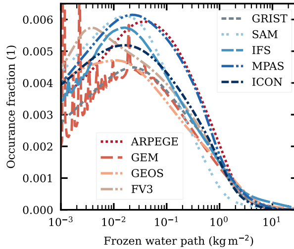
Figure 11. Logarithmically binned occurrence fractions (log-OF) of each model's FWP between 60^\circ \text{ S} and 60^\circ \text{ N} (Feb 2020). The spikes for some models are caused by discretization of the output.
