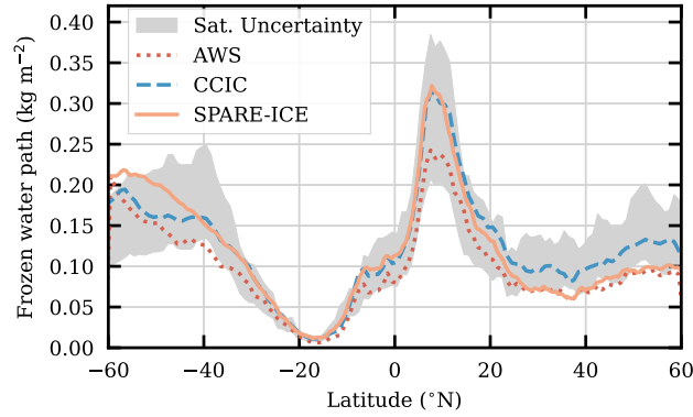
Figure 5. Zonal mean, for July and August 2025, of three retrievals based on passive observations. The CCIC data have been sub-sampled to the local solar times observed by AWS (approx. 10:30 and 22:30). The grey area represents the expected range according to CloudSat-based estimates covering 2007-2010 (see Sec. 3.6 for details)
