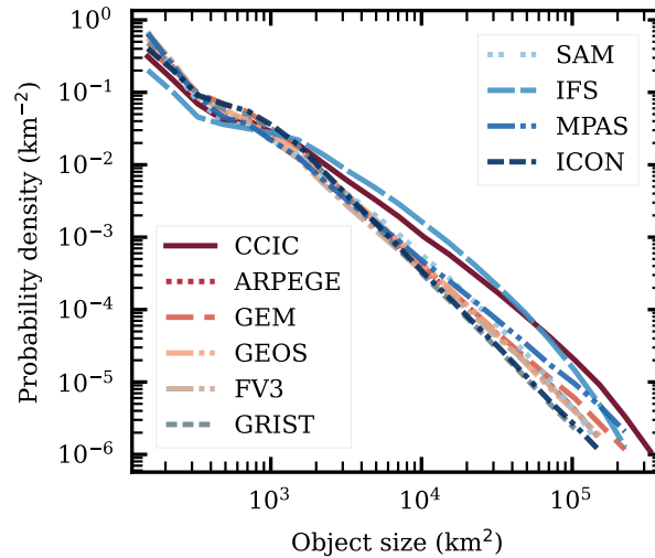
Figure 14. The probability distribution of convective core object areas. Considered area and definition of objects as in Fig. 13.
