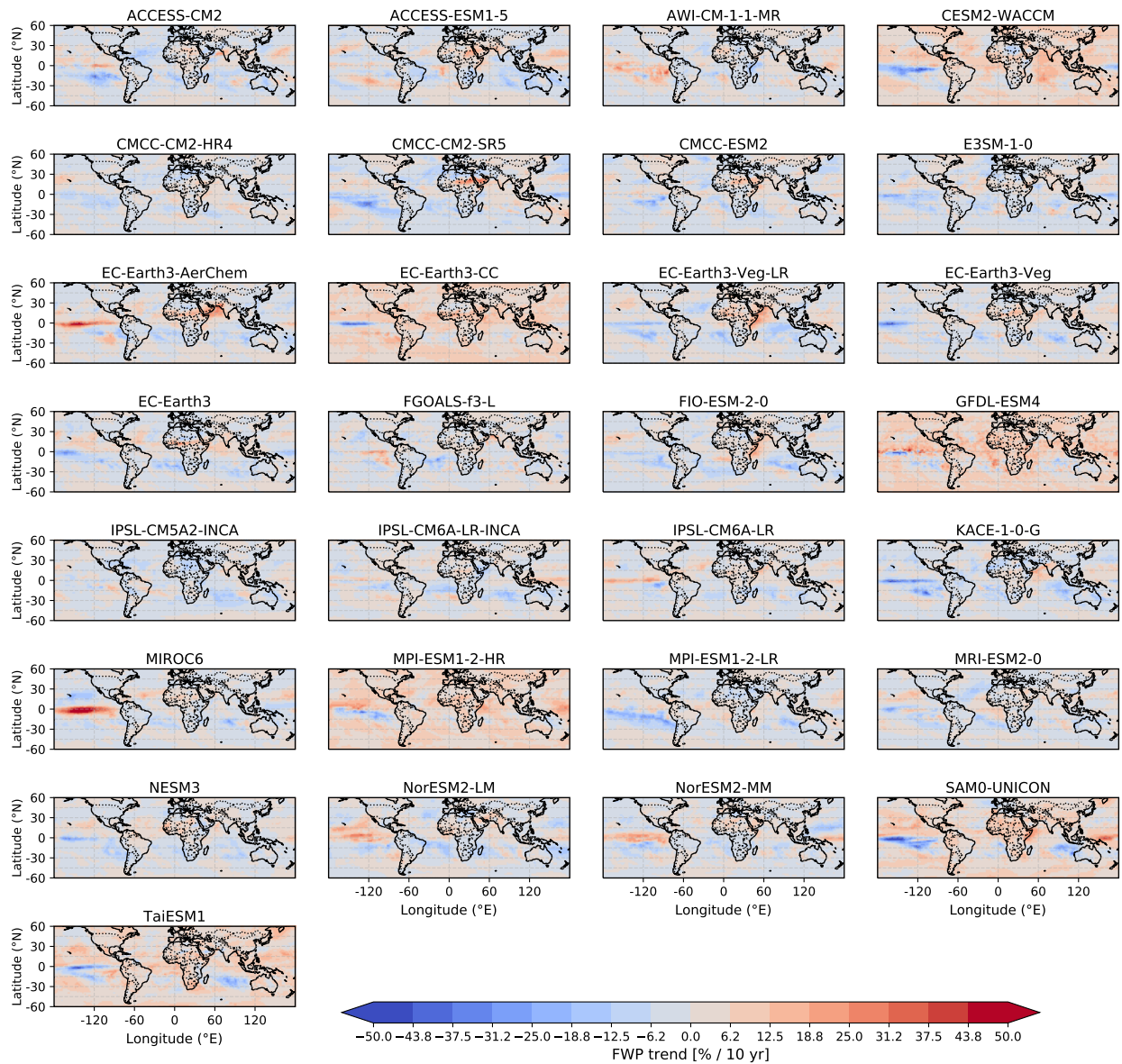
Figure B2. Decadal FWP trends from 1980 to 2014 for the CMIP6 historical simulations. The trends based on the monthly mean values in each model grid cell for the full period. Red-shaded regions correspond to increases in FWP, whereas blue-shaded regions correspond to decreases in FWP.
