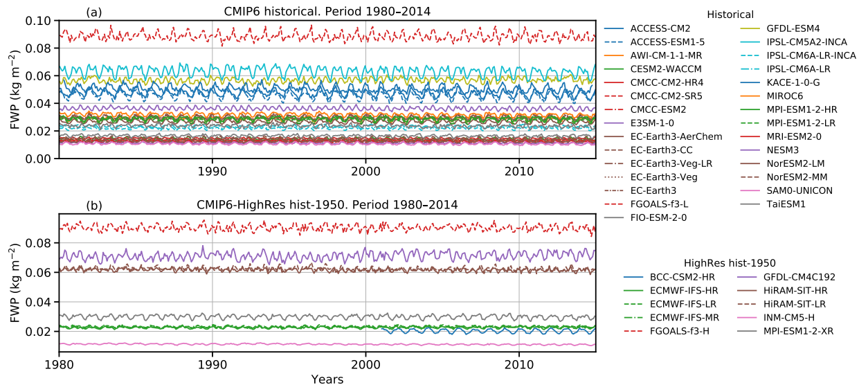
Figure B1. Time series of monthly means FWP between 60°S and 60°N during the period 1980-2014 for (a) CMIP6 historical simulations, and (b) CMIP6 HighRes hist-1950 simulations.
