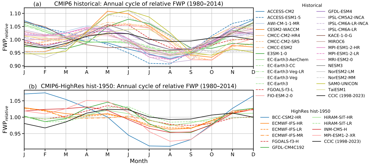
Figure 8. Annual cycles of relative FWPs ( FWP_{relative} ) between 60^{\circ}\text{S} and 60^{\circ}\text{N} , calculated for each model as the ratio of monthly mean FWP to the mean FWP over 1980–2014. Results are shown for (a) CMIP6 historical simulations and (b) CMIP6 HighRes hist-1950 simulations. The annual cycle of FWP_{relative} for CCIC over 1998–2023 is also shown in both panels for comparison.
