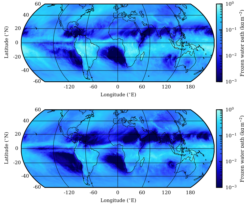
Figure 9. Gridded ( 1^\circ resolution) mean FWP for February 2020, for CCIC (top panel) and averaged over the nine considered GSRMs (lower panel).
