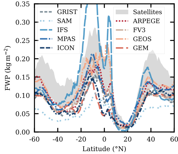
Figure 10. Zonal mean FWP of the GSRM models (Feb 2020). The grey area represents the expected range according to CloudSat-based estimates covering 2007-10 (Sec. 3.6). The primary peak of the IFS-model is cut off in an attempt to improve visual clarity for all other models. It has a maximum FWP value of 0.46 \text{ kg m}^{-2} at 9.5^\circ \text{ S} .
