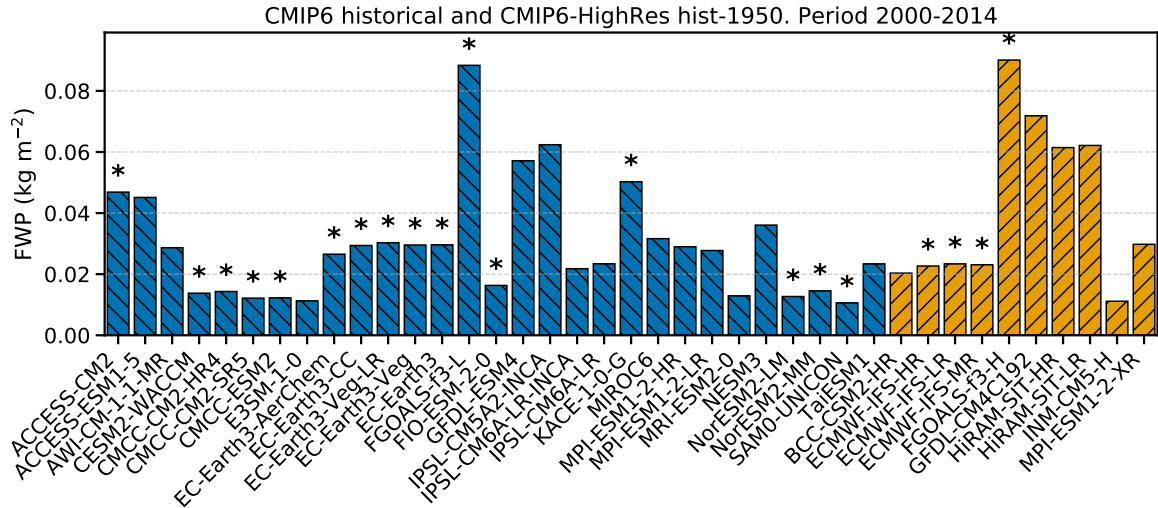
Figure 6. Average of monthly FWP means, between latitudes 60°S and 60°N, during the period 2000-2014 for the CMIP6 historical simulations (bars in blue with stripes descending), and CMIP6 HighRes hist-1950 simulations (bars in orange with stripes ascending). Models including falling ice in their FWP are marked with an asterisk (*).
