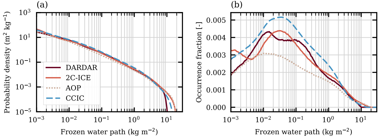
Figure 3. Distributions of retrieved FWP values from daytime observations during 2015 and for latitudes between \pm 60^\circ\text{N} . The sampling of the CCIC dataset is centred around CloudSat LTAN with an interval of \pm 15 minutes. All cases (including FWP = 0) are used in the normalisation. Panel (a) shows the overall probability distribution function. Panel (b) shows the logarithmically binned occurrence fractions (using 200 bins between 10^{-4} and 10^2 \text{kg m}^{-2} ).
