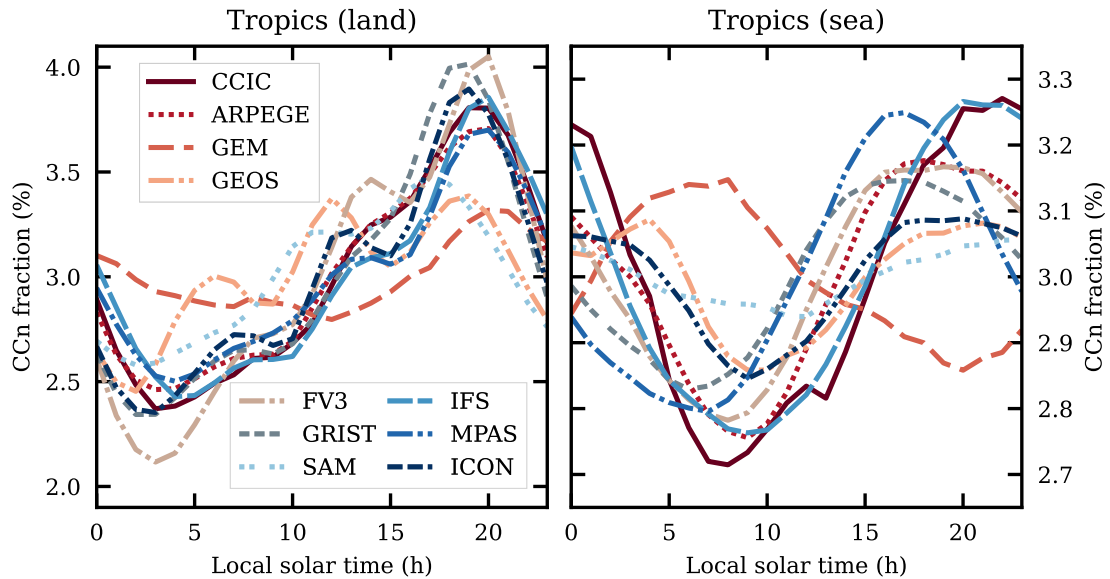
Figure 15. The diurnal variation of data exceeding the CC_n threshold, of the GSRM models and CCIC (Feb 2020), over land (left) and sea (right). The diurnal average of all datasets is 3 %, as stipulated by the definition of CC_n .
