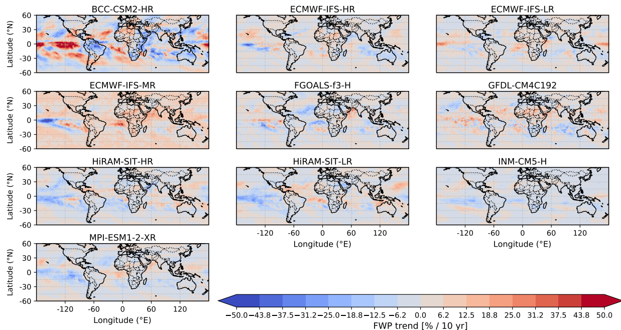
Figure B3. Decadal FWP trends from 1980 to 2014 for the CMIP6 HighRes hist-1950 simulations. Red-shaded regions correspond to increases in FWP, whereas blue-shaded regions correspond to decreases in FWP.
