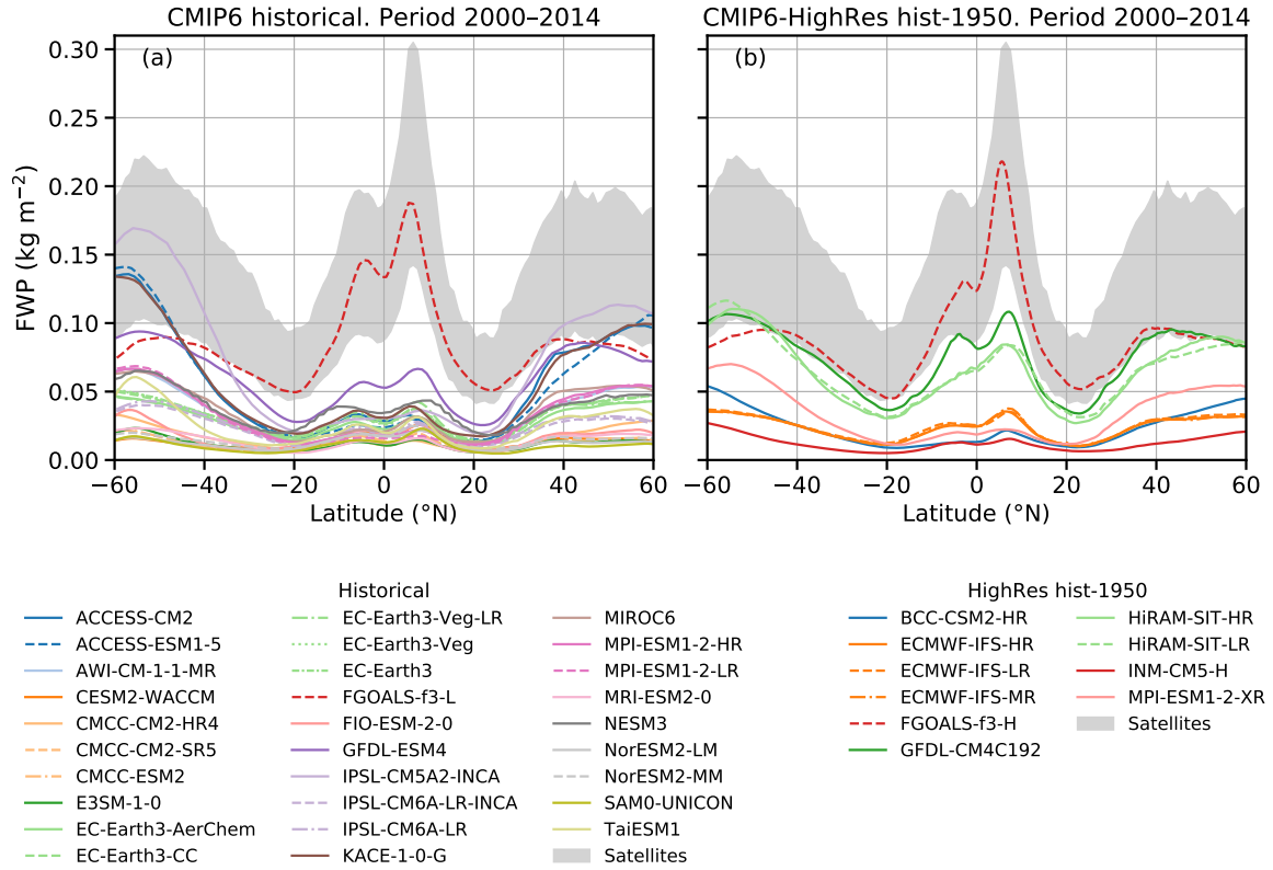
Figure 7. Zonal means of monthly FWP means during the period 2000-2014 for (a) CMIP6 historical simulations, and (b) CMIP6 HighRes hist-1950 simulations. The grey area represents the expected range according to CloudSat-based estimates covering 2007-10 (Sec. 3.6).
