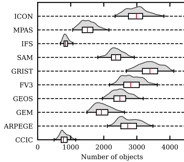
Figure 13. Distribution of number of convective core objects, inside 20^{\circ} S to 20^{\circ} N for each GSRM model and CCIC (Feb 2020). The grey areas are the probability distributions of object numbers, between model and retrieval time steps. A corresponding box-plot (representing the 0th and 100th percentile as whiskers, the 25th, 50 and 75th percentile as a box and the median as a red line) is shown underneath. Objects are defined as the set of adjacent grid cells (including diagonals) whose FWP value is in the top 3 % for the dataset of concern.
