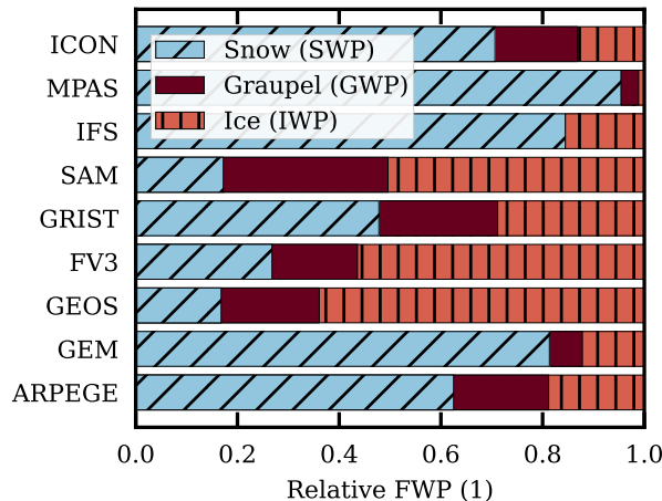
Figure 12. Relative fraction of ice, snow and graupel to the total frozen water, for each GSRM model. Compiled using all data between 60° S and 60° N (Feb 2020). For IFS, snow incorporates the graupel category.
