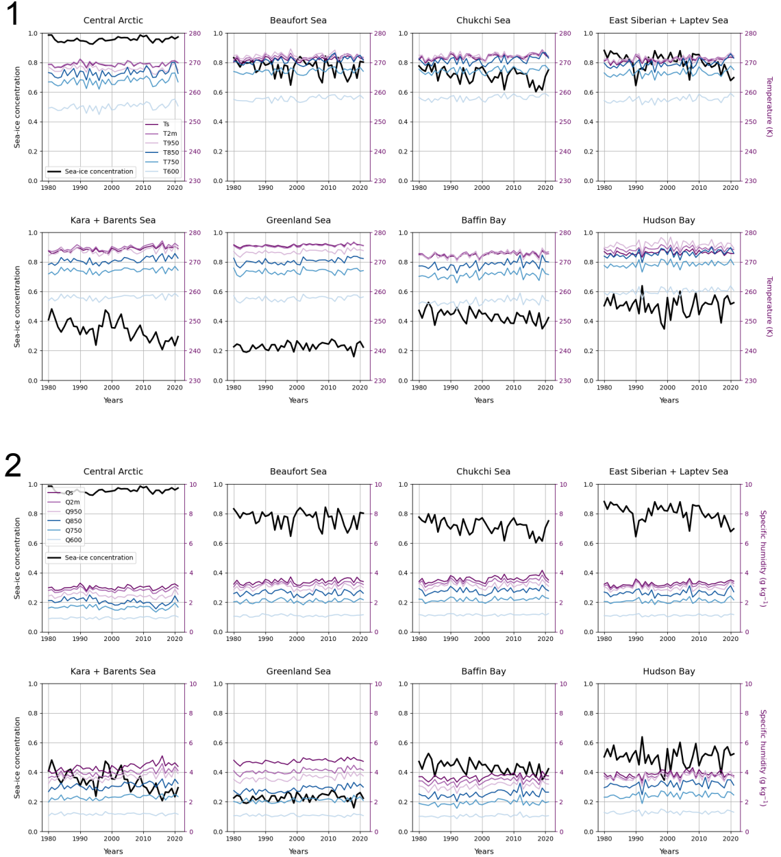
Figure S2. Seasonal means calculated from daily means in May–June–July during years 1980–2021 averaged over the areas of eight Arctic basins (as shown in Fig. 1). Part 1: Sea-ice concentration and temperature at the surface and the levels of 2 m, 950 hPa, 850 hPa, 750 hPa, and 600 hPa ( T_s , T_{2m} , T_{950} , T_{850} , T_{750} , T_{600} ). Part 2: Same as Part 1 but for the surface and air specific humidities. Only grid cells fully covered by the sea were considered in this analysis.
