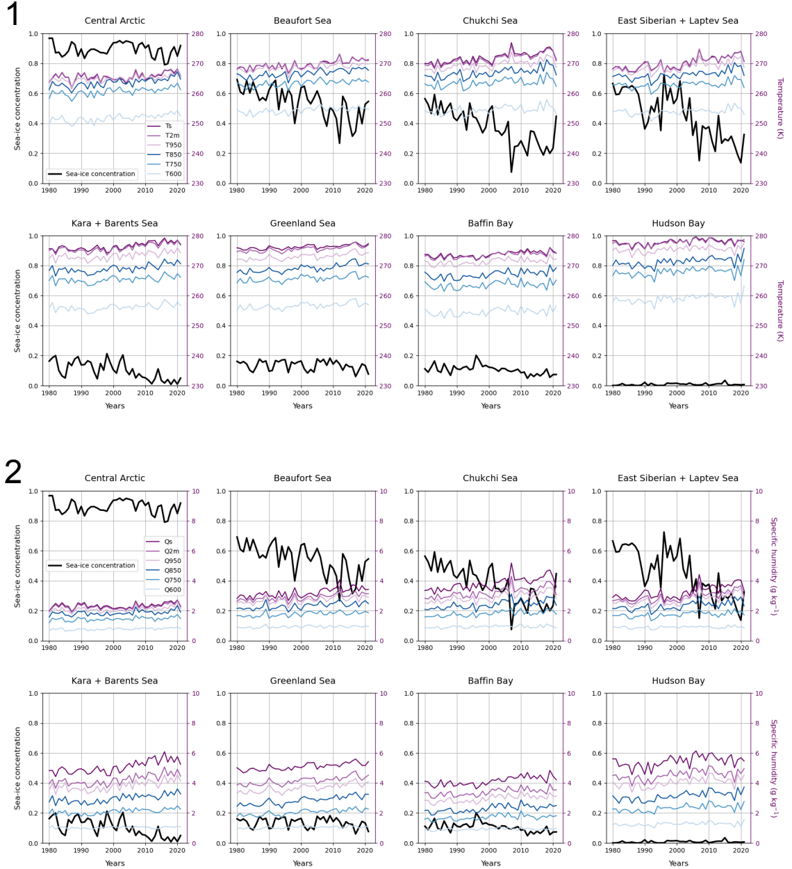
Figure S3. Seasonal means calculated from daily means in August–September–October during years 1980–2021 averaged over the areas of eight Arctic basins (as shown in Fig. 1). Part 1: Sea-ice concentration and temperature at the surface and the levels of 2 m, 950 hPa, 850 hPa, 750 hPa, and 600 hPa ( T_s , T_{2m} , T_{950} , T_{850} , T_{750} , T_{600} ). Part 2: Same as Part 1 but for the surface and air specific humidities. Only grid cells fully covered by the sea were considered in this analysis.
