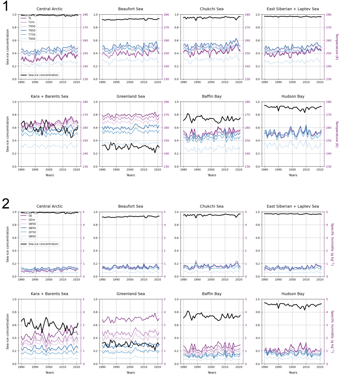
Figure S1. Seasonal means calculated from daily means in February–March–April during years 1980–2021 averaged over the areas of eight Arctic basins (as shown in Fig. 1). Part 1: Sea-ice concentration and temperature at the surface and the levels of 2 m, 950 hPa, 850 hPa, 750 hPa, and 600 hPa ( T_s , T_{2m} , T_{950} , T_{850} , T_{750} , T_{600} ). Part 2: Same as Part 1 but for the surface and air specific humidities. Only grid cells fully covered by the sea were considered in this analysis.
