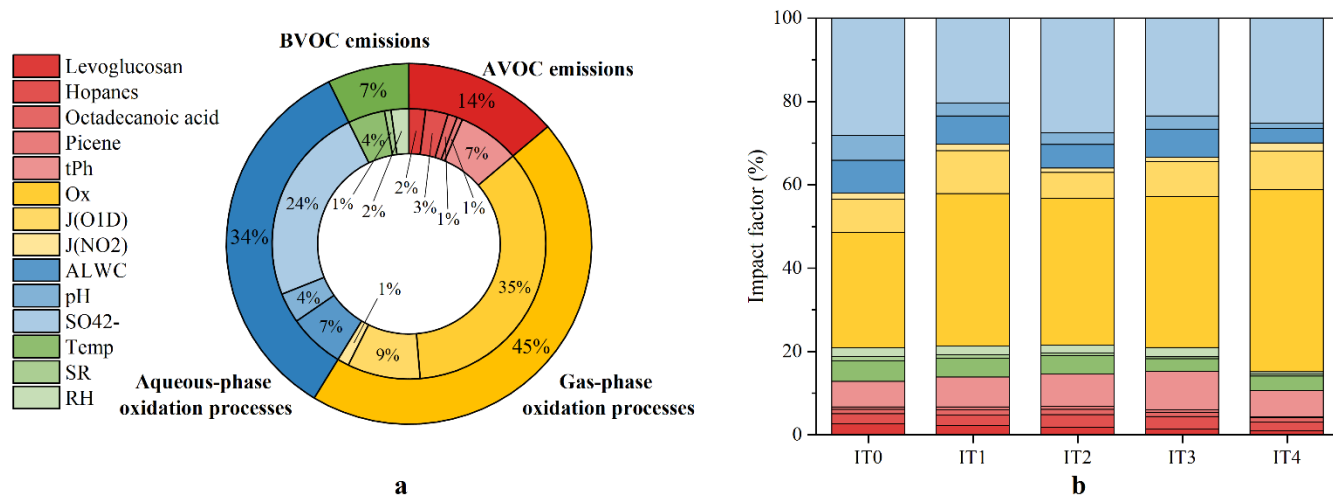
Figure 6. (a) Impact of changes of each variable on C_2 variation during the whole study period. (b) Impact factor of individual variable under different pollution conditions.
