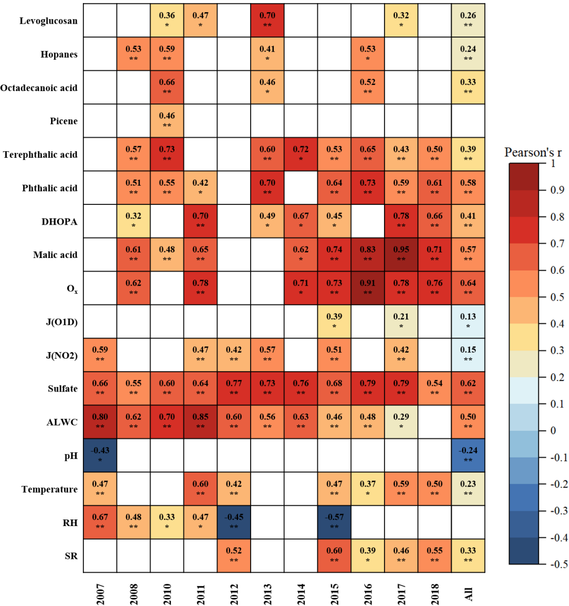
Figure 3. Correlations between C 2 and primary anthropogenic source markers, SOA markers, indicators for gas- and aqueous-phase oxidation , as well as meteorological parameters. Blank cells indicate no significant correlations. One asterisk, two asterisks denote p value < 0.05, 0.01, respectively. Due to the unavailability of O x data in 2012 and 2013, correlation analysis was not conducted for these two years.
