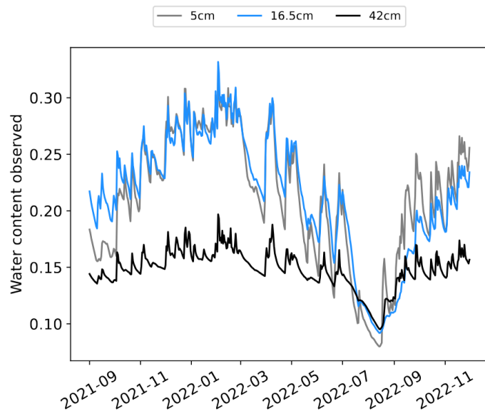
Figure S2: Soil water content measured with TDR sensors beneath a spruce plot of the Strengbach catchment at three different depths (5, 16.5 and 42cm). Monitoring devices included Campbell TDR probes (model CS616, Campbell Scientific Inc., Logan, UT, USA) and Campbell temperature probes (model 107, Campbell Scientific Inc., Logan, UT, USA) to allow for temperature correction, connected to a Campbell CR1000 data logger with a 10-min recording interval. The standard quadratic calibration equation provided by the manufacturer was used to derive volumetric water content ( \text{m}^3/\text{m}^3 ). An important decrease in soil water content was observed in July and August 2022 across the entire soil profile. An earlier decrease was also observed in May and June at depths of 5 and 16.5cm. Those two drying periods are consistent with the simulation outputs presented in Section 3.1. Notice that these measurements were conducted on a different plot from the one where soil solutions were sampled.
