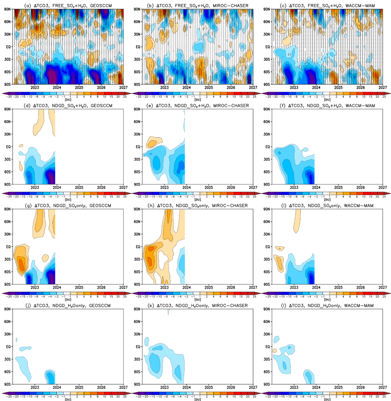
Figure 2. Latitude vs time changes (perturbed minus control) in total column ozone (TCO3) simulated in GEOSCCM (left; a,d,g,j), MIROC-CHASER (middle; b,e,h,k) and WACCM-MAM (right; c,f,i,l). Row 1 is for the free-running experiment with simultaneous injection of SO 2 and H 2 O (stippling defined as in Fig. 1). Rows 2-4 are for the nudged simulations (2022-2023), with SO 2 +H 2 O injection (row 2), SO 2 -only injection (row 3) or H 2 O-only injection (row 4).
