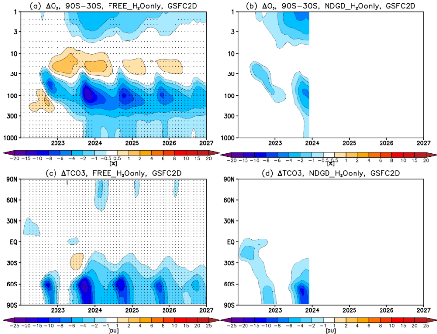
Figure 10. Row 1 (a-b): Pressure vs time changes (perturbed minus control) in 90°S–30°S average ozone mixing ratios simulated in GSFC2D with H 2 O-only injection in the free-running experiment (FREE_H 2 Oonly; left) and in the nudged experiment (NDGD_H 2 Oonly; right). Row 2 (c-d): the corresponding latitude vs time changes in total column ozone. Stippling in left column marks regions where the response is not statistically significant (defined as in Fig. 1).
