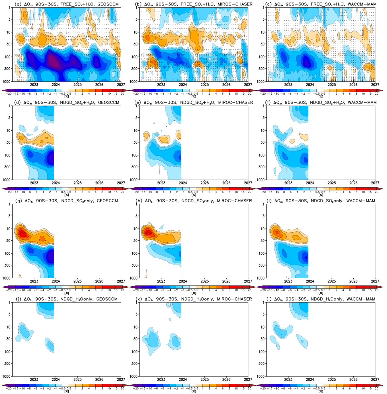
Figure 3. Pressure vs time changes in the SH extra-tropical (90°S–30°S) ozone mixing ratios simulated in GEOSCCM (left; a,d,g,j), MIROC-CHASER (middle; b,e,h,k) and WACCM-MAM (right; c,f,i,l). Row 1 is for the free-running experiment with simultaneous injection of SO 2 and H 2 O (stippling defined as in Fig. 1). Rows 2–4 are for the nudged simulations (2022–2023), with SO 2 +H 2 O injection (row 2), SO 2 -only injection (row 3) or H 2 O-only injection (row 4).
