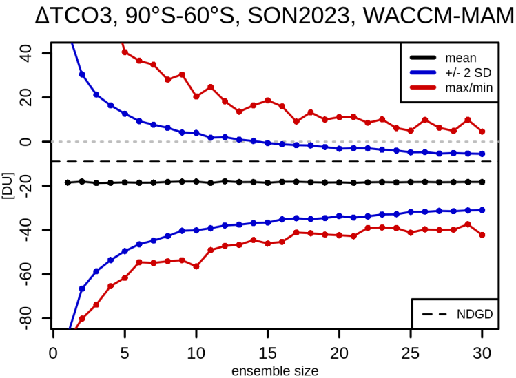
340 Figure 8. Detectability of the September-October-November (SON) 2023 Antarctic total column ozone (TCO3) response in the free-running simulation with the simultaneous injection of SO 2 and H 2 O in WACCM-MAM. Results obtained by randomly subsampling each ensemble with replacement to obtain 2000 artificial ensembles each of different ensemble size. Black lines denote the mean response, and blue and red lines indicate the \pm 2 standard deviation and the maximum/minimum ranges, respectively, of the possible responses. The dashed black line denotes the response obtained from the corresponding nudged simulation. 345
