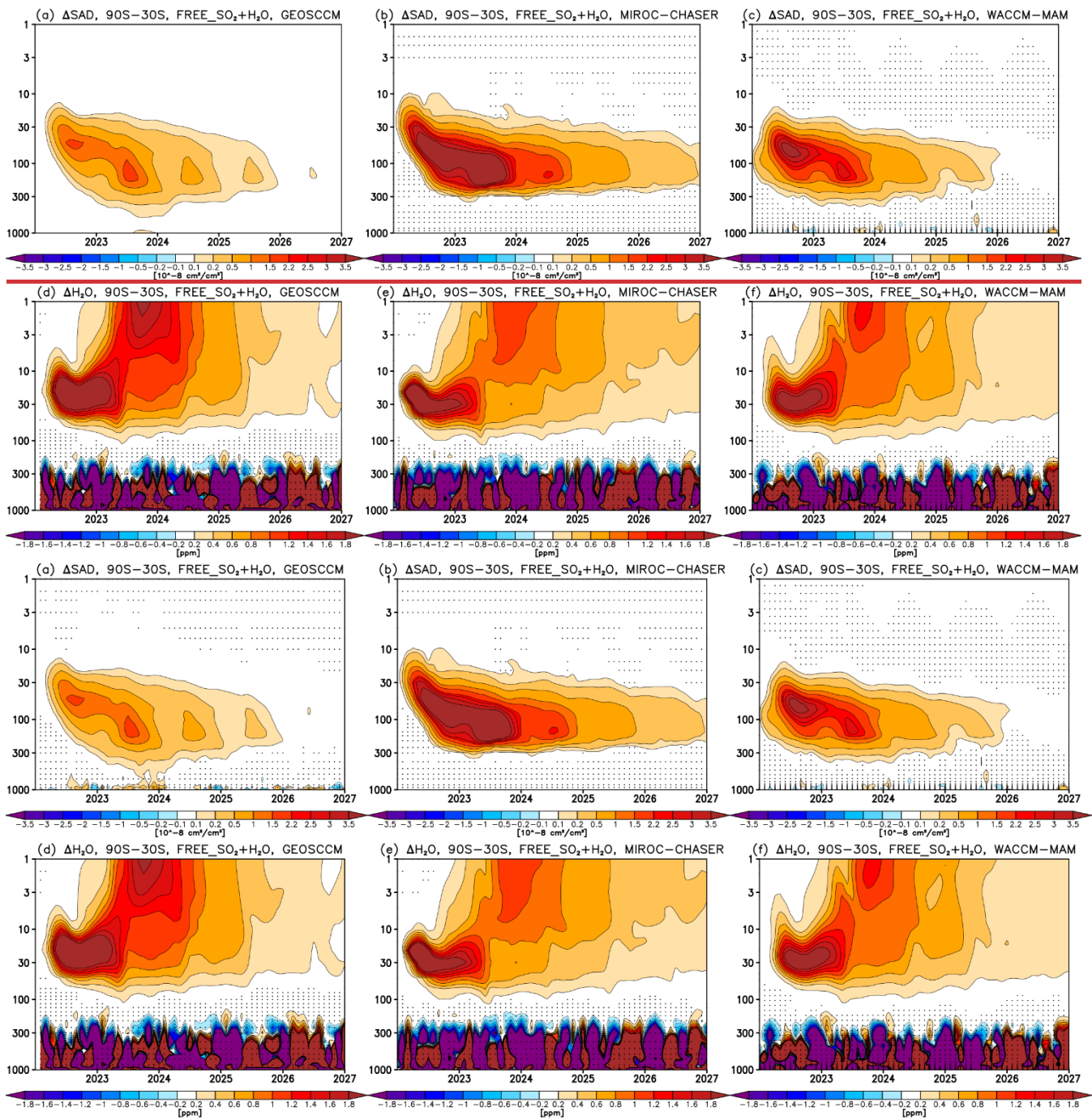
155 Figure 1. Pressure vs time changes (perturbed minus control) in the SH extra-tropical (90°S-30°S) aerosol SAD (row 1; a-c) and 160 water vapor (row 2; d-f) simulated in the free-running experiment with simultaneous injection of SO 2 and H 2 O (FREE_SO 2 +H 2 O) in GEOSCCM (left; a,d), MIROC-CHASER (middle; b,e) and WACCM-MAM (right; c,f). Stippling marks regions where the response is not statistically significant (with the response taken to be significant if it exceeds ±2 standard errors in the difference in means). The aerosol SAD diagnostics used for GEOSCCM and MIROC included only sulfate while for WACCM-MAM this also included contribution from other aerosols (mostly in the troposphere); however, this will not affect the derived (perturbed minus
