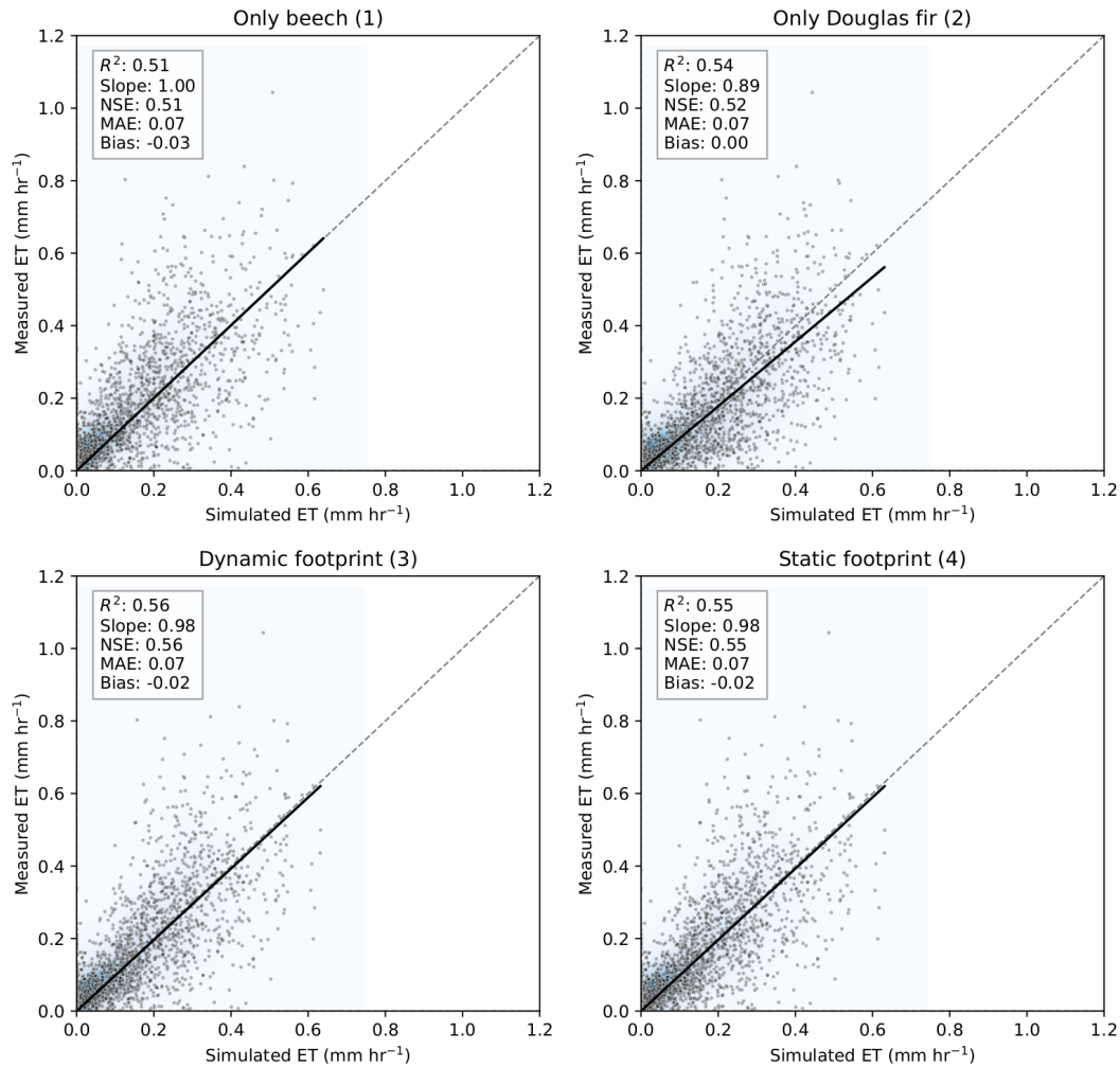
375 Figure 7: Comparison between hourly measured and simulated evapotranspiration (ET, mm hr -1 ) at the ECOSENSE forest for different model configurations: pure beech simulations (1) and pure Douglas fir simulations (2), dynamically weighted simulations according to the hourly footprint (3), and the static footprint (4) with fixed species proportions (66.5% beech and 33.5% Douglas fir). The shaded heatmap represents the kernel density estimate of point concentrations.
