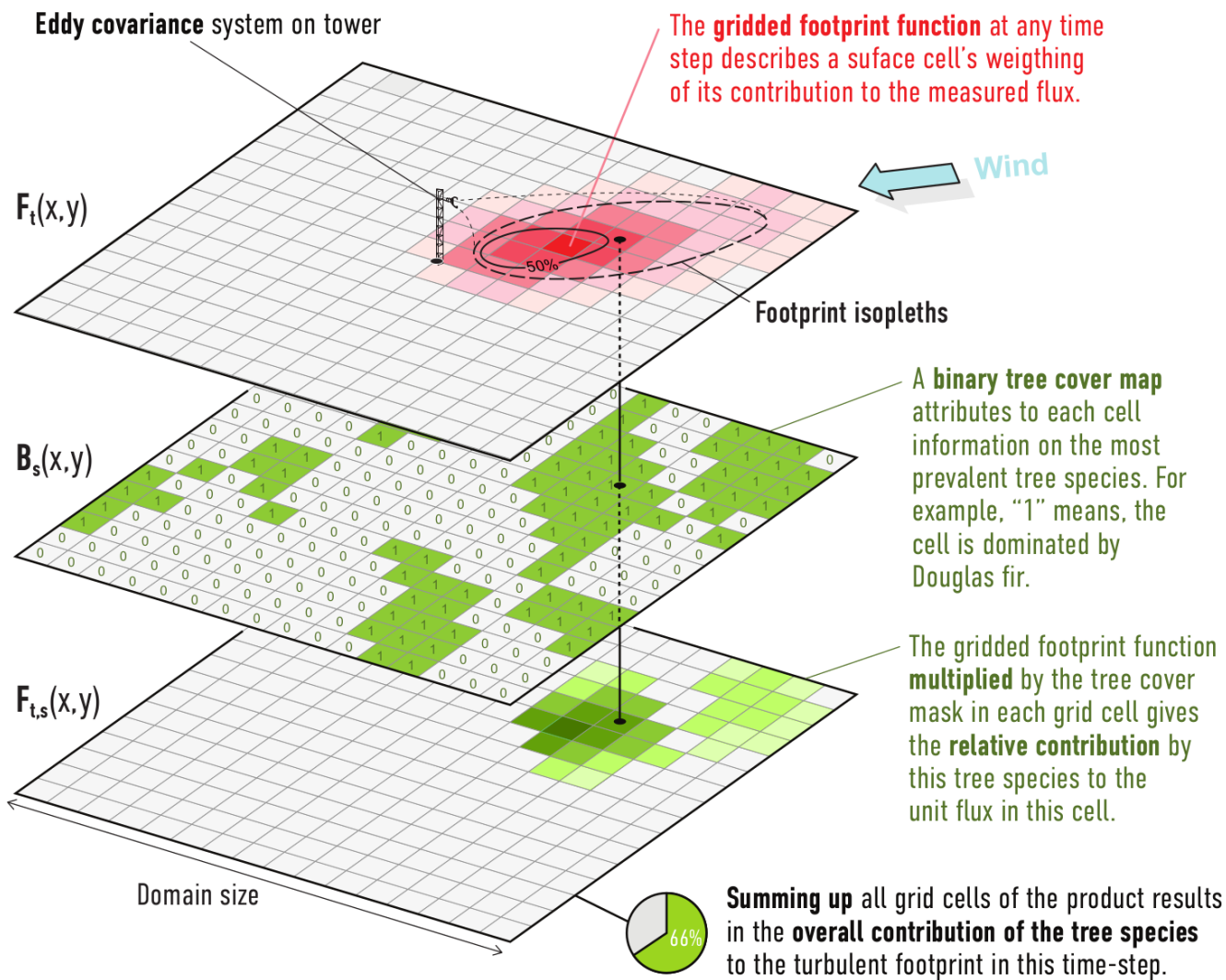
Figure 3: Workflow for estimating tree species contributions to EC flux measurements using raster-based spatial analysis. For each species, a binary presence raster (middle) was generated (1 = species present, 0 = absent). Each binary raster was then multiplied by the corresponding hourly footprint function (top) to retain only the contribution from the target species. The total contribution of each species at each time step was obtained by summing the values of the resulting raster. This process was repeated for each species and each hourly footprint in the analysis period.
