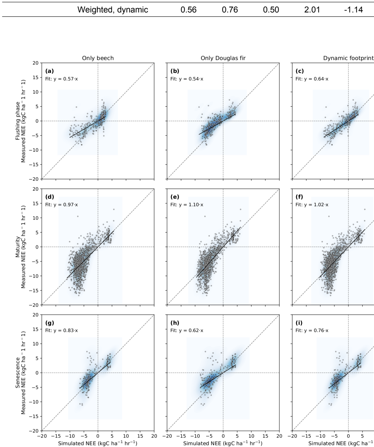
Figure 9: Seasonal differentiation of hourly measured vs. simulated net ecosystem exchange (NEE, \text{kgC ha}^{-1} \text{hr}^{-1} ) at the ECOSENSE forest considering the configurations: pure beech (first column, panels a, d, and g) pure Douglas fir (second column, panels b, e, and h), and the result for dynamically weighting the forest types according to the specific hourly footprint (third col-
