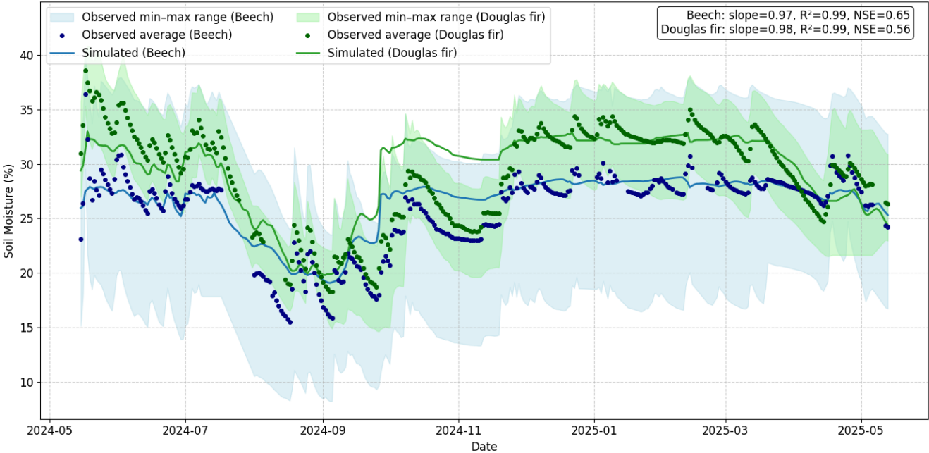
325 Figure 4: Comparison of simulated and measured soil moisture at 30 cm depth for beech and Douglas fir plots from 15 May 2024 to 15 May 2025 at the ECOSENSE forest. The shaded area represents the observed range (min–max across five sensors in each plot), the dots show the average of the measured flux, while the solid line shows the model simulation.
