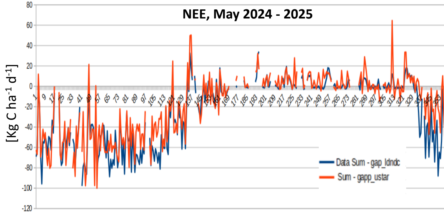
Fig. S...: simulated (blue) and measured (red) daily net ecosystem exchange (NEE) of carbon dioxide ( graphics and letter size will be improved ).
